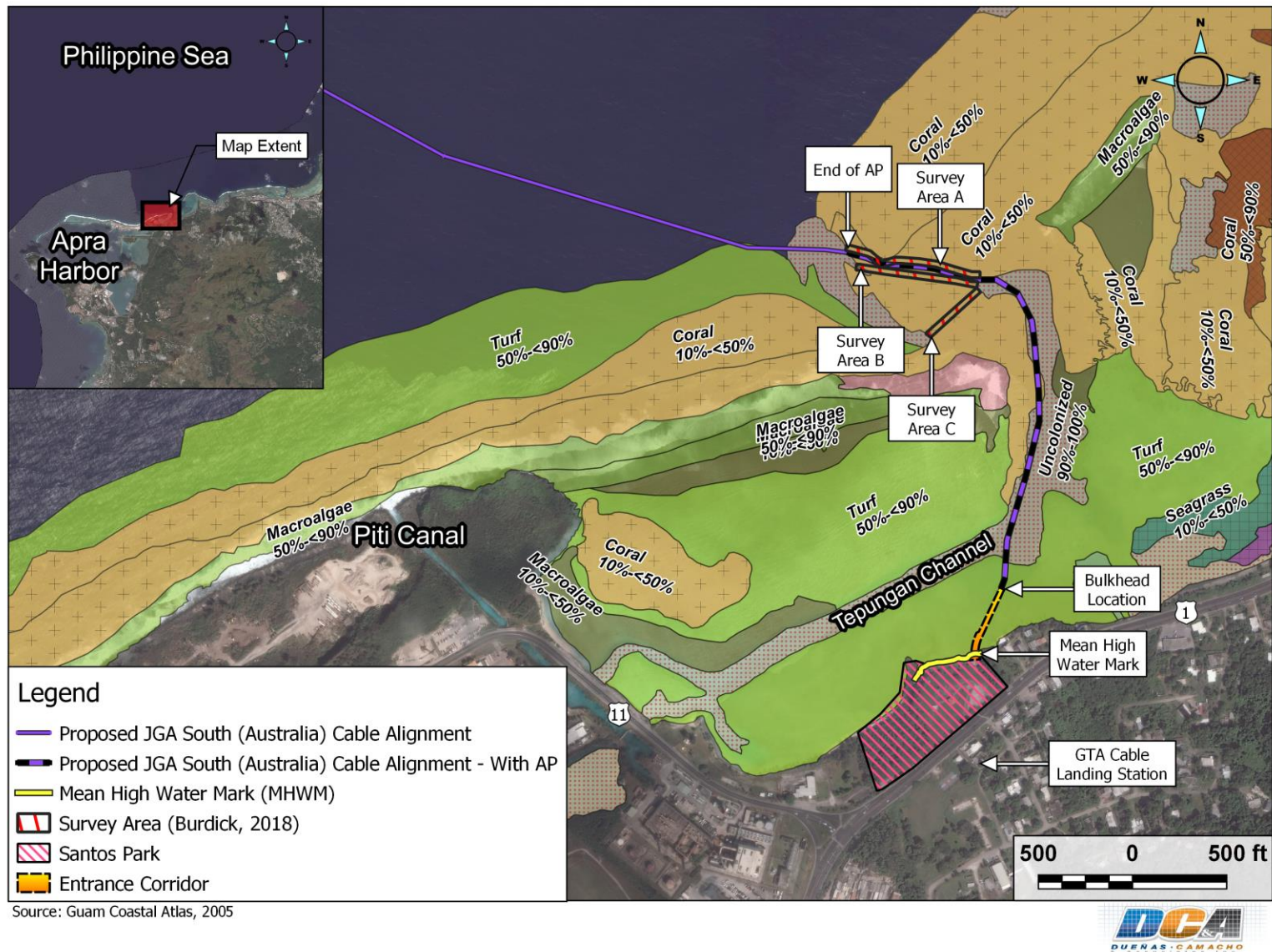
Figure 4. Benthic Habitat map of the JGA South Cable in Piti, Guam.
