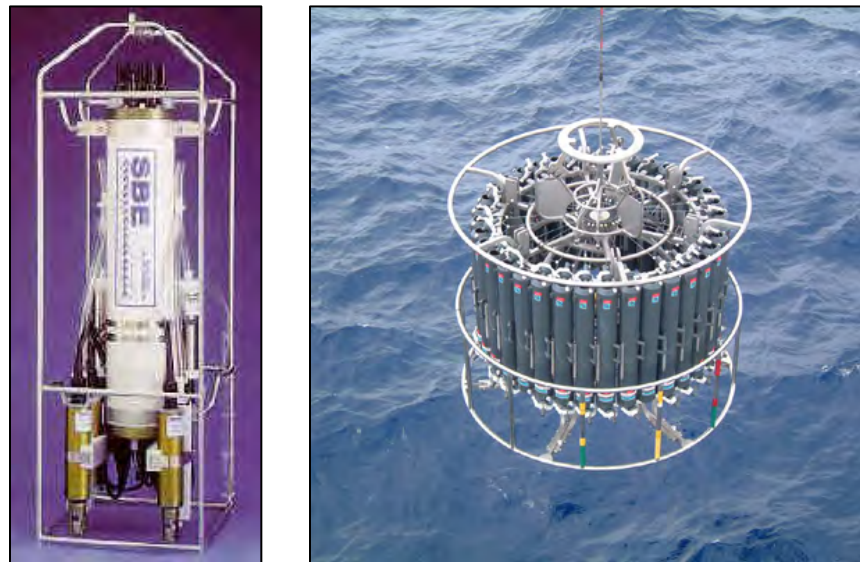
Figure A-34 Sea-Bird 911 plus CTD profiler and deployment on a sampling rosette.
