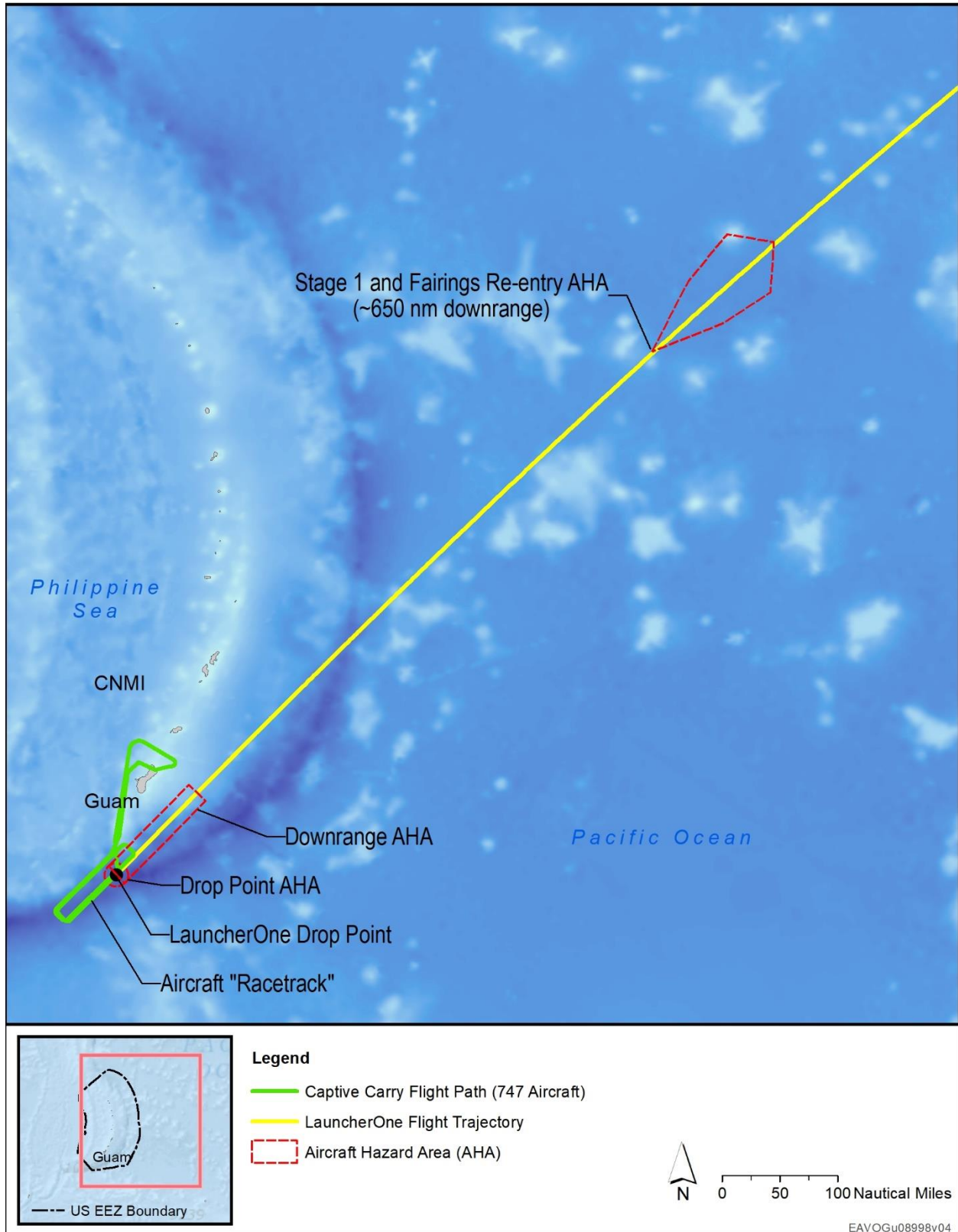
Figure 2.1-7. LauncherOne Flight Trajectory Including Drop Point, Downrange AHA, and Stage 1 and Fairings Re-entry AHA
