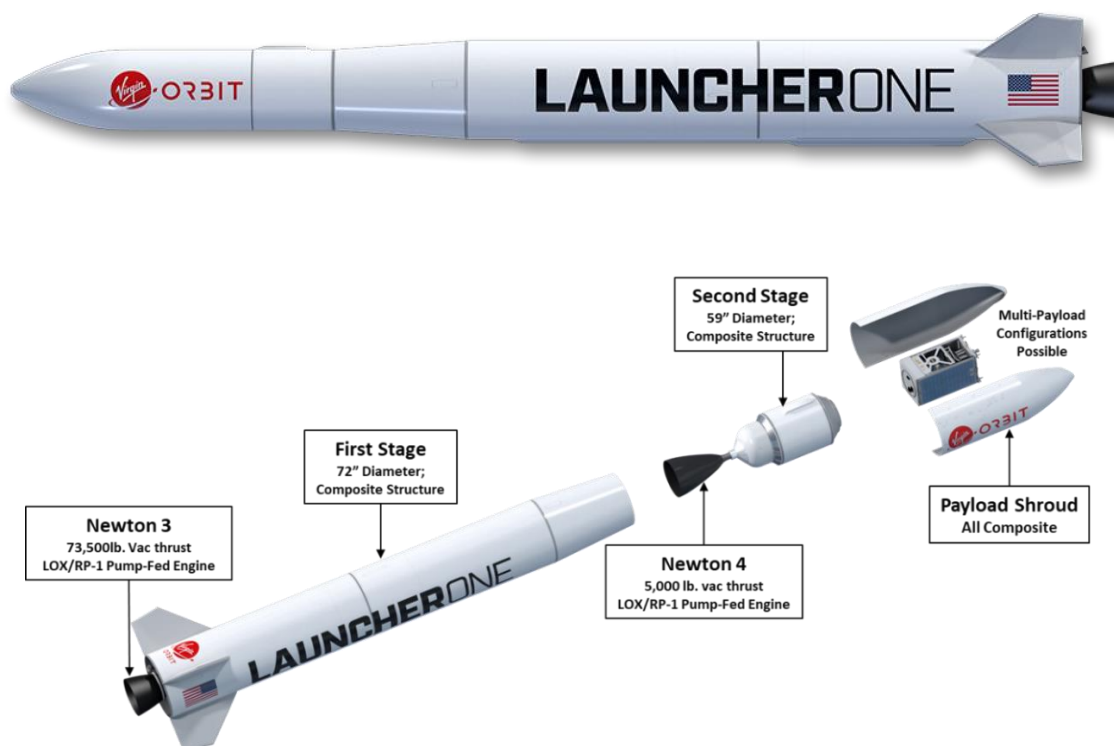
Figure 2.1-4. LauncherOne Rocket
