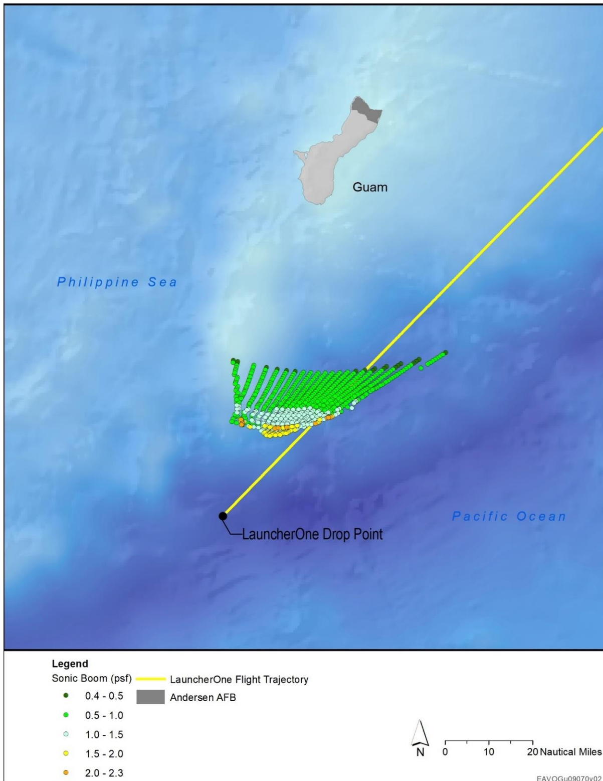
Figure 3.5-2. Modeled Potential Sonic Boom from LauncherOne Vehicle
