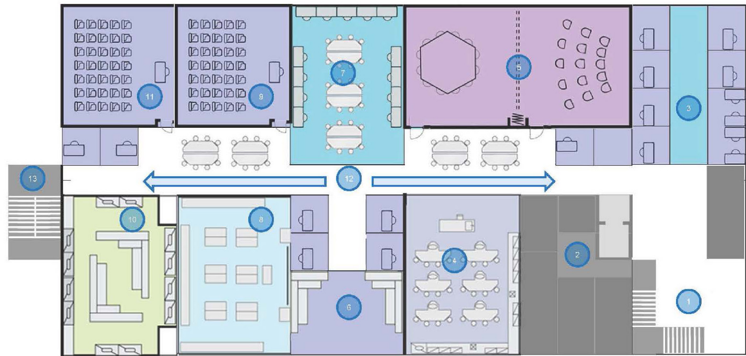
A prototypical classroom building developed using the 1,200SF module. This example shows ten modules of programmable space (for classrooms/offices/labs) per floor. The programmable space does not include utility / circulation space.
