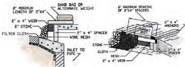
Figure 5.3. Fabric and rock curb inlet protection.
