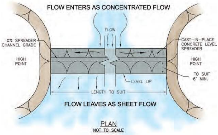
Figure 5.6. Concrete and earth lipped level spreaders (Adapted from: RI Stormwater Manual and NC State University).
