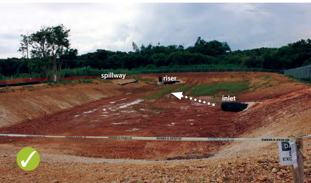
Large sediment basin with inlet pipe, outlet riser, and emergency spillway.
