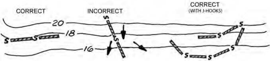
Figure 2.4. Reasons Silt Fences Fail (Adapted from: Center for Watershed Protection)
