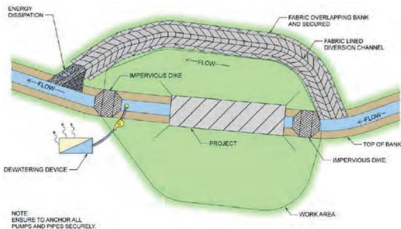
Figure 3.13. Photos of pipe and lined-channel diversions (Sources: Fisheries and Oceans Canada and C.S. Britton) and a schematic illustrating a channel diversion with impervious dikes and a dewatering device (Source: NC DOT, 2003).
