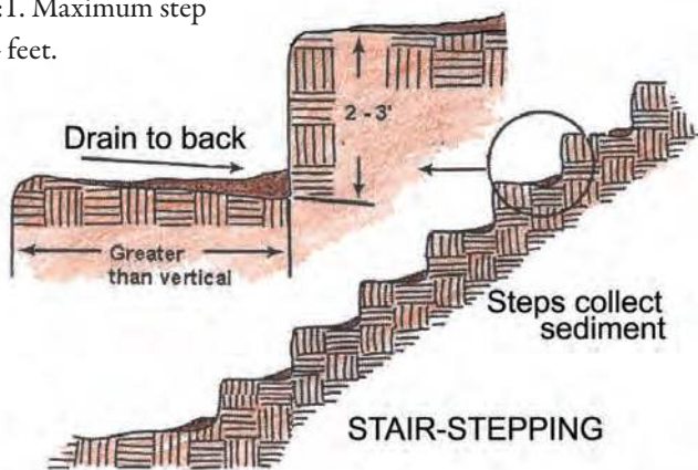
Figure 4.2. Stair-step grading to protect slopes.
