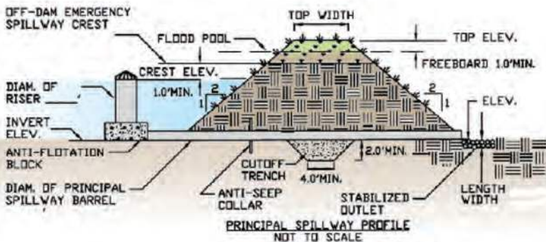
Figure 3.8. Sediment basin spillway profile. Basins located in limestone may not need an outlet.
