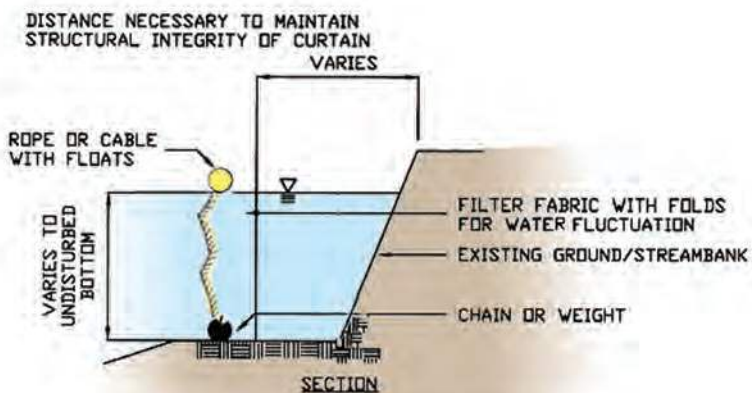
Figure 2.6. Typical turbidity curtain with flotation and anchoring devices.
