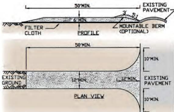
Figure 2.2. Stabilized construction entrance with optional mountable berm.
