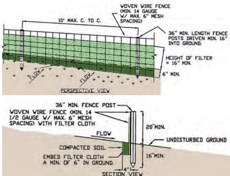
Figure 2.3. Silt fence installation with wire mesh support.
