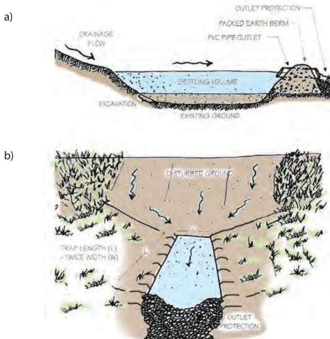
Figure 3.7. Examples of excavated traps with (a) pipe or (b) rock outlet (AS-EPA Guidance Manual for Runoff Control, 2001). Traps located in limestone may not need an outlet.
