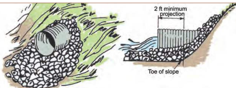
Figure 5.5. Protect outfalls without headwalls (Source: British Columbia, 2001).
