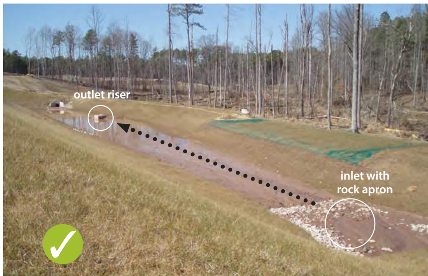
Large sediment basin to be converted to permanent stormwater practice once construction complete and accumulated sediment is removed. Good distance from inlet to outlet riser. Good stabilization of side slopes and spillway.
