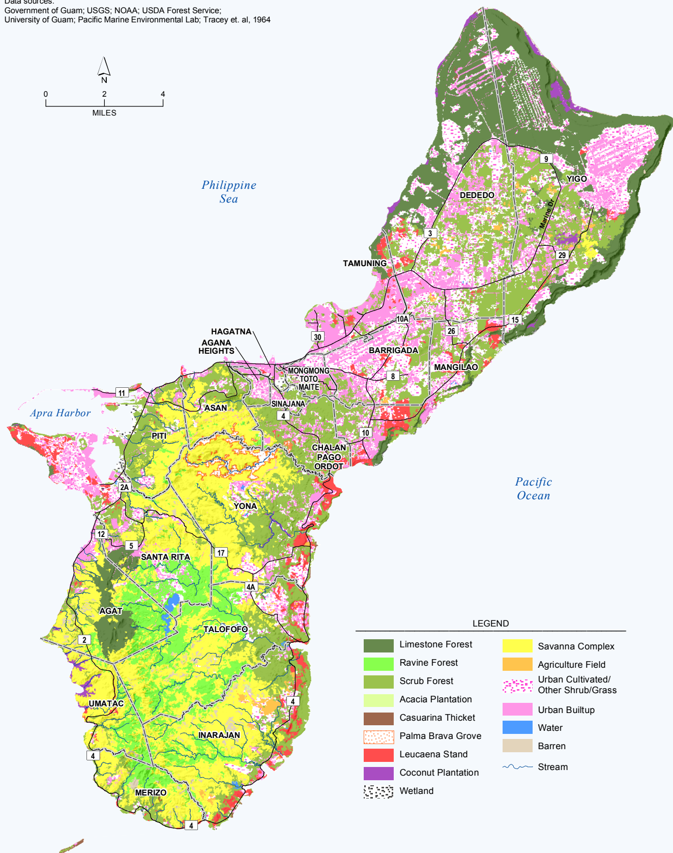
Figure D-4 Vegetation
