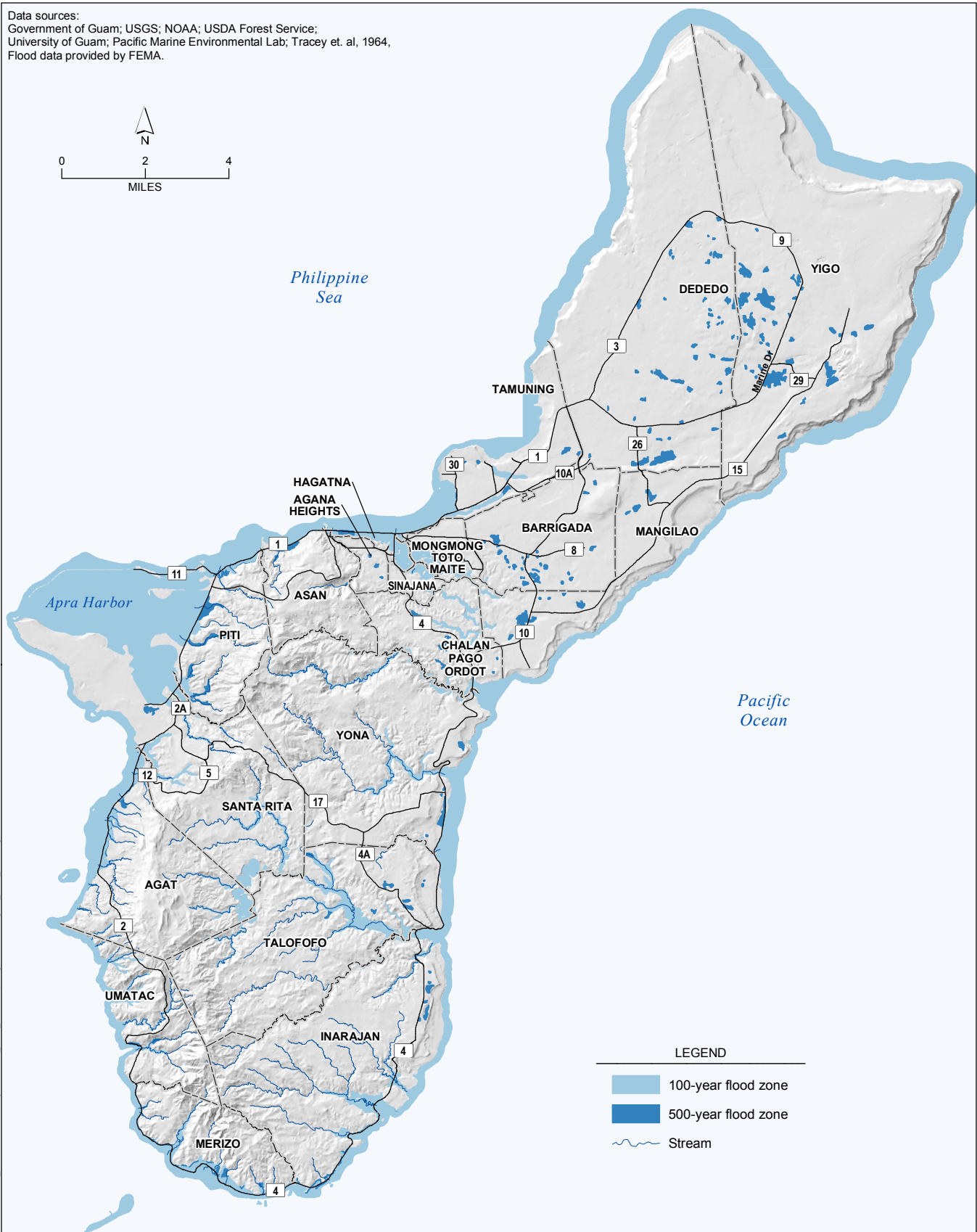
Figure D-17 Special flood hazard area
