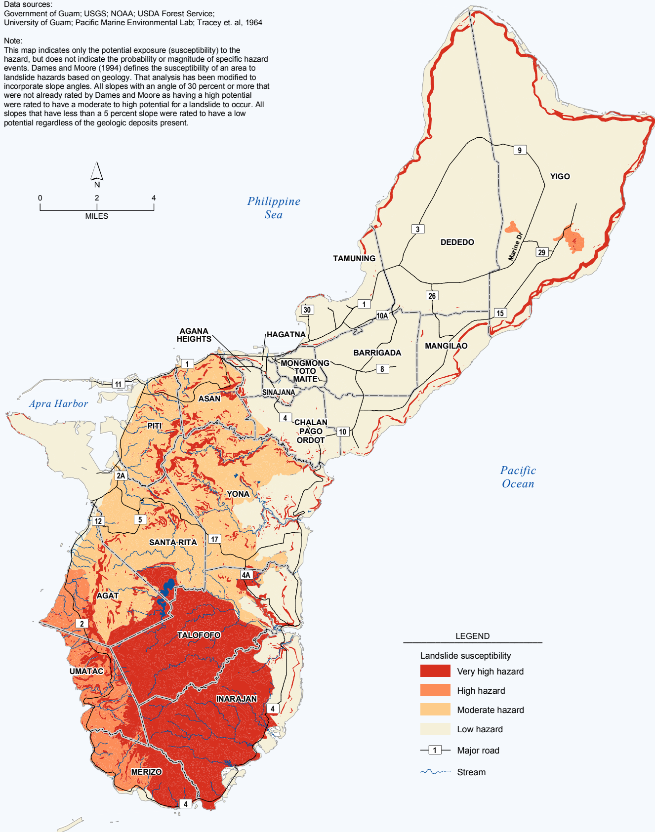
Figure D-23 Landslide susceptibility
