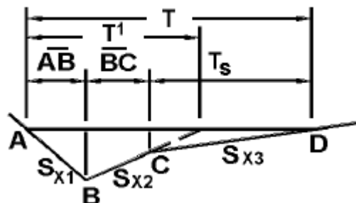
No Curb, V-Shaped Gutter
