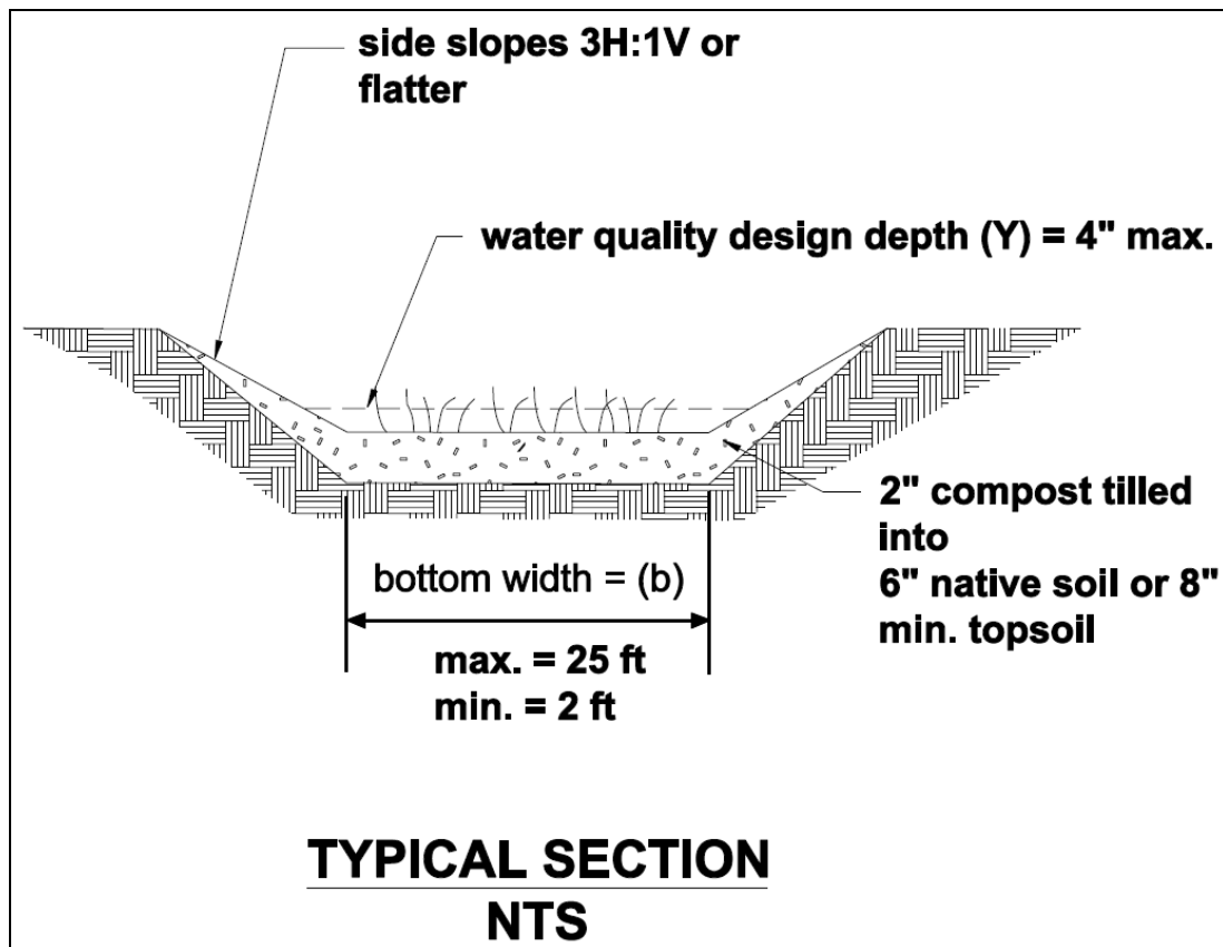
Figure 6-21: BMP RT.05 - Wet Biofiltration Swale
