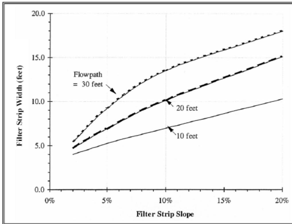
Figure 6-16: Narrow-Area Vegetated Filter Strip Design
