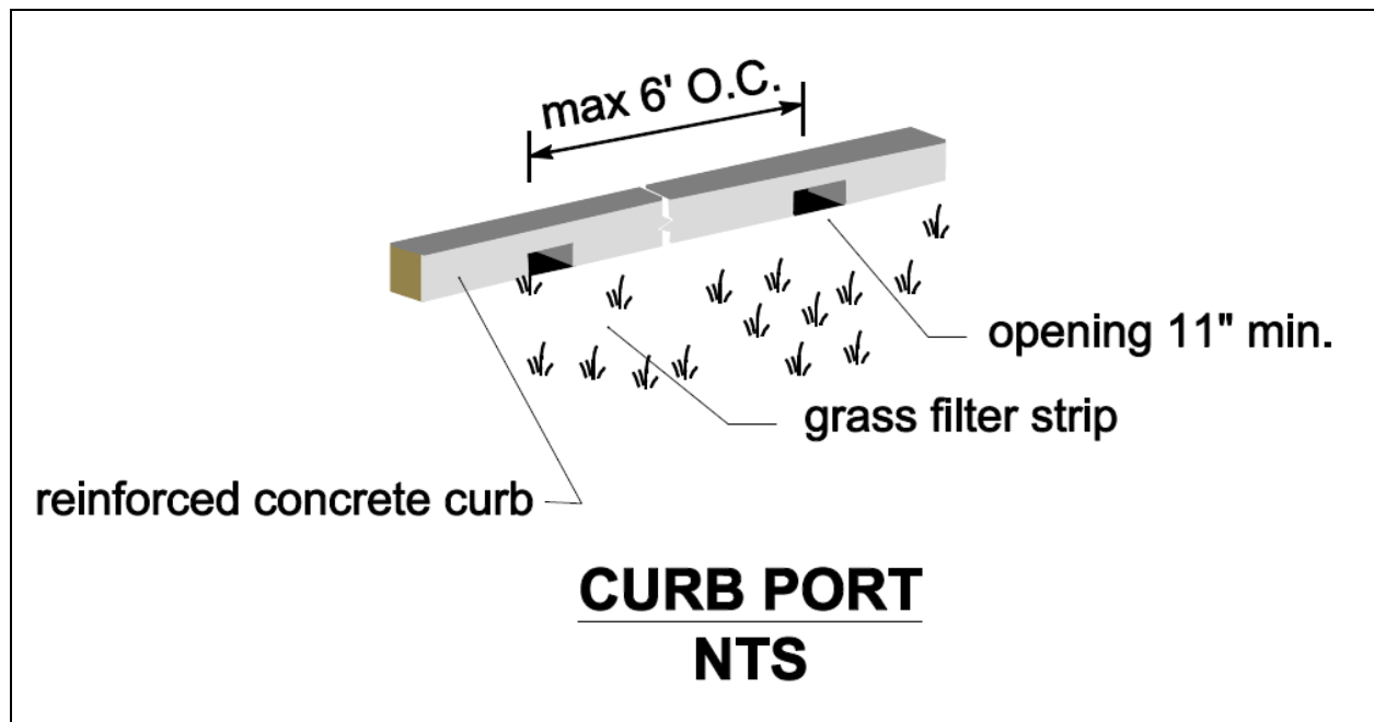
Figure 6-44: Flow Spreader – Through-Curb Port
