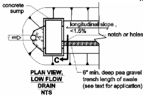
Figure 6-20: Bioinfiltration Swale Details
