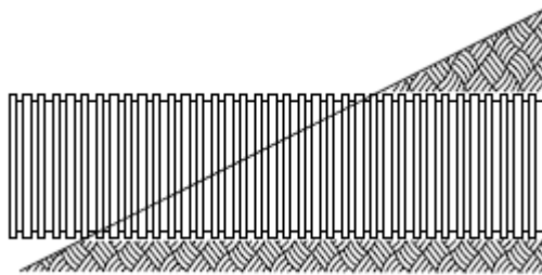
Figure 5-5: Projecting End
