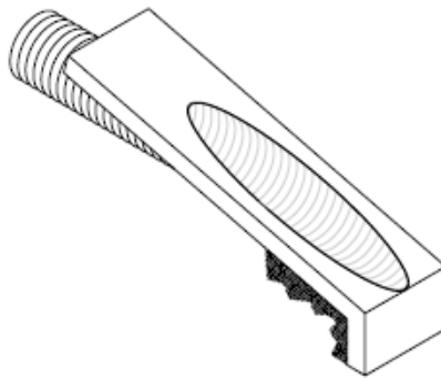
Figure 5-8: Slope Collar
