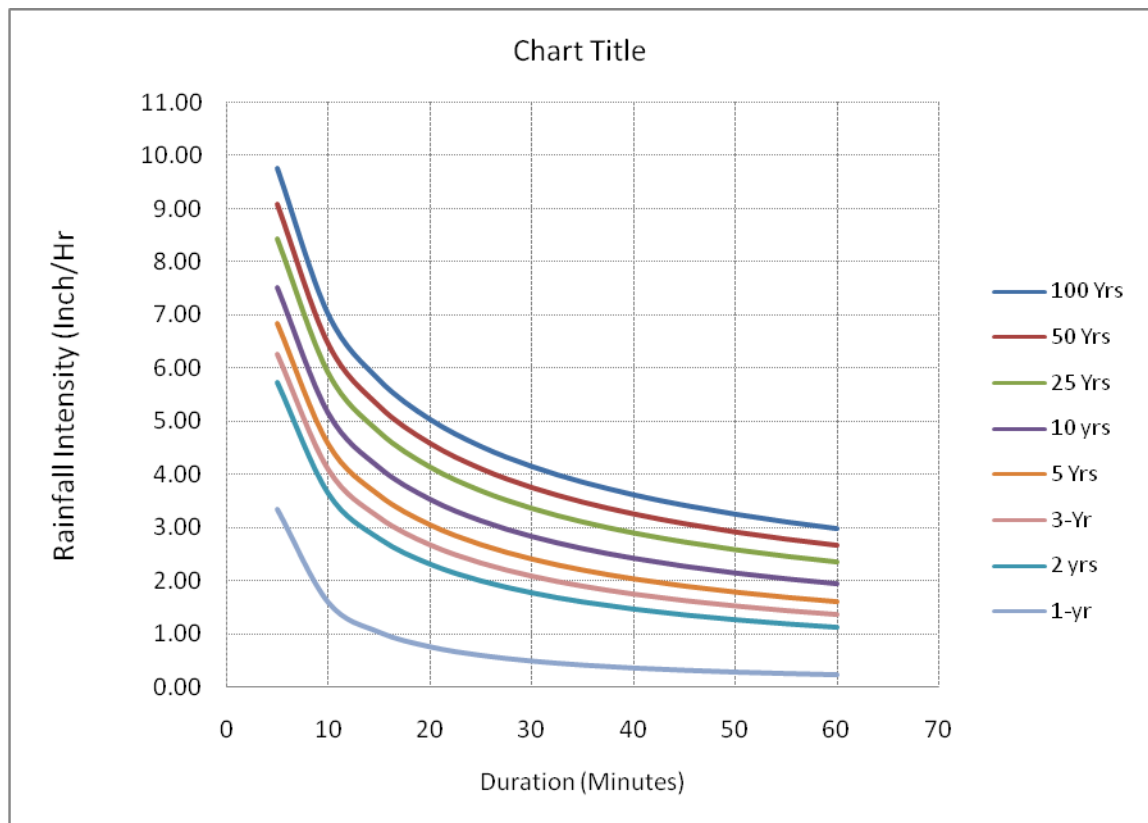
Figure 4-1: Intensity-Duration-Frequency (IDF) Curves for a One-Hour Duration Storm
