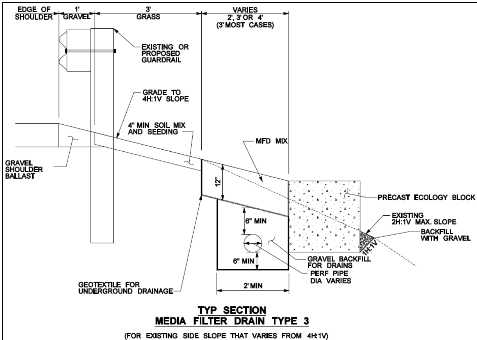
Figure 6-25: BMP RT.07 - Media Filter Drain Type 3
