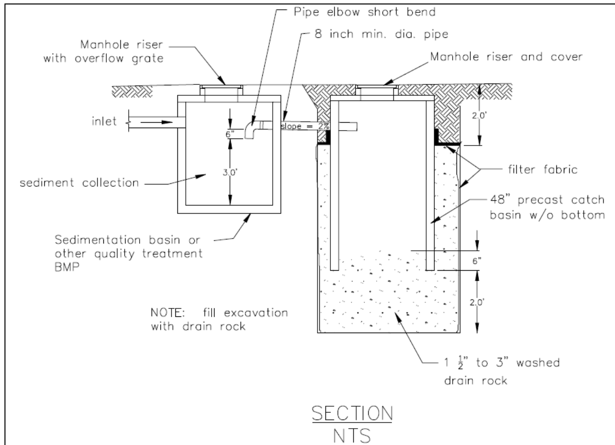
Figure 6-13: BMP IN.05 - Drywell
