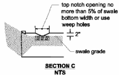
Figure 6-20: Bioinfiltration Swale Details
