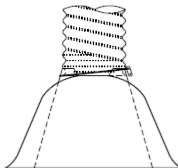
Figure 5-7: Flared End Section
