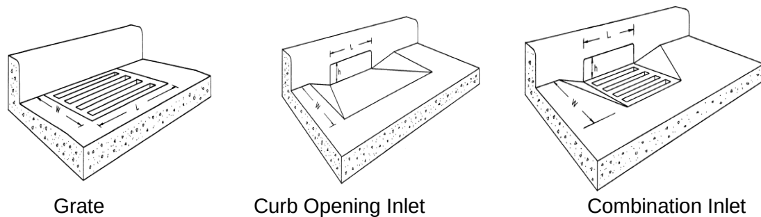
Figure 5-2: Perspective View of Gutter and Curb Opening Inlets
