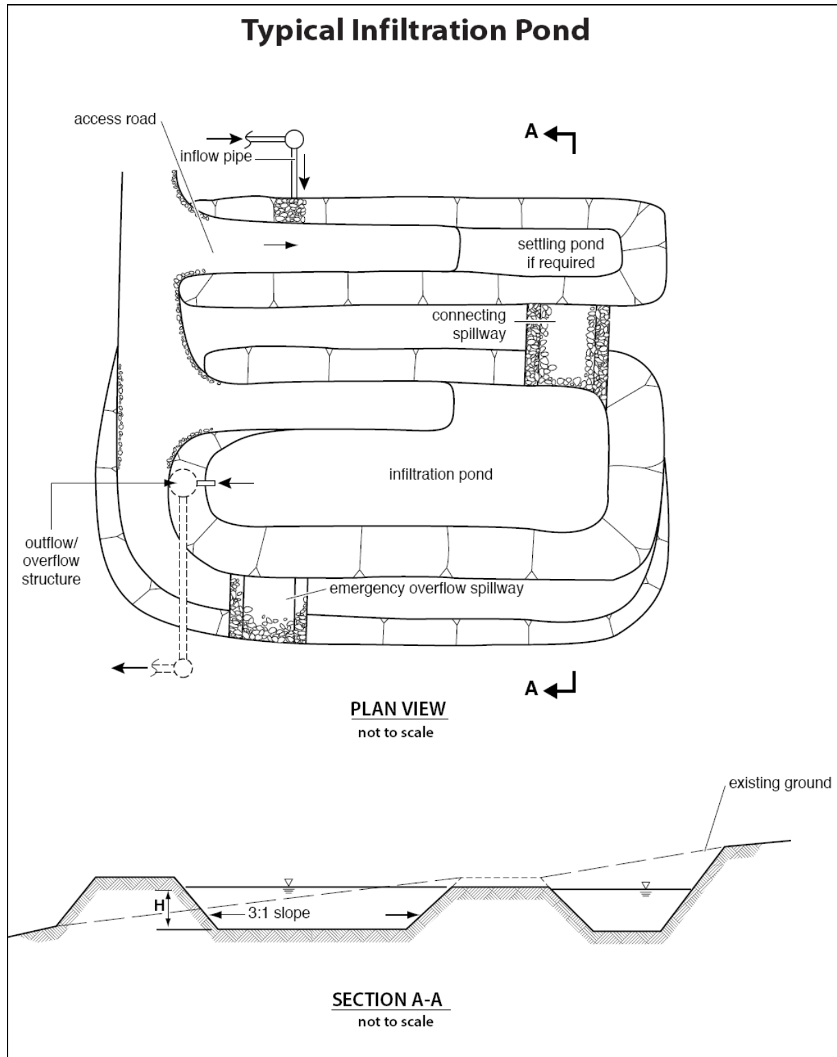
Figure 6-5: Infiltration Pond
