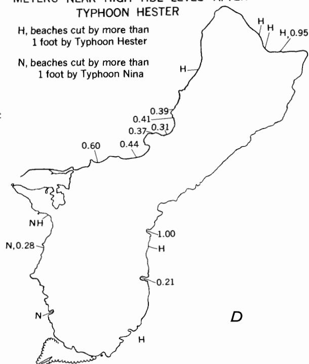
FIGURE 51.—Beach sands. A, Locality numbers of beach samples and beach profiles (fig. 54). B, Percentage insoluble residue of high-tide samples. C, Median diameter, in millimeters, of high-tide and adjacent low-tide samples. D, Changes produced by Typhoons Hester and Nina.
