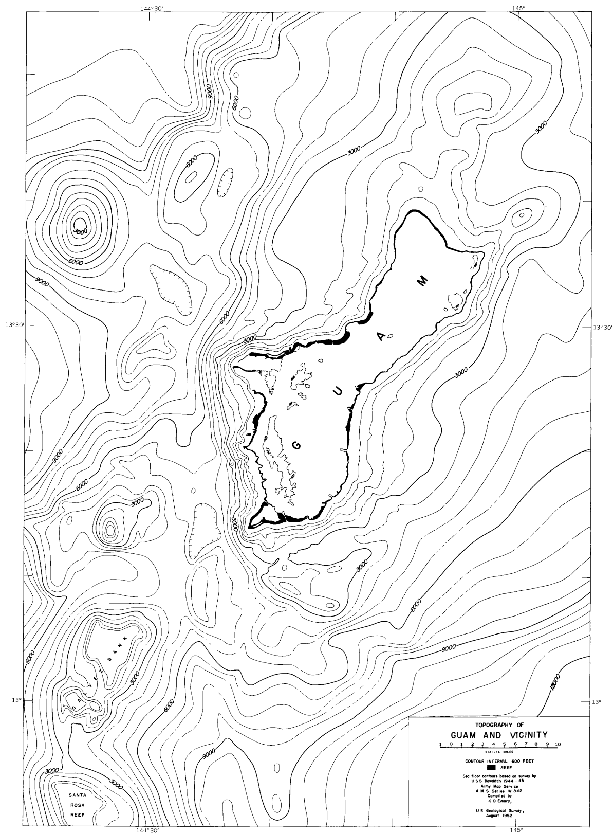
FIGURE 3.—Bathymetric chart of Guam and vicinity. Contour interval is 600 feet (100 fathoms) on both land and sea floor. Reef areas shown by solid black pattern.
