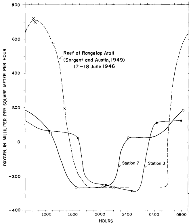
FIGURE 50.—Oxygen gain (values above zero) and loss (values below zero) at two stations of reef at Agana Bay as compared with reef at Rongelap Atoll.
