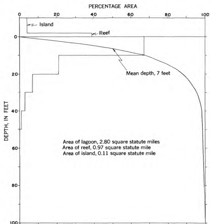
FIGURE 15.—Histogram and cumulative depth curves of Cocos Lagoon.
