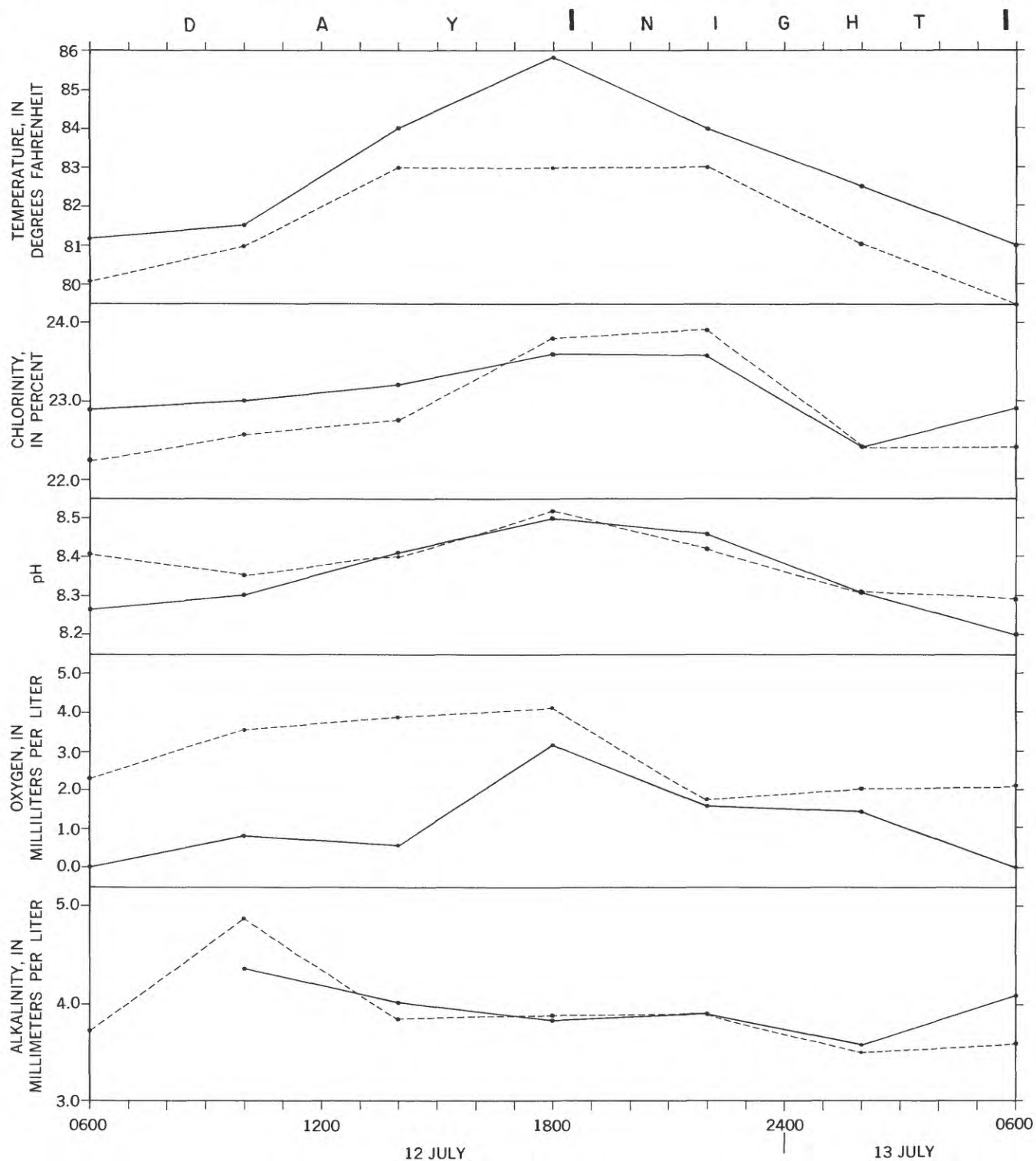
FIGURE 65.—Typical diurnal changes in the characteristics of the water in solution basins. Dashed line is for surface water and solid one is for bottom water withdrawn by a siphon hose. Basin is 24 inches wide, 24 inches long, 3 inches deep, and contains about 14 quarts of water. It is about 2 feet above high tide.
