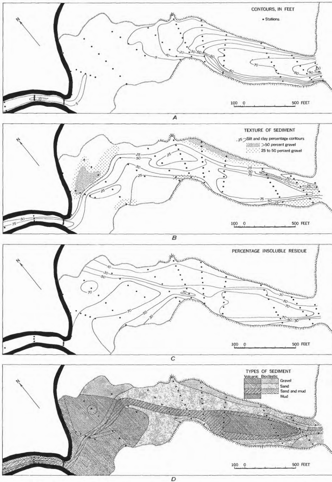
FIGURE 33.—Pago Channel—topography, sediment grain size, percentage insoluble residue, and types of sediment.
