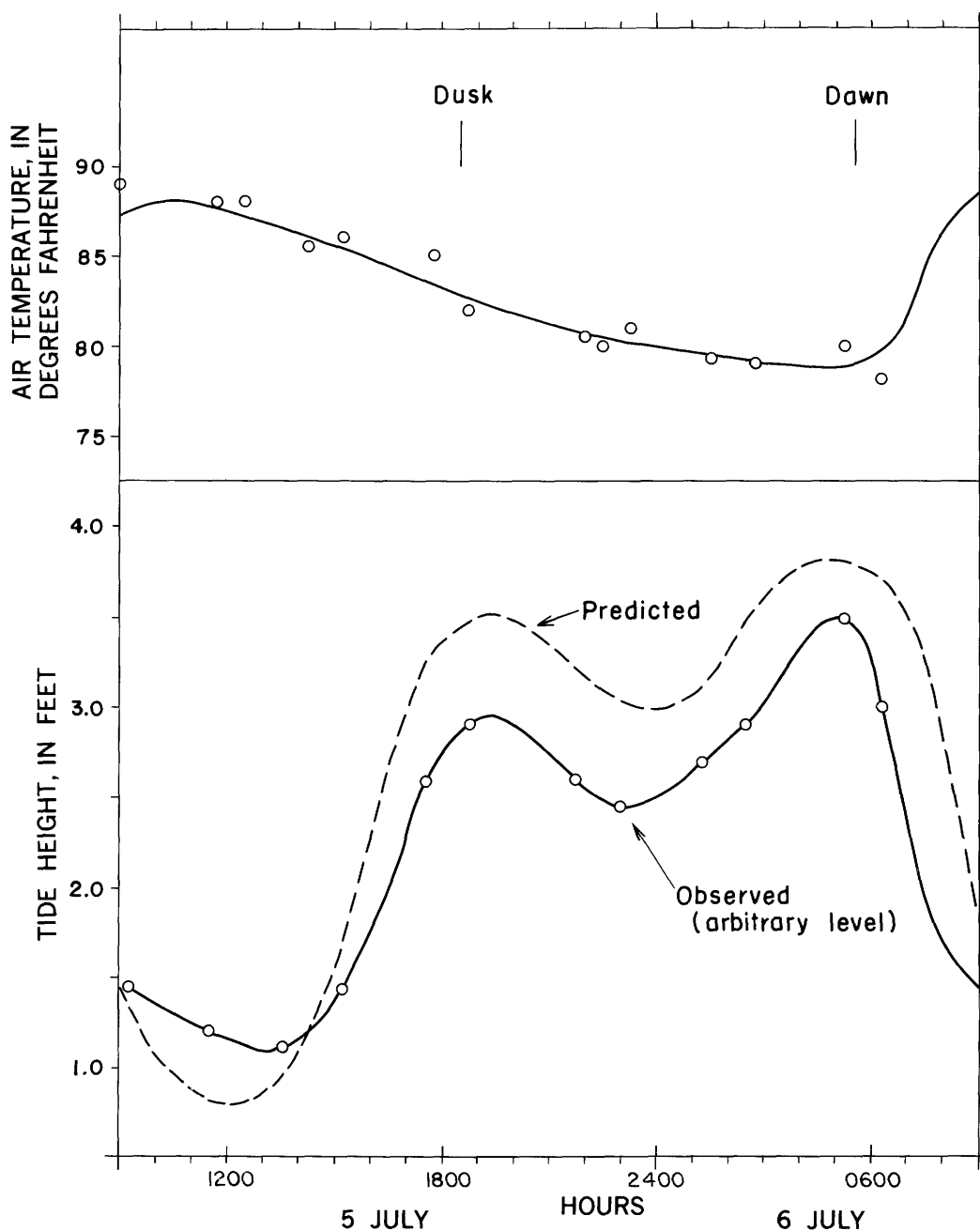
FIGURE 48.—Air temperature and tide curves during the study of reef water at Agana Bay.
