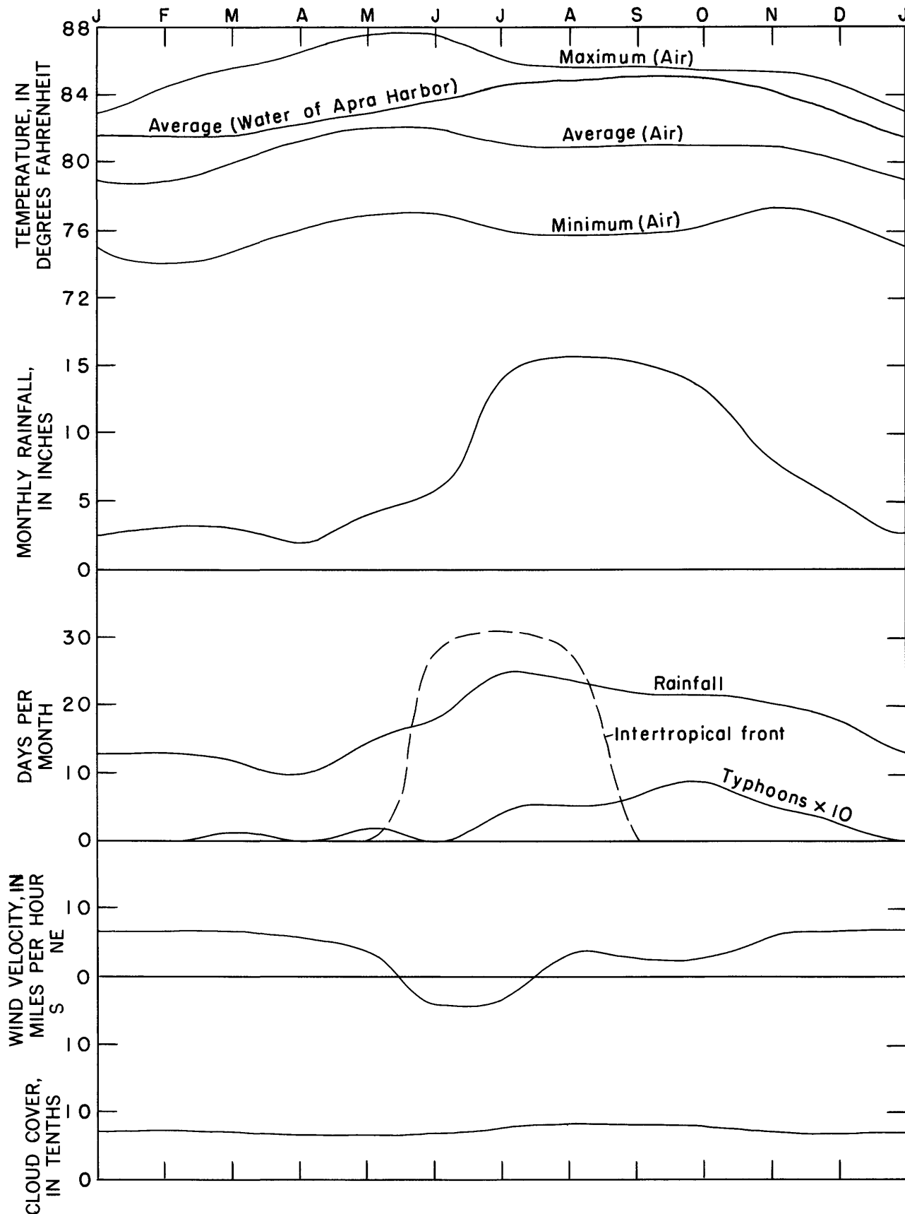
FIGURE 1.—Climatological data for Guam. Ten-year (plus) summary before October 1949 is largely from Combs (1949). Data on water temperature are from the U.S. Coast and Geodetic Survey.
