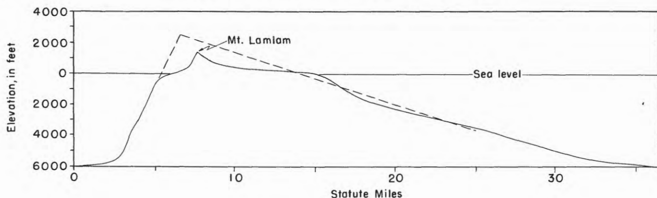
FIGURE 5.—East-west profile through Mount Lamiam. Lower profile has vertical exaggeration of \times 5 ; upper one has identical vertical and horizontal scales.
