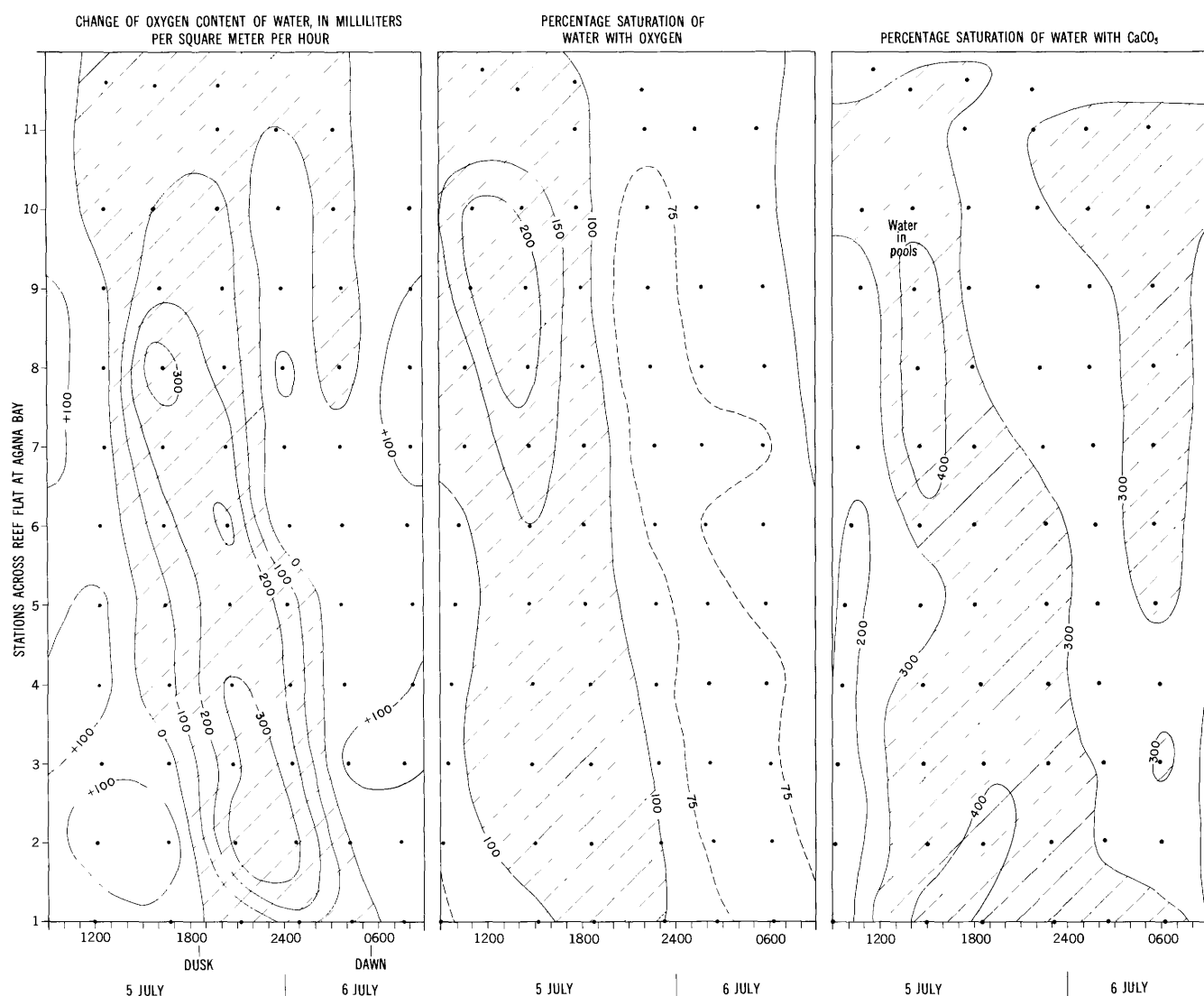
FIGURE 49.—Oxygen production, oxygen percentage saturation, and calcium carbonate percentage saturation in water of reef at Agana Bay.
