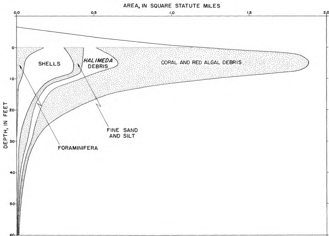
FIGURE 25.—Vertical distribution of sediment composition corrected for actual area of the lagoon floor at various depths.
