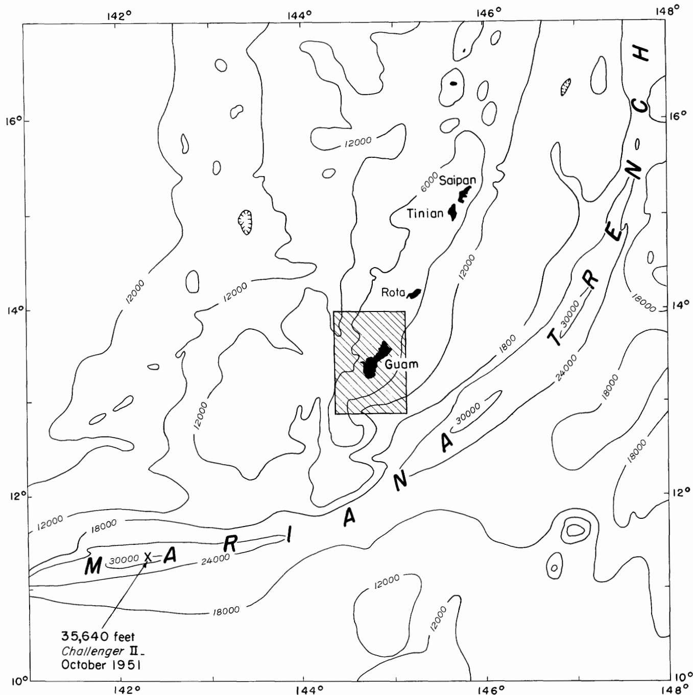
FIGURE 2.—General bathymetric chart of region (adapted from Hess, 1948). Contour interval is 6,000 feet (1,000 fathoms). Shaded insert shows position of detailed chart of sea floor near Guam (fig. 3).
