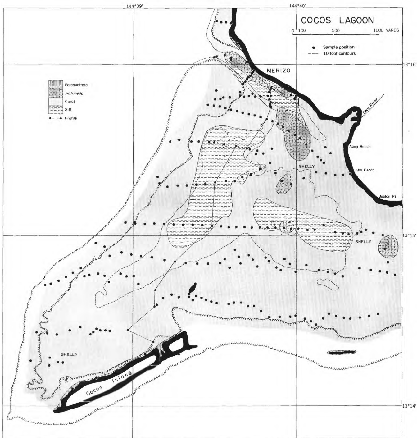
FIGURE 26.—Generalized sediment map of Cocos Lagoon.
