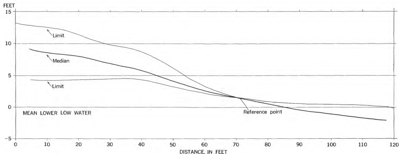
FIGURE 55.—Mean and limiting beach profiles. Reference point is 1.5 feet above mean lower low water.
