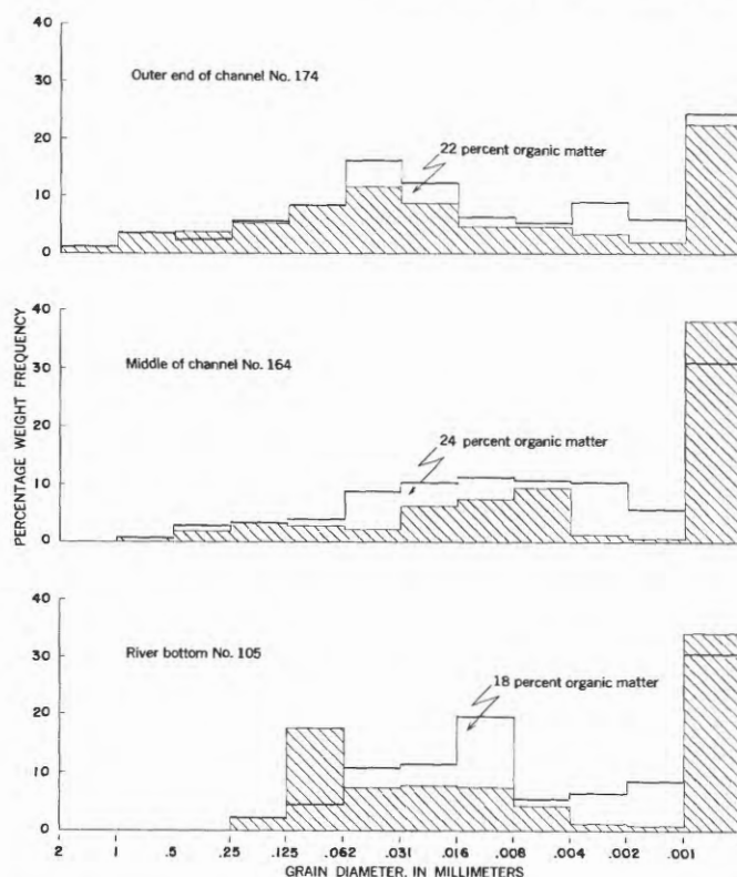
FIGURE 34.—Grain-size distribution of sediment from channel and river at Pago Bay. The heavy histograms show data for untreated samples, whereas cross-hatched portions show data for remnant of samples after organic matter was extracted with hydrogen peroxide.
