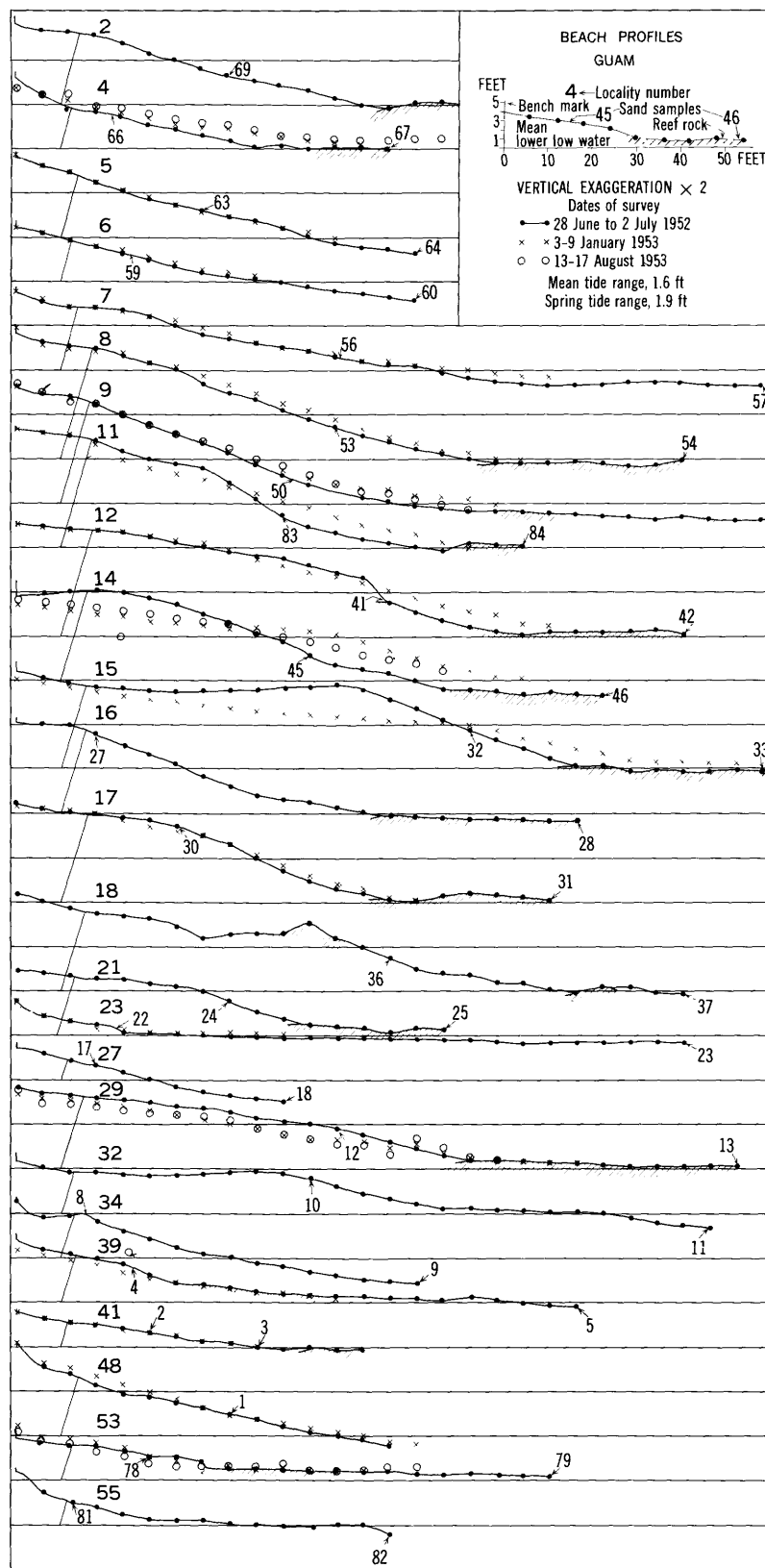
FIGURE 54.—Beach profiles at localities of figure 51A.
