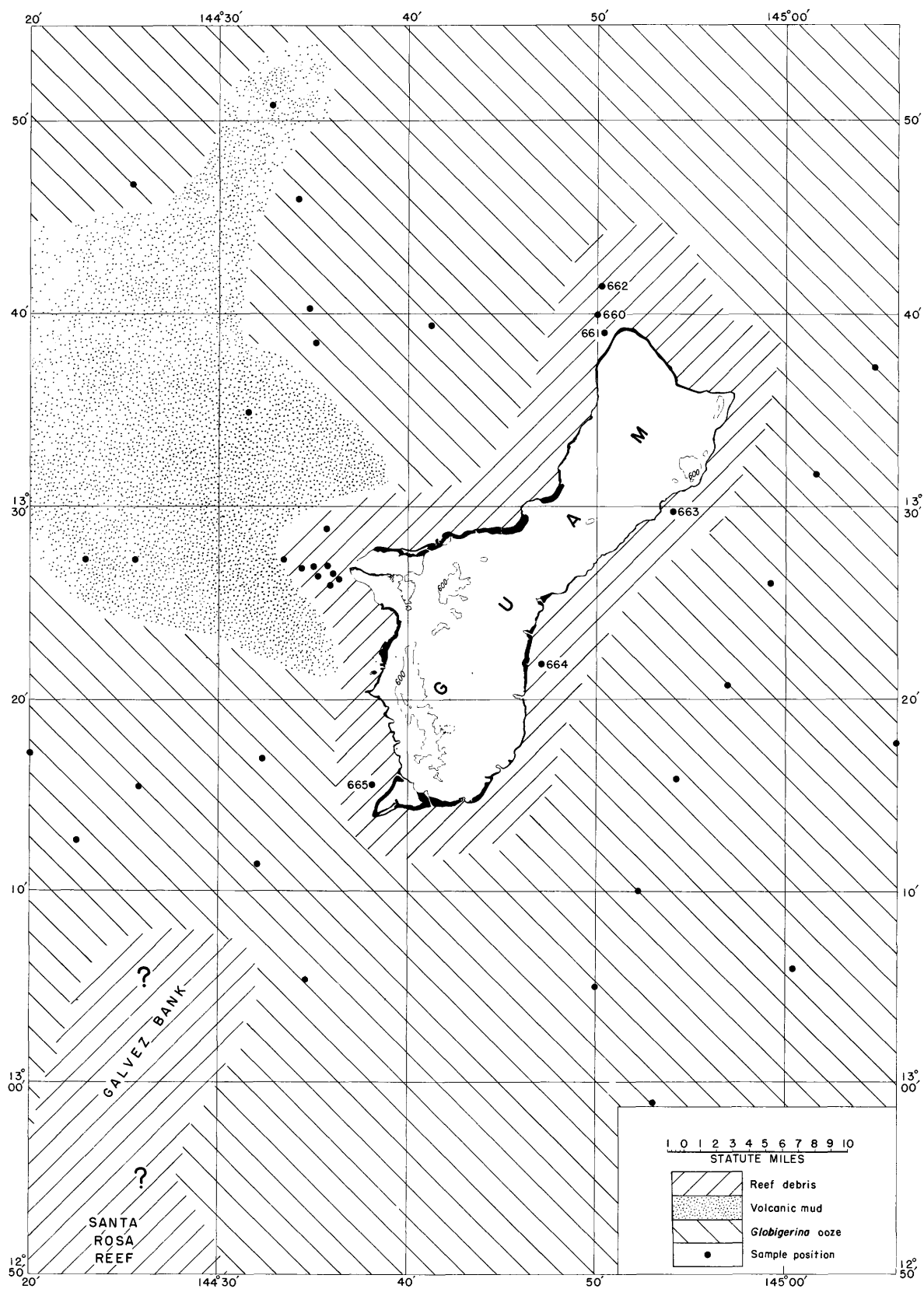
FIGURE 8.—Distribution of deep-sea sediments near Guam, compiled from various sources.
