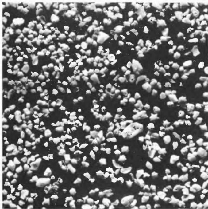
FIGURE 41.—Sample 201; Cocos Island; lat 13°14.3' N., long 144°39.1' E. Beach sand consisting dominantly of Foraminifera and comminuted coral. \times 3\frac{1}{2} .
