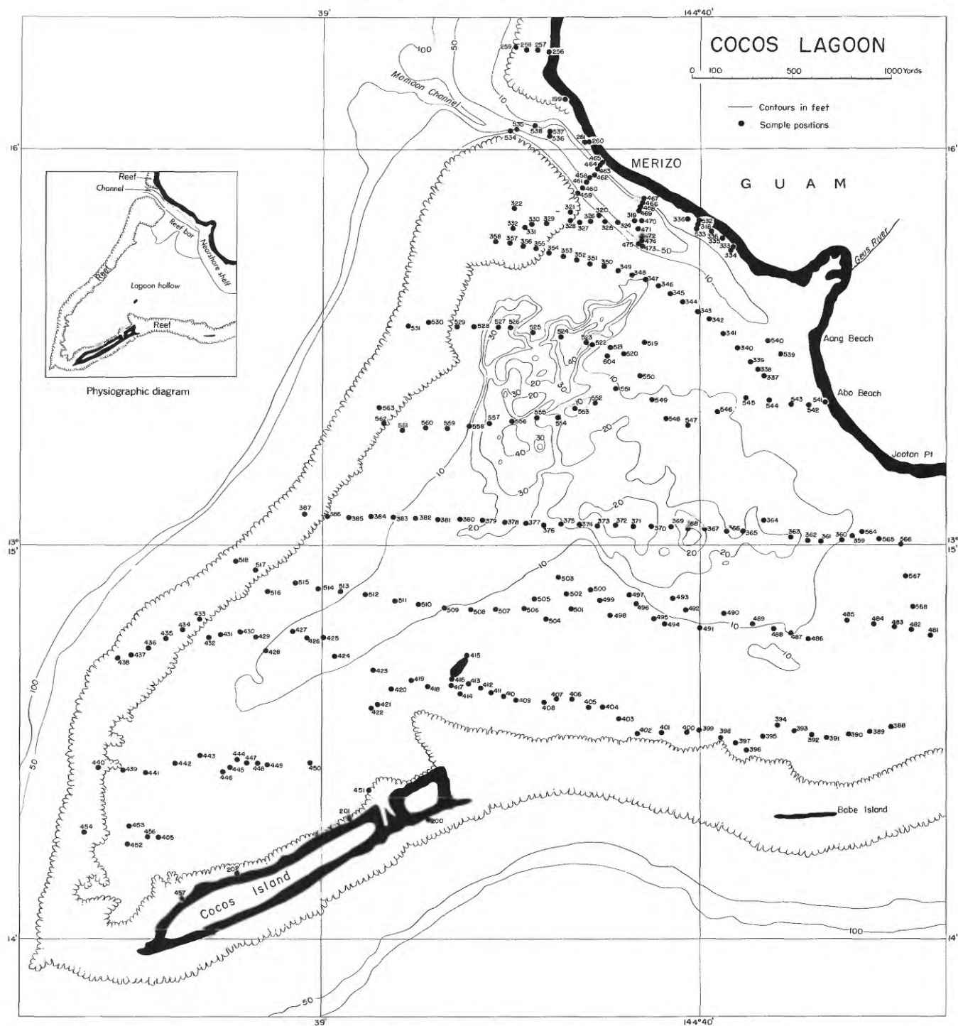
FIGURE 14.—Topography of Cocos Lagoon. Sonic soundings obtained by U.S. Navy Hydrographic Office in 1944, supplemented by data of present study. Shoreline outlined by wide black line.
