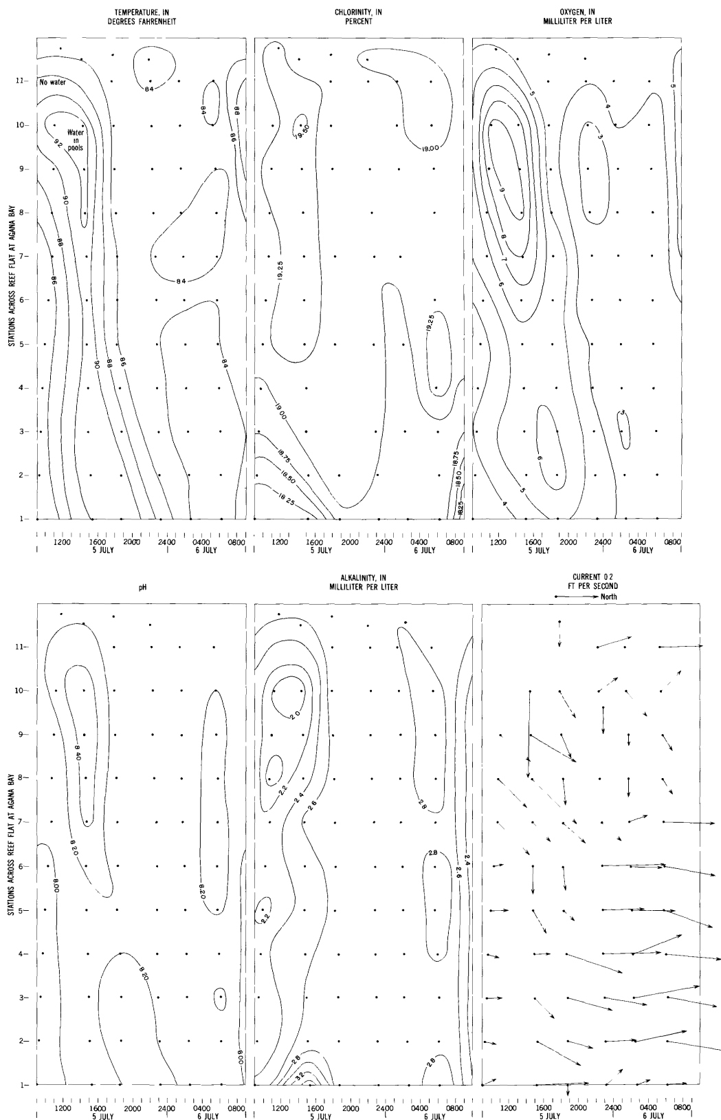
FIGURE 47.—Characteristics of water during a 24-hour study of the water at Agana Bay from shore to reef edge. Graph shows changes in water at fixed points 200 feet apart across the reef (vertical scale) with time (horizontal scale).
