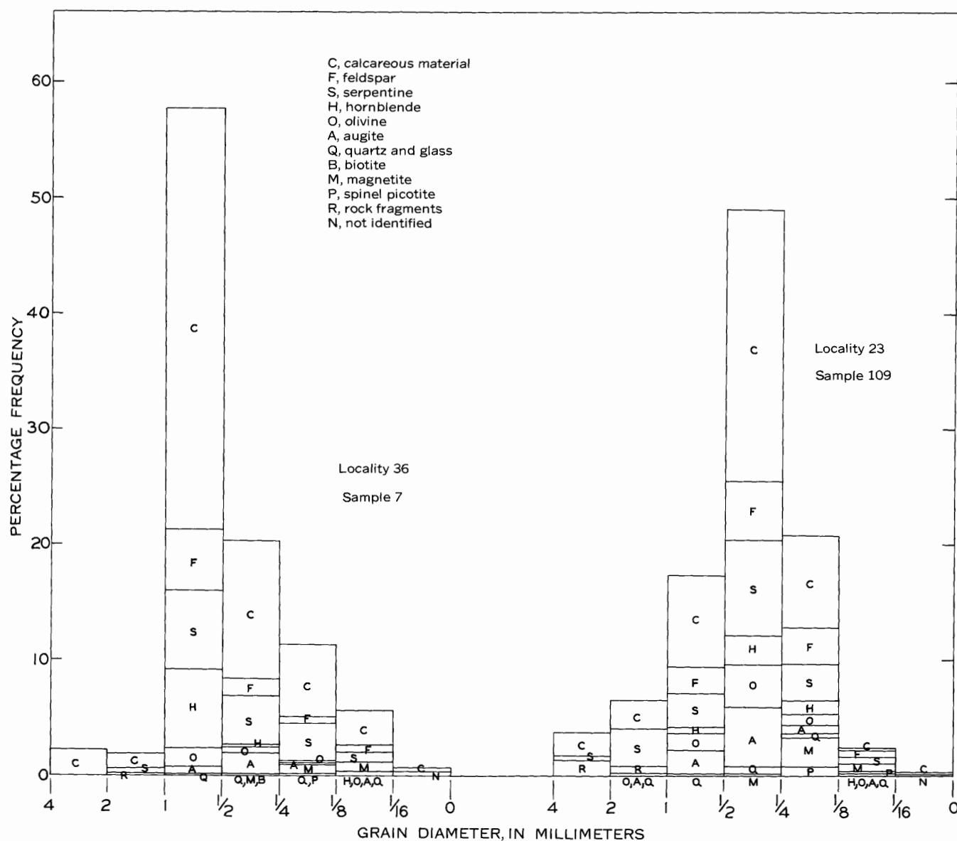
FIGURE 53.—Histograms of two beach sands that contain large percentages of detrital sediments. The size distribution of the commoner detrital minerals is also indicated.
