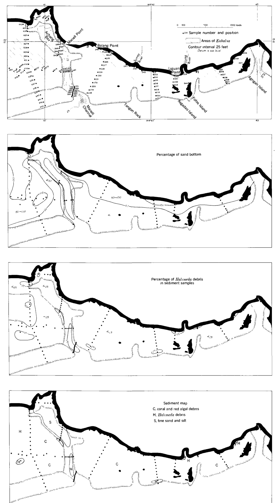
FIGURE 37.—Achang Reef—topography and surface composition.
