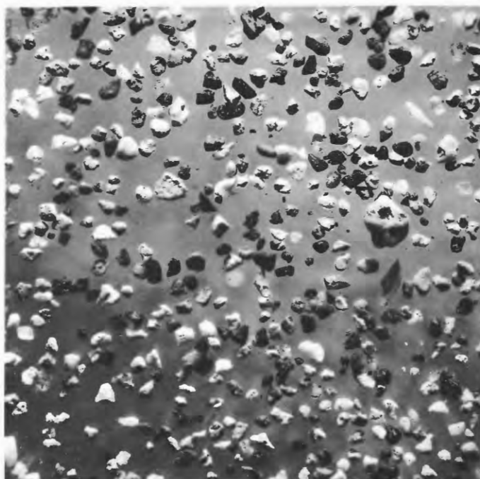
FIGURE 42.—Sample 7; Agfayan Bay; lat 13°15.9' N., long 149°44.2' E. Beach sand composed of inorganic detrital grains (mostly serpentine, hornblende, and plagioclase) that comprise 38.5 percent of whole sample; remainder is mostly comminuted coral and shells. \times 3\frac{1}{2} .
