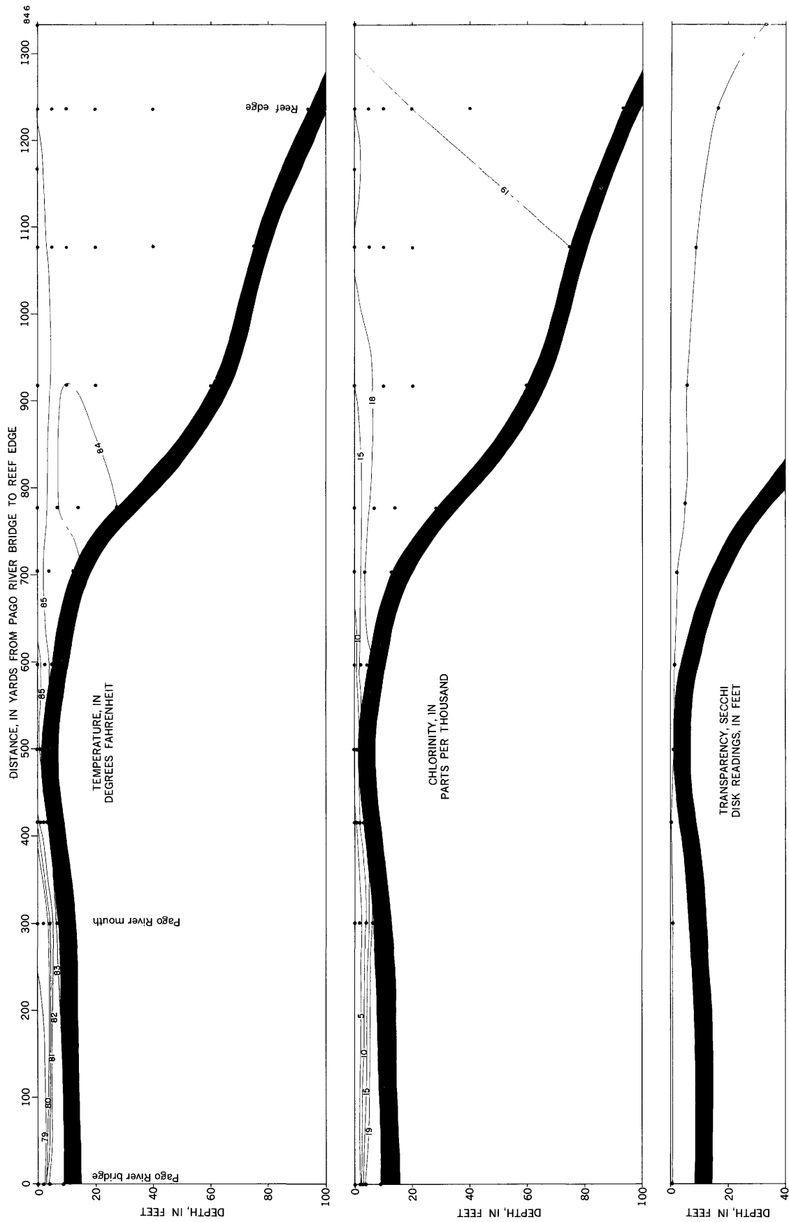
FIGURE 36.—Vertical section of water along axis of Pago Channel.
