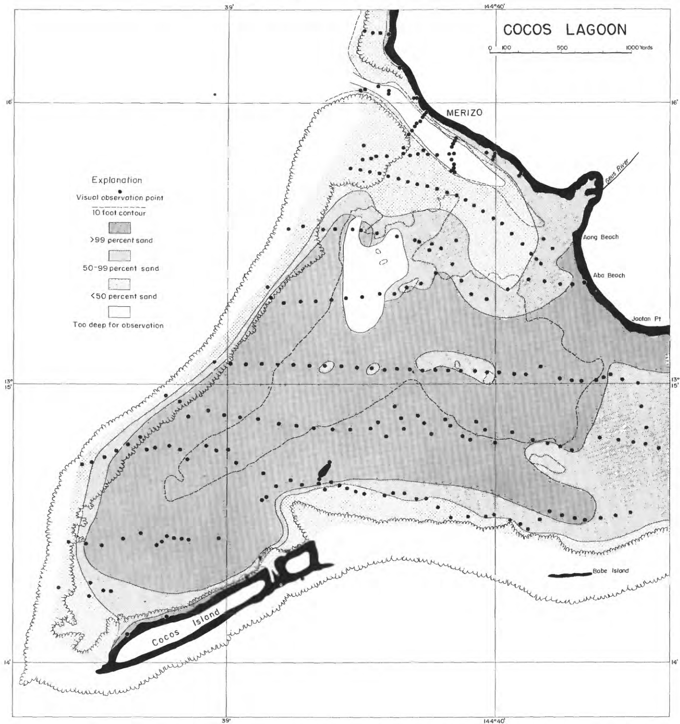
FIGURE 17.—Percentage of sand and coral bottom on floor of Cocos Lagoon. Determined by visual observation of the bottom from the launch, SES 800.
