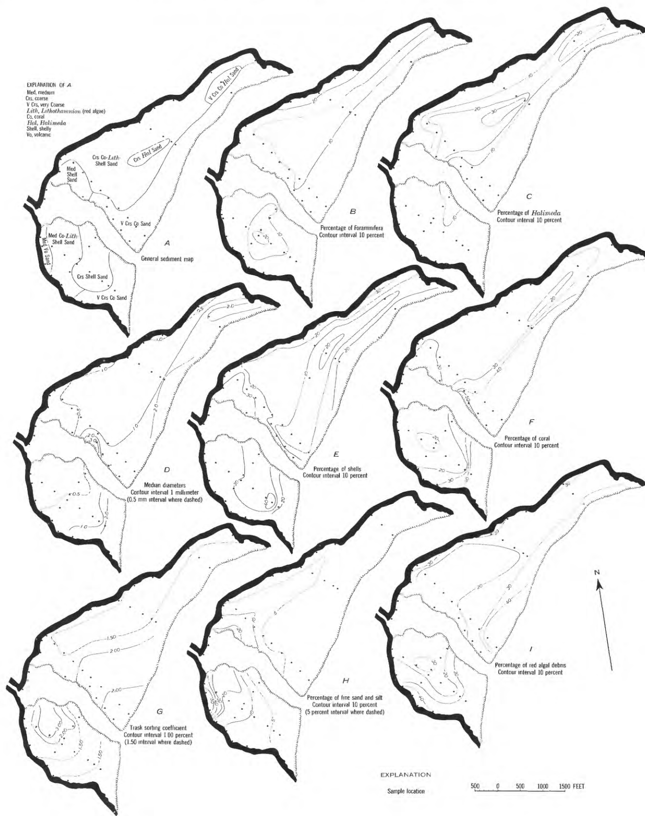
FIGURE 44.—Pago Reef—composition of sediment.
