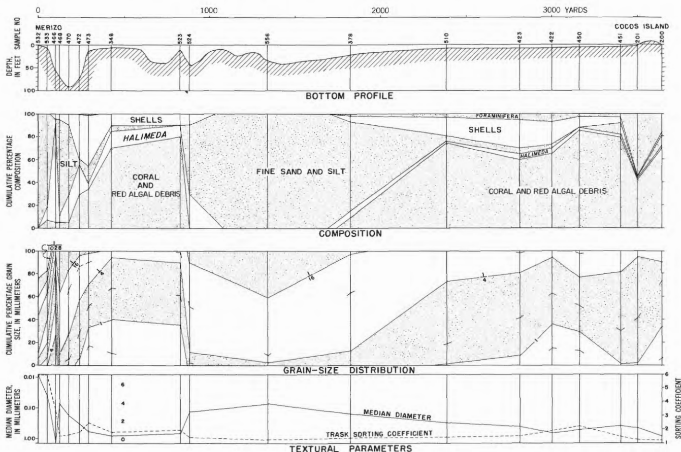
FIGURE 23.—Profile across Cocos Lagoon along line shown in figure 26. Sediment character is shown in terms of composition, grain-size distribution, and median diameter and Trask sorting coefficient.
