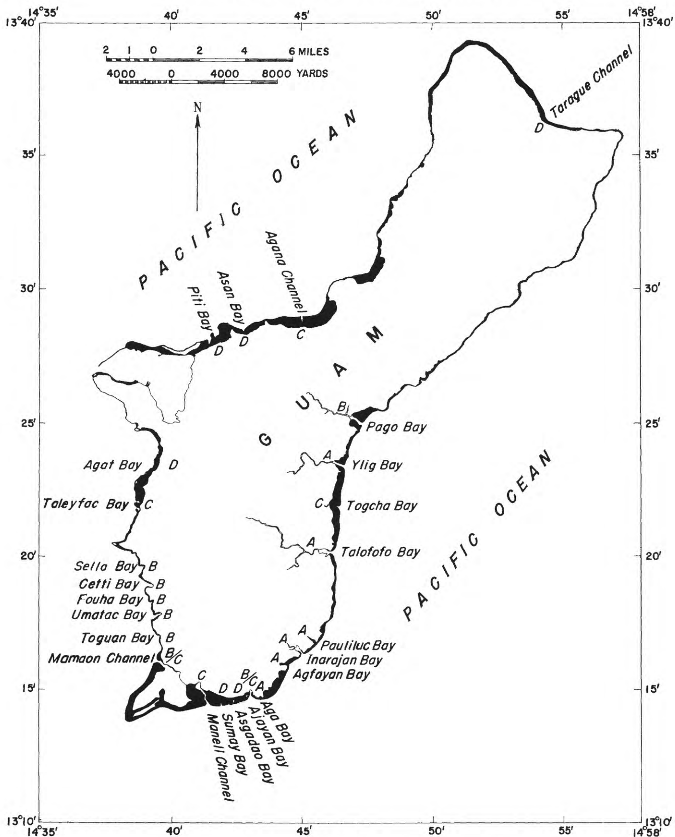
FIGURE 28.—Geographic distribution of different classes of reef indentations or channels.
