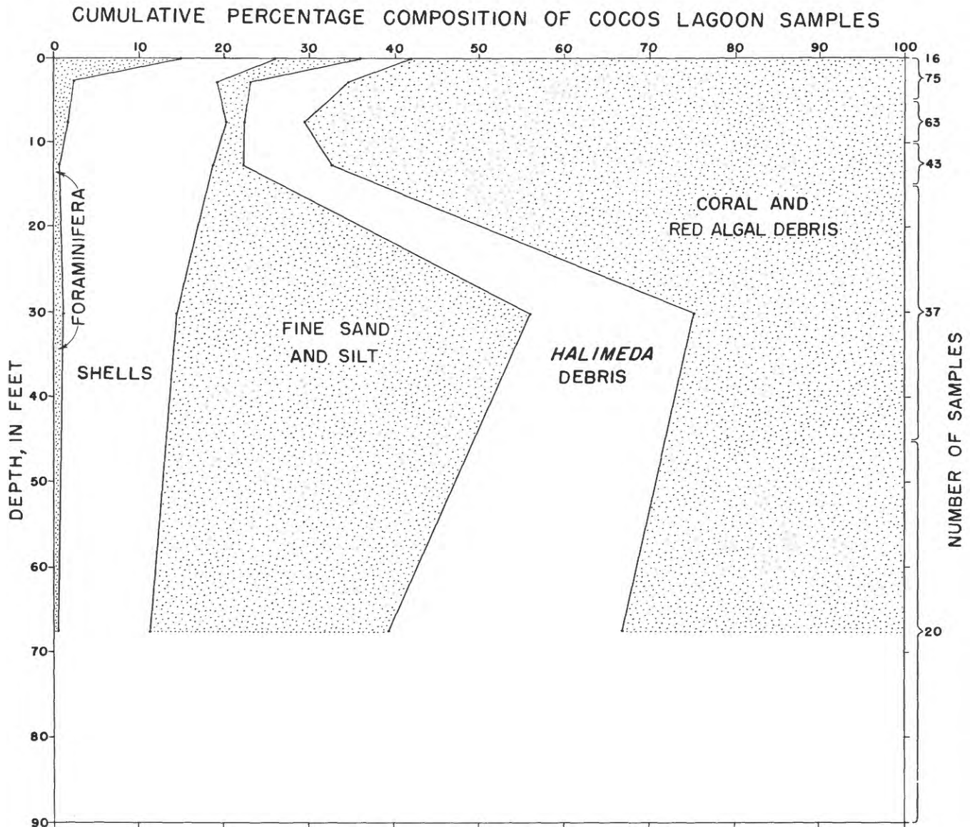
FIGURE 24.—Vertical distribution of sediment composition in terms of average percentage composition of sediment samples at various depth increments.
