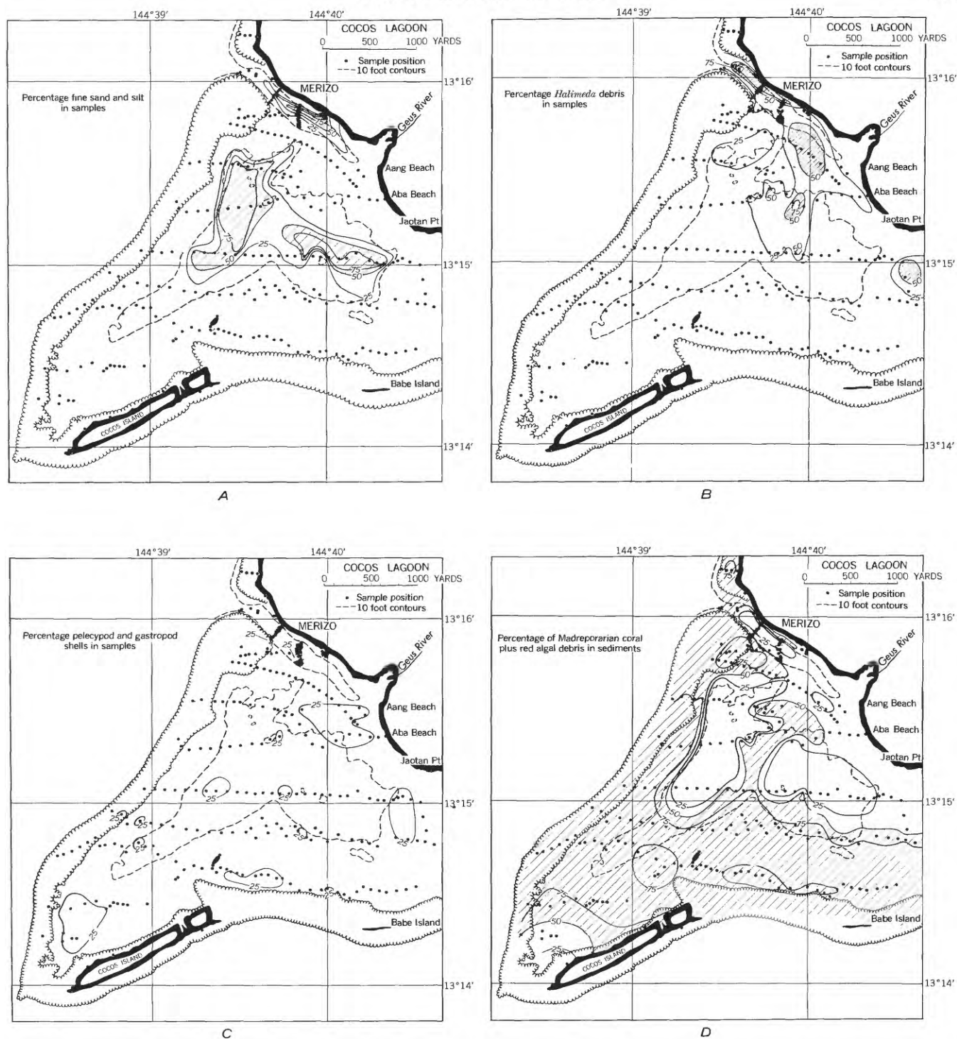
FIGURE 22.—A, Percentage of fine sand and silt in sediments of Cocos Lagoon. Dots indicate positions of bottom samples from which the data were derived. B, Percentage of Halimeda debris in sediments of Cocos Lagoon. C, Percentage of pelecypod and gastropod shells in sediments of Cocos Lagoon. D, Percentage of combined madreporarian coral and lithothamnioid algae in sediments of Cocos Lagoon.
