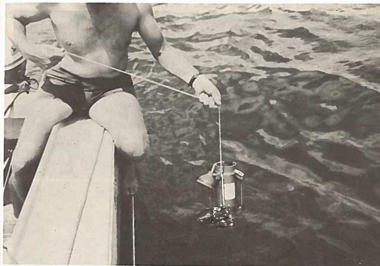
Figure 8. VAN DORN SAMPLER. The device will be messenger tripped at 10 m.
