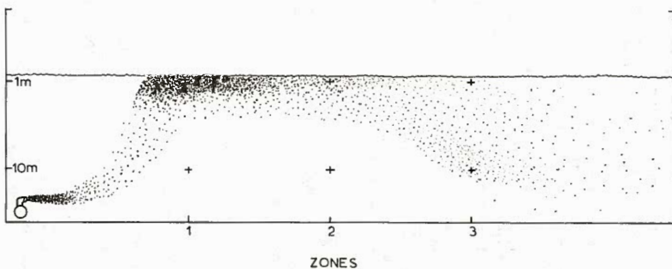
Figure 24. HYPOTHETICAL BEHAVIOR OF PLUME. The stippling shows the relative concentration of coliforms. The dimensions of this figure are not to scale.
