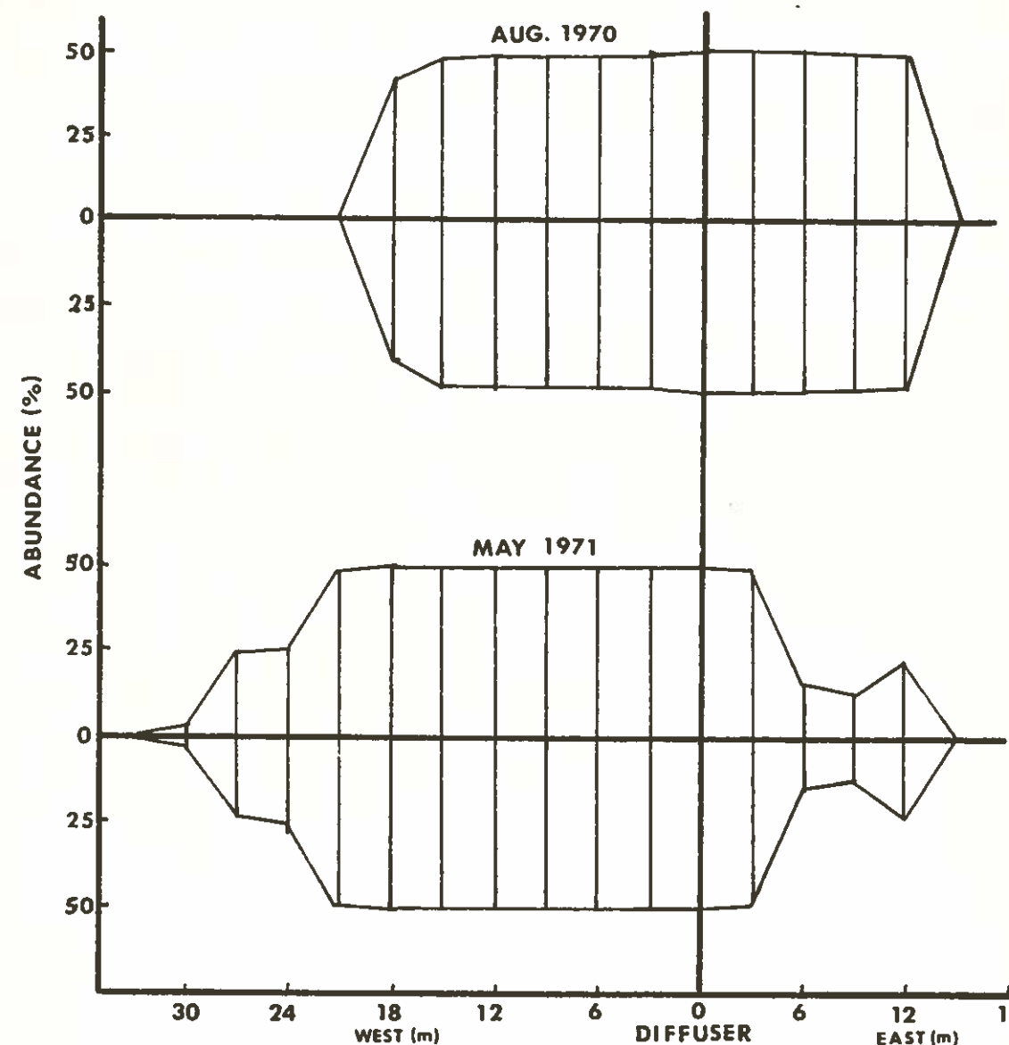
Figure 27. ABUNDANCE (%) OF CLADOPHORA SP. The diagram shows distribution on the east and west sides of the diffuser during August 1970 and May 1971.
