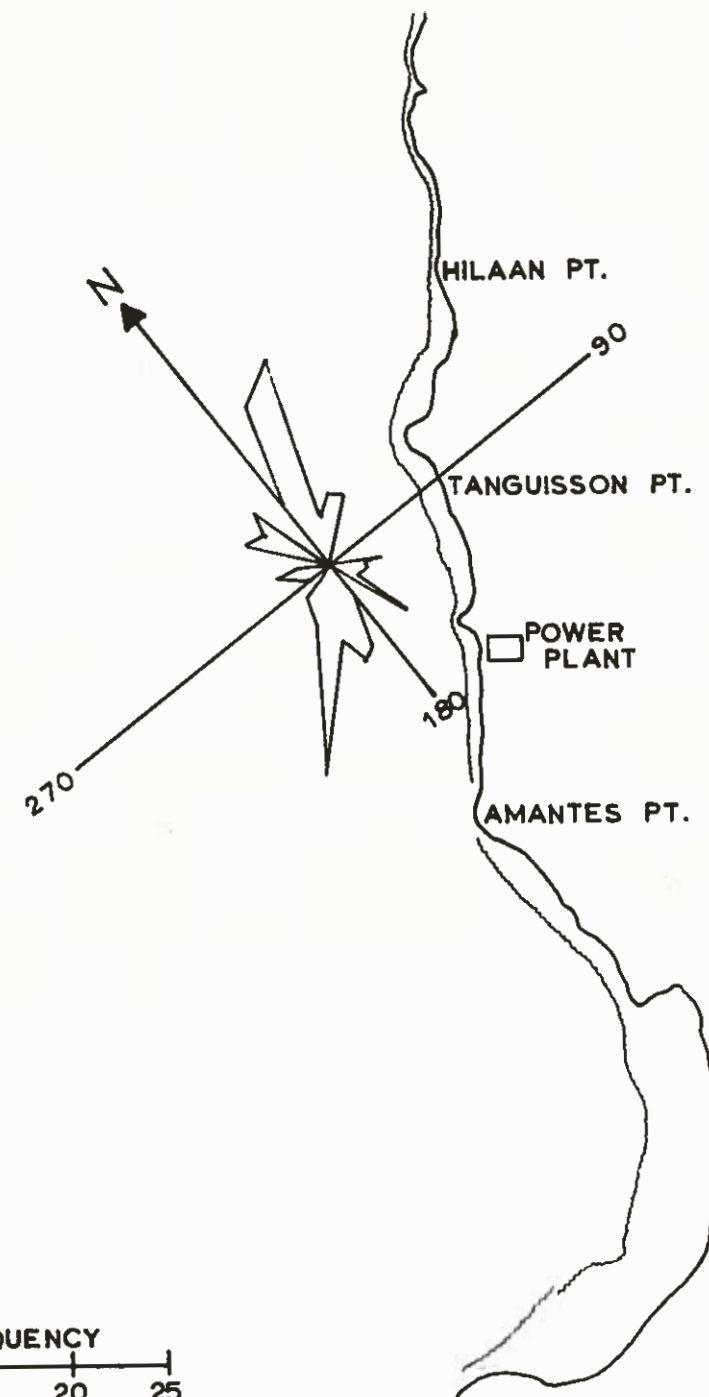
Figure 9. Mean frequency diagram for current direction at 23 m (TSK meter).
