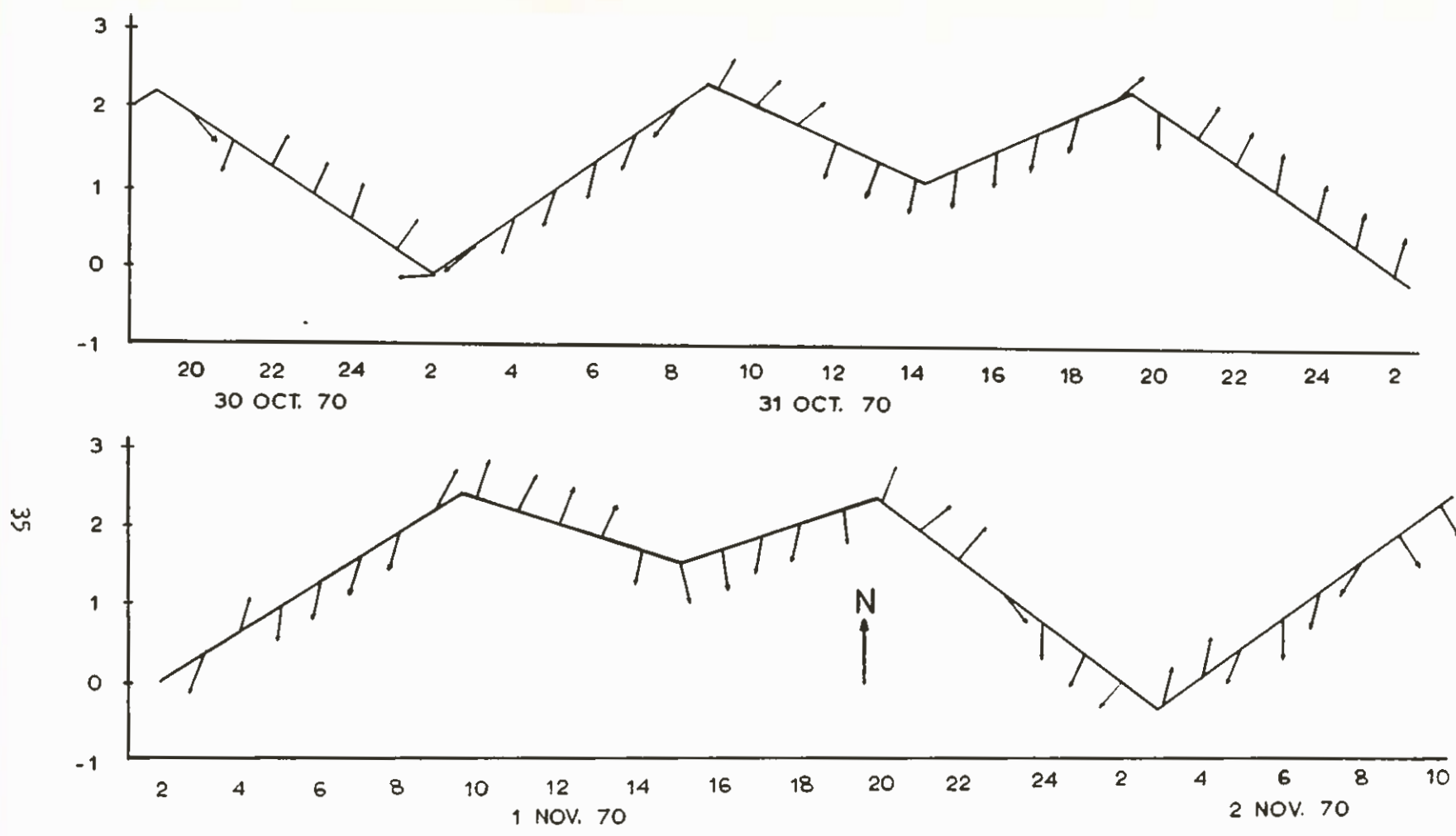
Figure 12. Sample segment from one current meter tape indicating a close fit between tide cycle and current direction. Some early shifts are evident but in general, there is a northerly set during ebb tides and a southerly one during floods. (Arrows are direction only).
