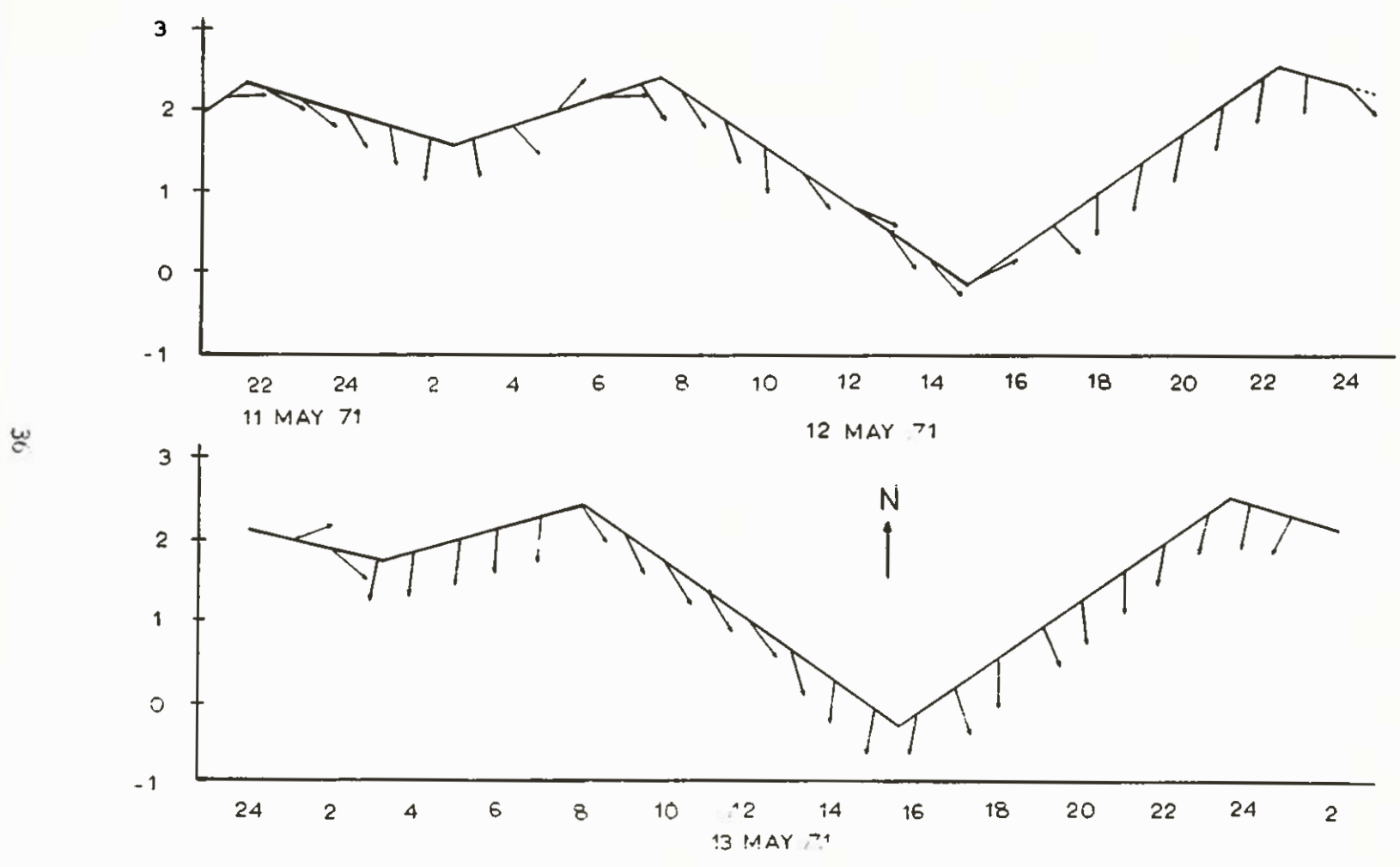
Figure 13. Sample segment from one current meter tape showing a predominance of southerly components with little correlation with tide cycle.
