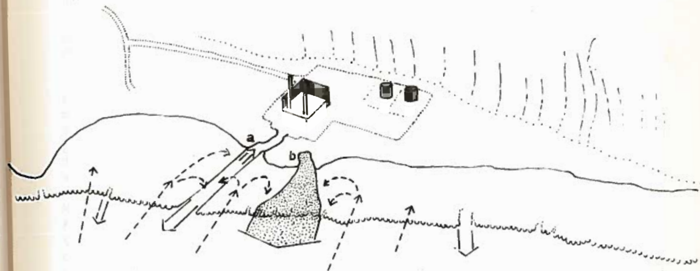
Figure 5. Current patterns on the reef flat prior to release of effluent. The dashed lines show movement of wave transported water onto the reef flat and the subsequent movements of that water along shore. The stippled arrows, labeled with roman numerals, show the major escape points of the reef flat water. (a- power plant, b- shoreline, c- reef flat, d- Naval Communications Station swimming lagoon, e- intake channel, f- outfall site).
