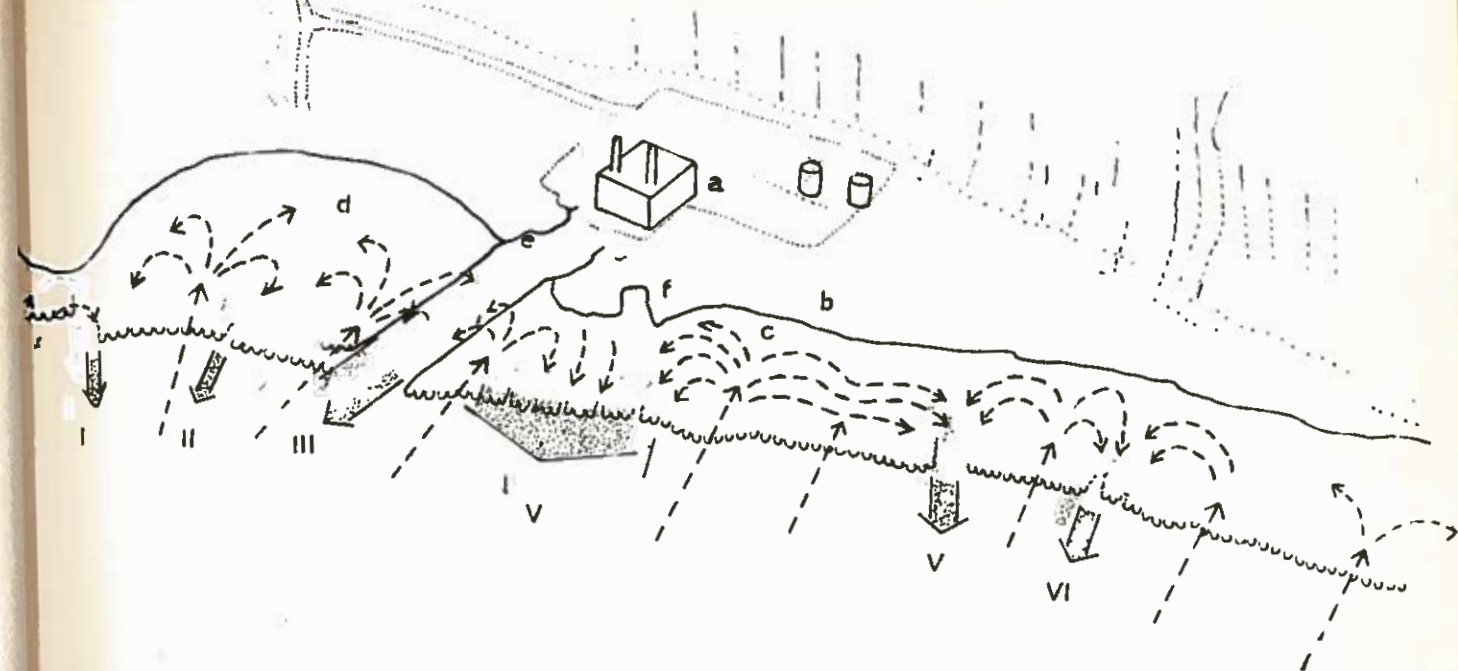
Figure 5. Current patterns on the reef flat prior to release of effluent. The dashed lines show movement of wave transported water onto the reef flat and the subsequent movements of that water along shore. The stippled arrows, labeled with roman numerals, show the major escape points of the reef flat water. (a- power plant, b- shoreline, c- reef flat, d- Naval Communications Station swimming lagoon, e- intake channel, f- outfall site).
