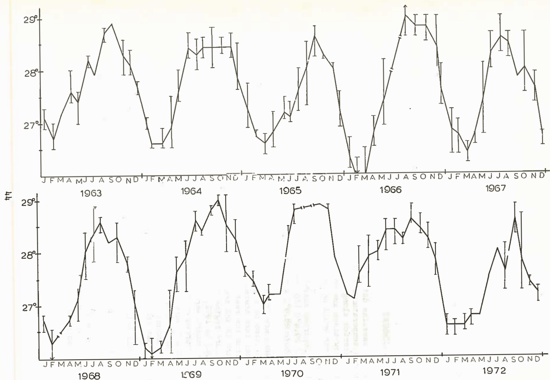
Figure 18. Plot of monthly mean sea surface temperatures for a 10 year period at Tanqissson Point Transect A. Vertical bar represents monthly range of temperatures.
