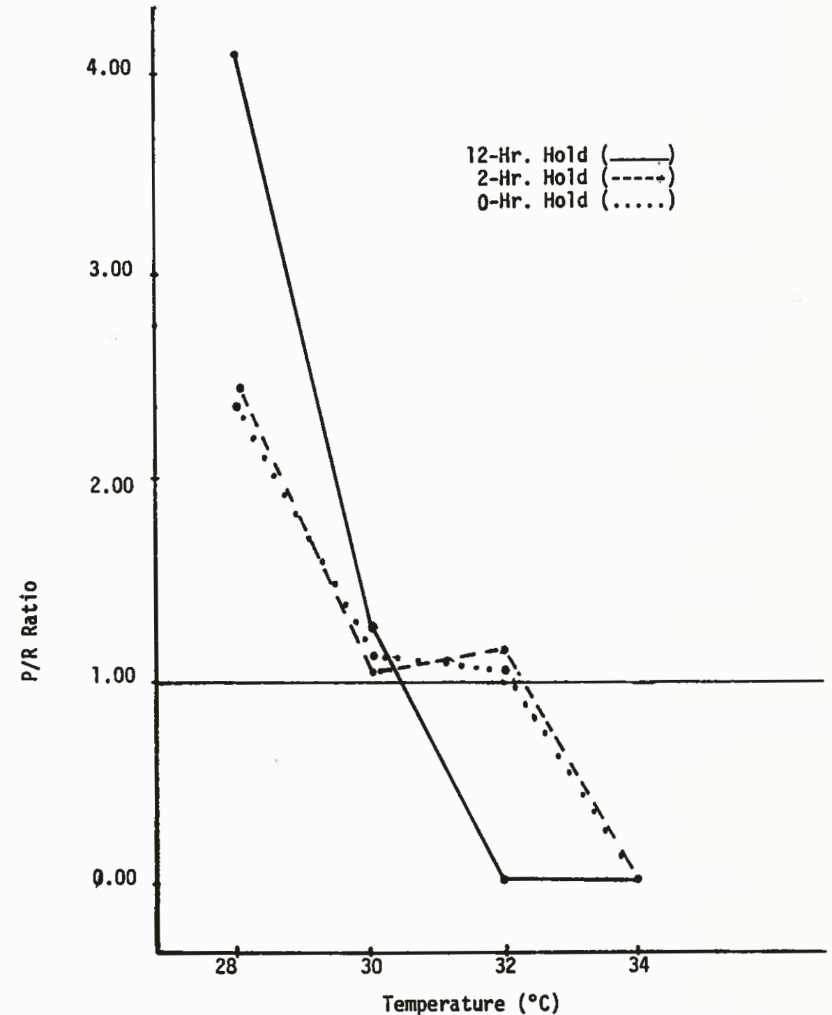
Fig. 2. Net photosynthesis/respiration ratio at four different temperatures obtained in the three experiments.
