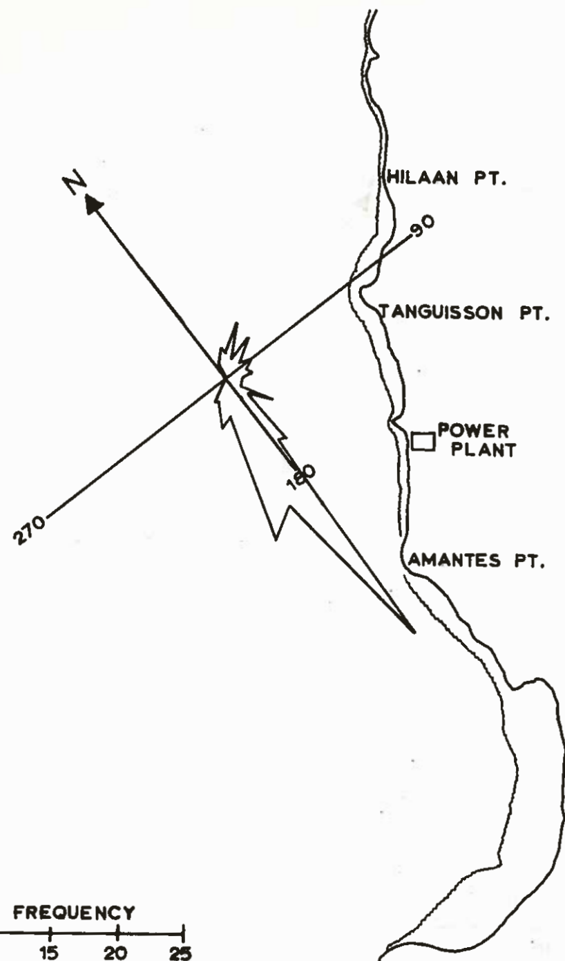
Figure 8. Mean frequency diagram for current direction at 10 to 14 m (Hydroproducts meter).
