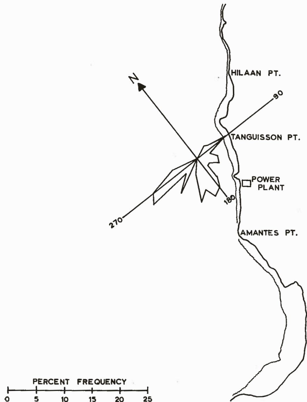
Figure 10. Mean frequency diagram for current direction at 30 m (Hydroproducts meter).
