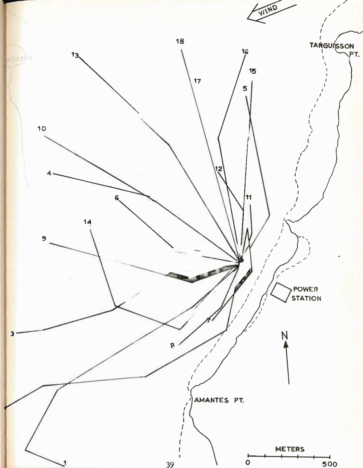
Figure 15. One meter drift cross casts. The drift cast numbers are as follow:
