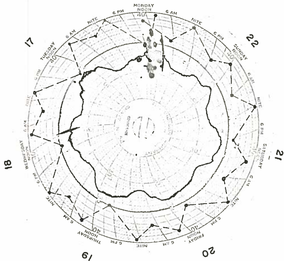
Figure 14. Sample temperature recordings for the outfall lagoon of the Piti Power Plant (Sta. 26, Fig. 13). The dashed lines indicate tidal fluctuations and were drawn by hand. The MLLW datum for the tidal records is also indicated.
