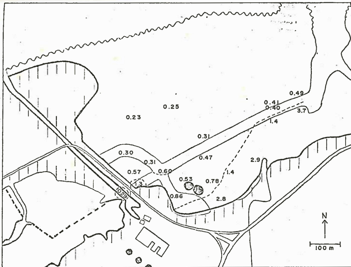
Figure 11. Turbidity values (Jackson Turbidity Units) in West Piti Bay on 24 April 1974 after removal of the construction dike. The blackened areas on the reef flat represent two large silt piles left after dredging of the adjacent swimming area.
