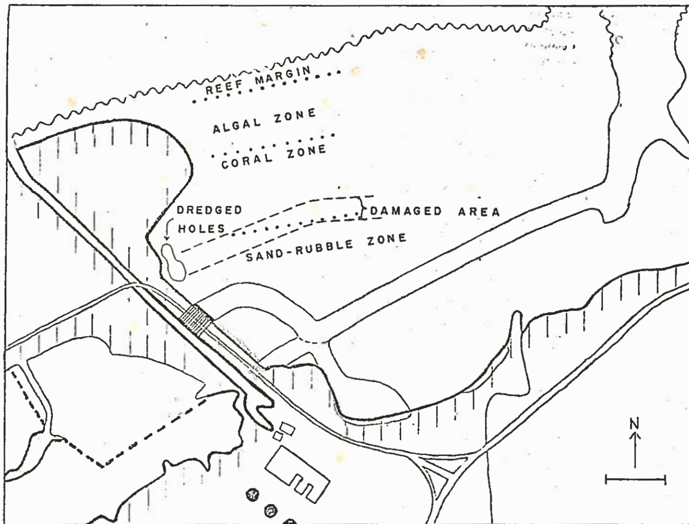
Figure 12. Reef zones, bulldozer-damaged area, and other features referred to in the text. The parallel lines across the causeway at the end of the curved part of the channel represent the construction area for a new submerged passage through the causeway. The stippling next to the causeway shoreline represents a silt plume caused by this construction.
