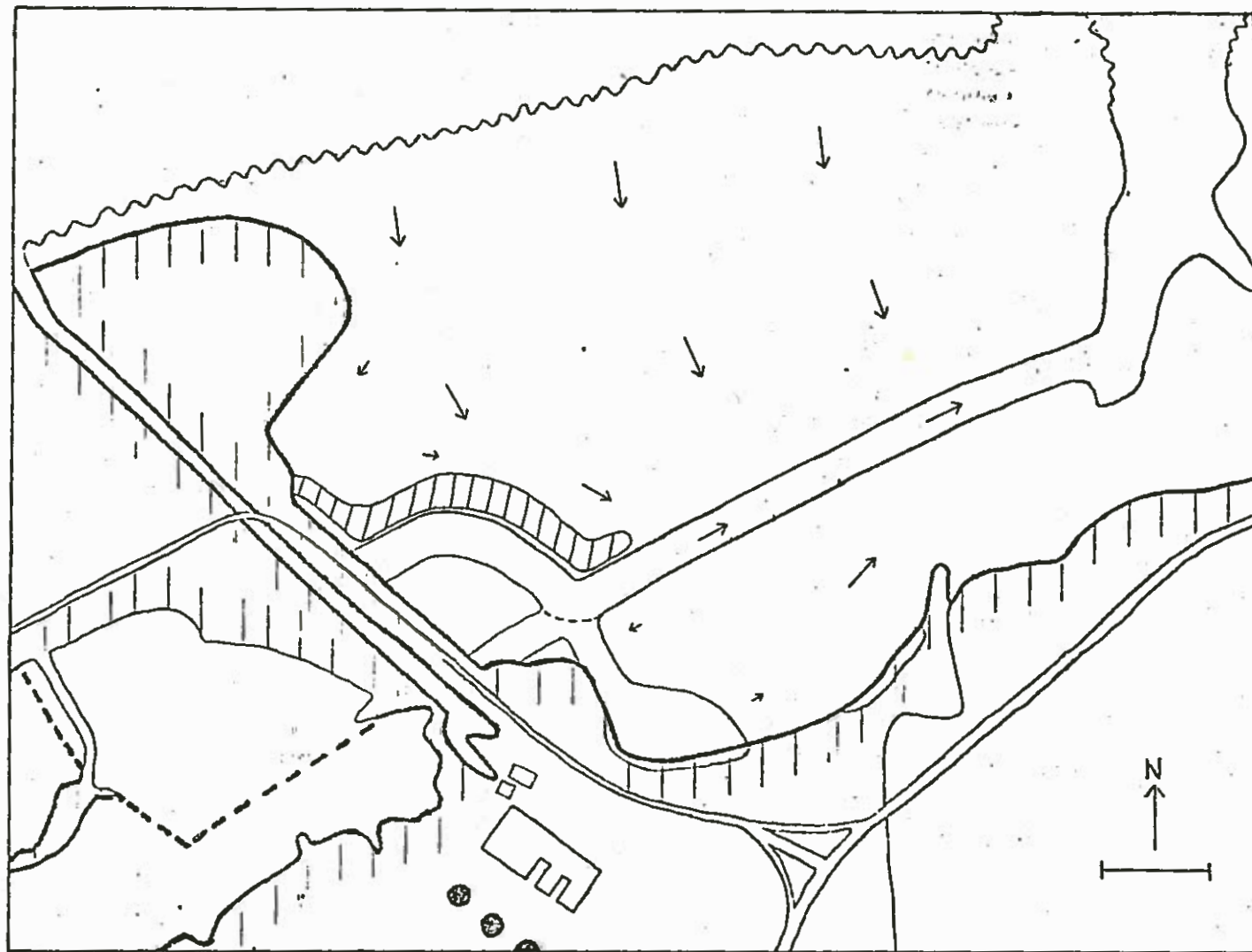
Figure 4. General current patterns in West Pitt Bay with the curved portion of the construction dike in place. Note the lack of culverts through the dike. The length of the arrows is roughly proportional to the flow velocity.
