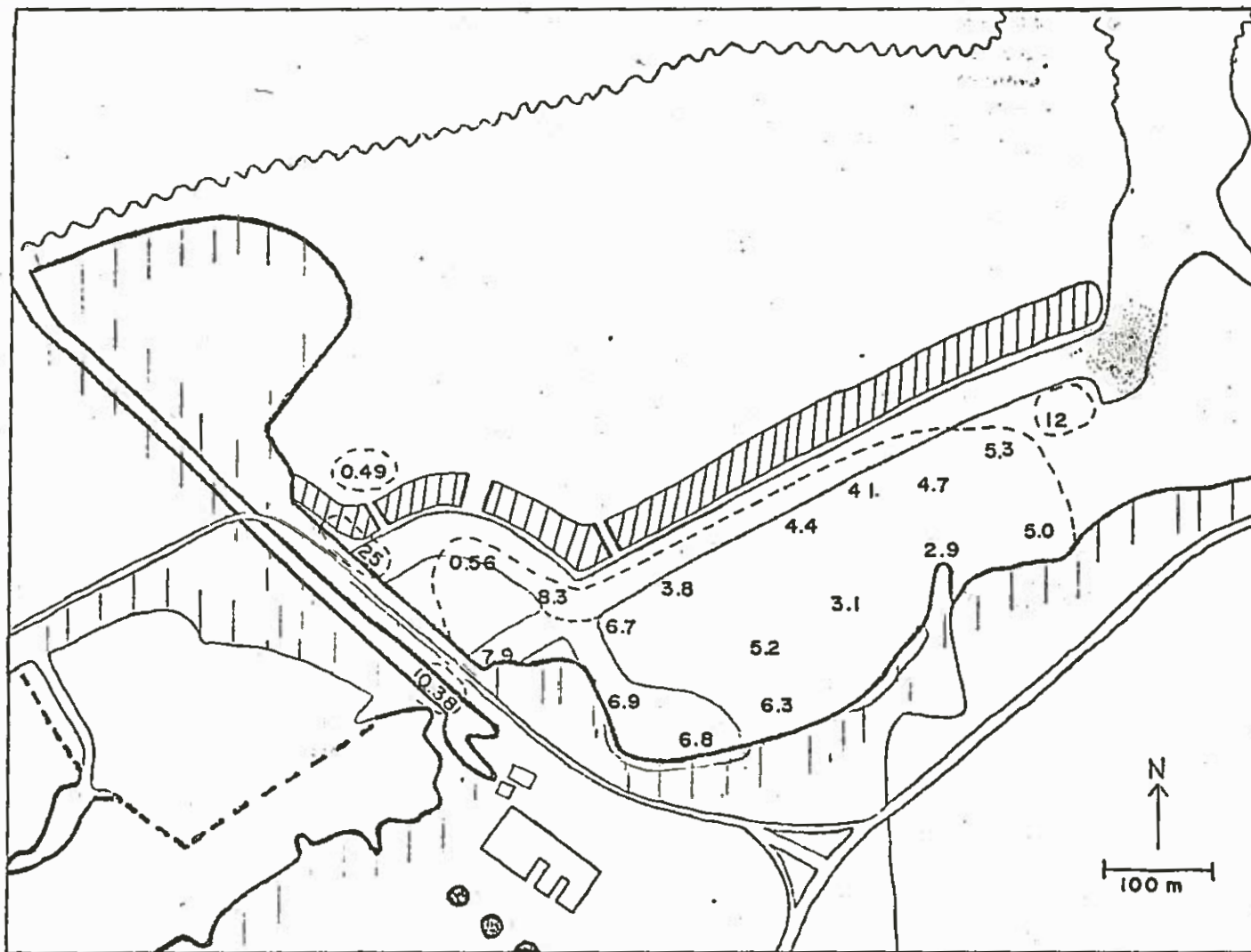
Figure 10. Turbidity values (Jackson Turbidity Units) in West Piti Bay on 14 February 1973 with the construction dike at its maximum extent. The stippling in the deeper part of the bay represents a visually obvious region of highly turbid water,
