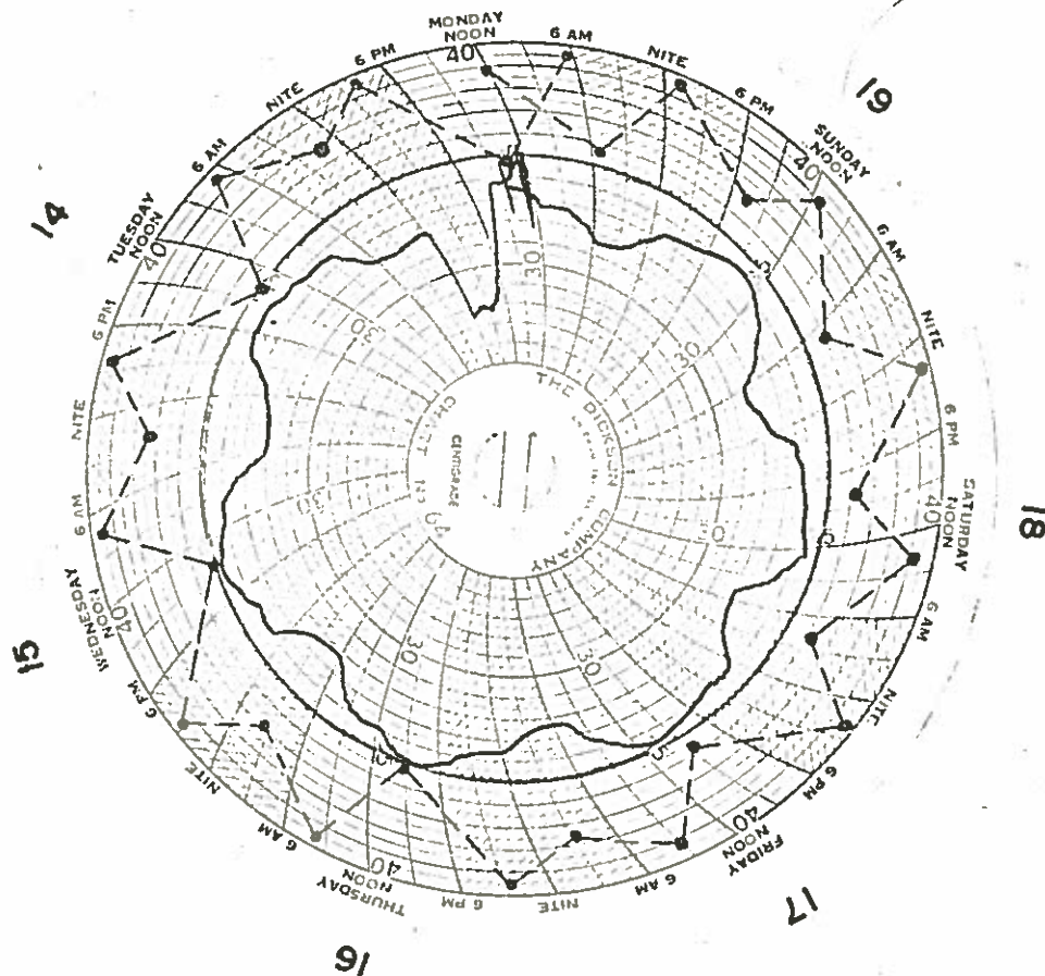
Figure 14. Sample temperature recordings for the outfall lagoon of the Piti Power Plant (Sta. 26, Fig. 13). The dashed lines indicate tidal fluctuations and were drawn by hand. The MLLW datum for the tidal records is also indicated.
