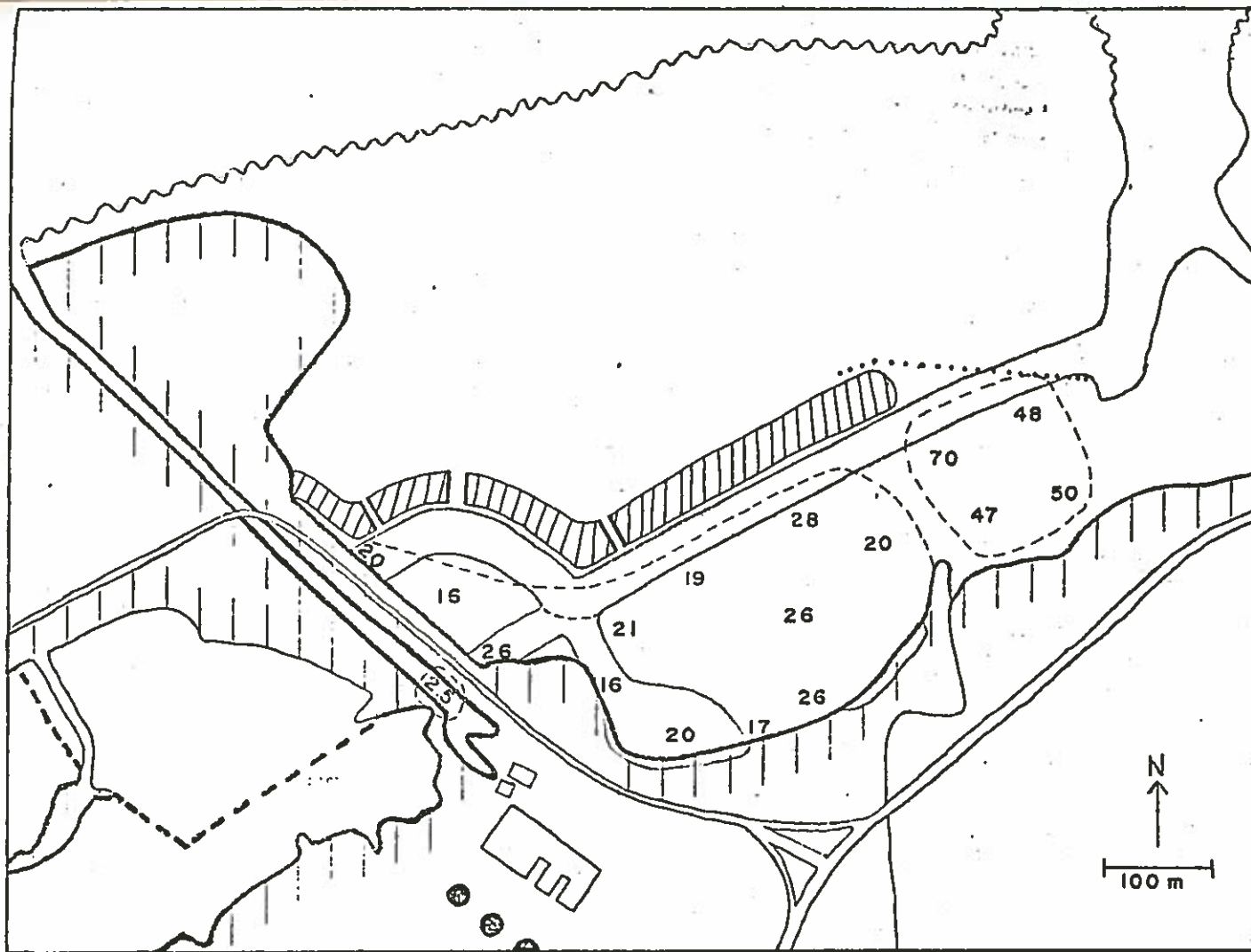
Figure 9. Turbidity values (Jackson Turbidity Units) in West Piti Bay on 5 February 1973. The dotted line extending eastward from the end of the construction dike represents the boundary between visually turbid and clear water.
