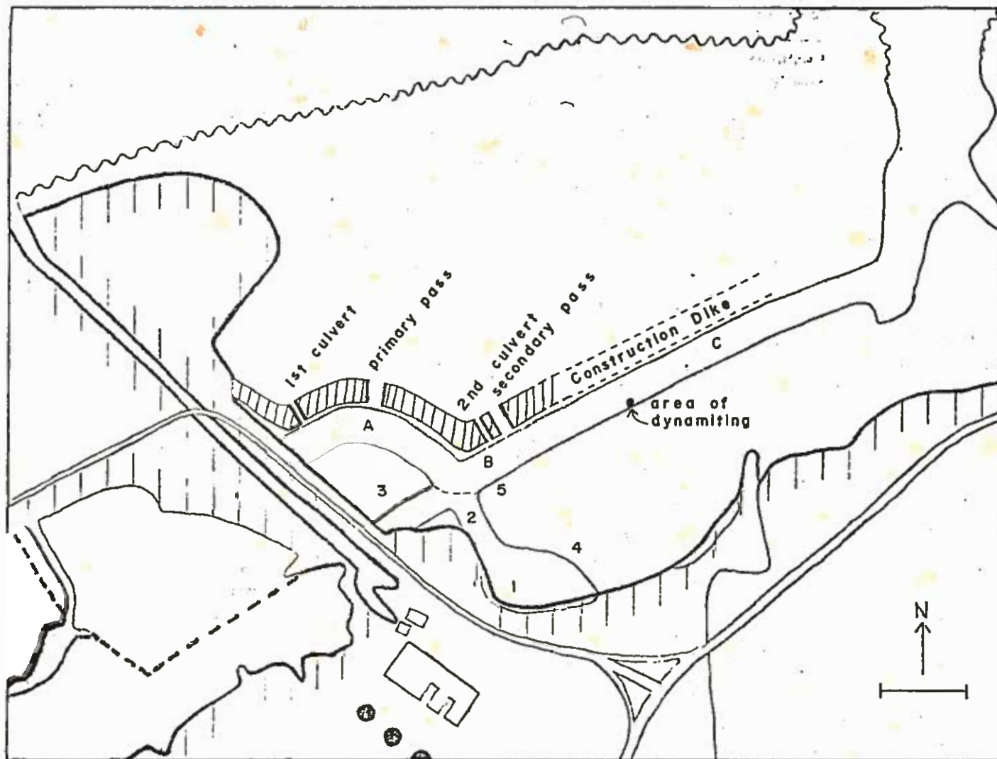
Figure 6. Location of features and sampling stations referred to in the text and in Tables 3 and 4. The letters indicate stations for flow velocities and volume transports in Tepungan Channel after dredging was completed. The numbers indicate turbidity sampling stations.
