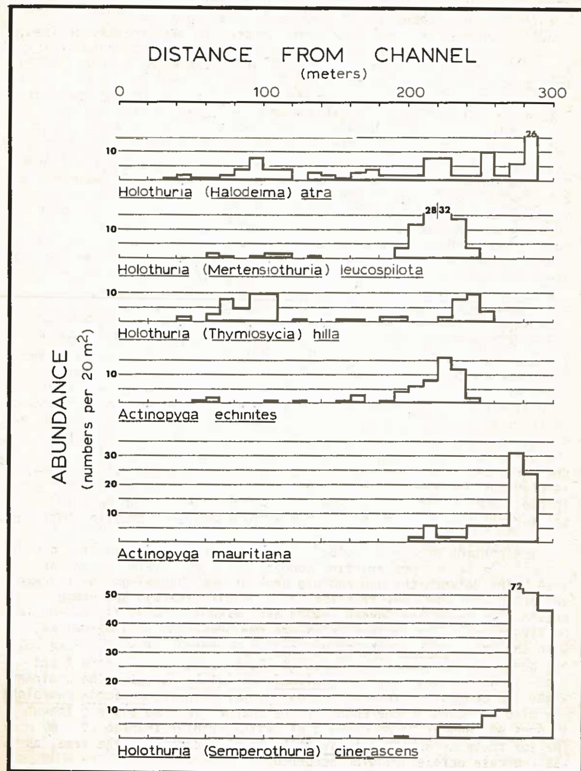
Figure 22. Abundance of major holothurian species across the reef flat in West Piti Bay.
