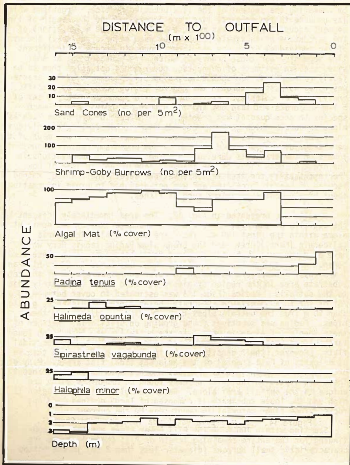
Figure 12. Abundance of major benthic features and organisms in Piti Channel.
