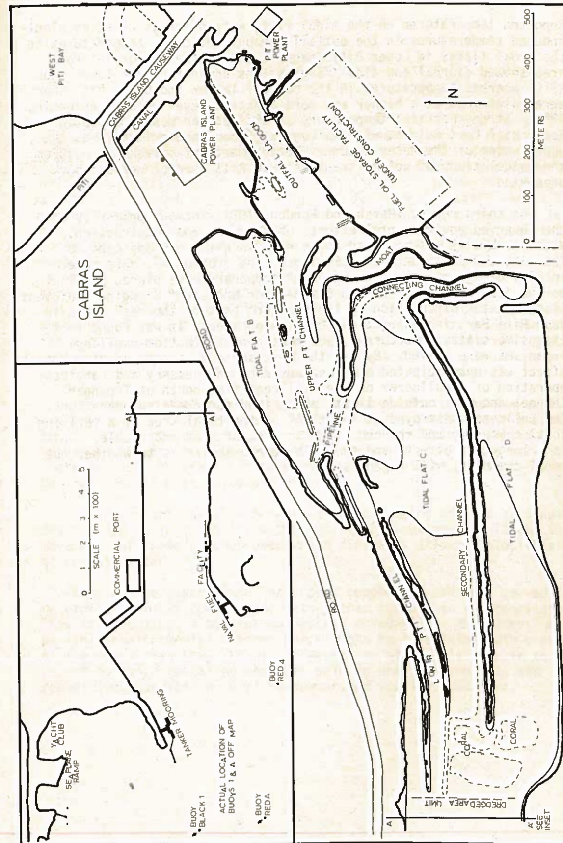
Figure 4. Major features of the area affected by the effluents of the Piti and Cabras Power Plants. Inputs of water from power plant outfalls are indicated by arrows.
