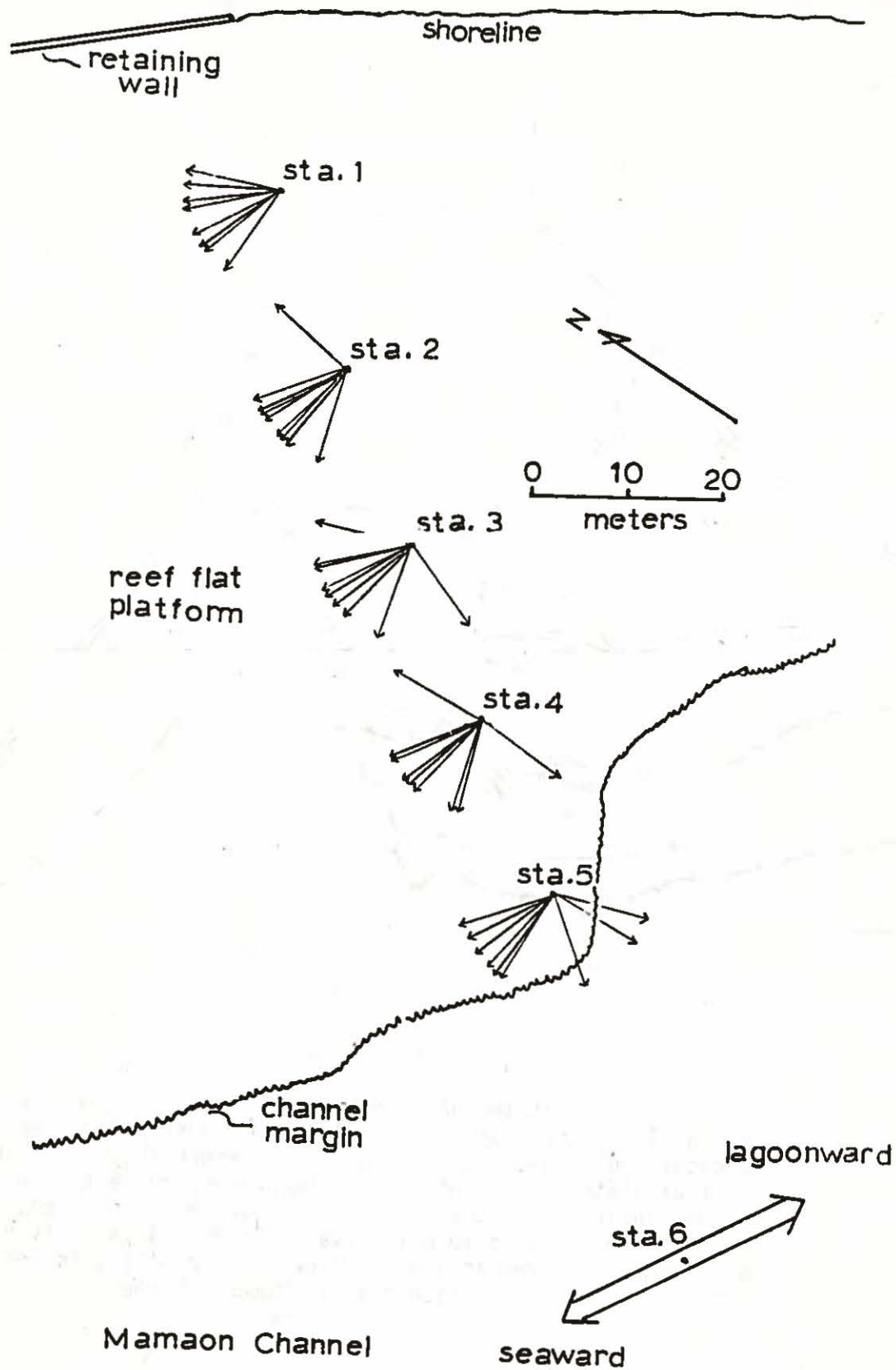
Figure 16. Current patterns on the reef-flat platform and in adjacent Mamaon Channel. Stations 1-5 are 20 meters apart. Station 6 is located in the middle of Mamaon Channel. See Figure 19 for the location of the study (Station C-3) in relation to the whole of Cocos Lagoon.
