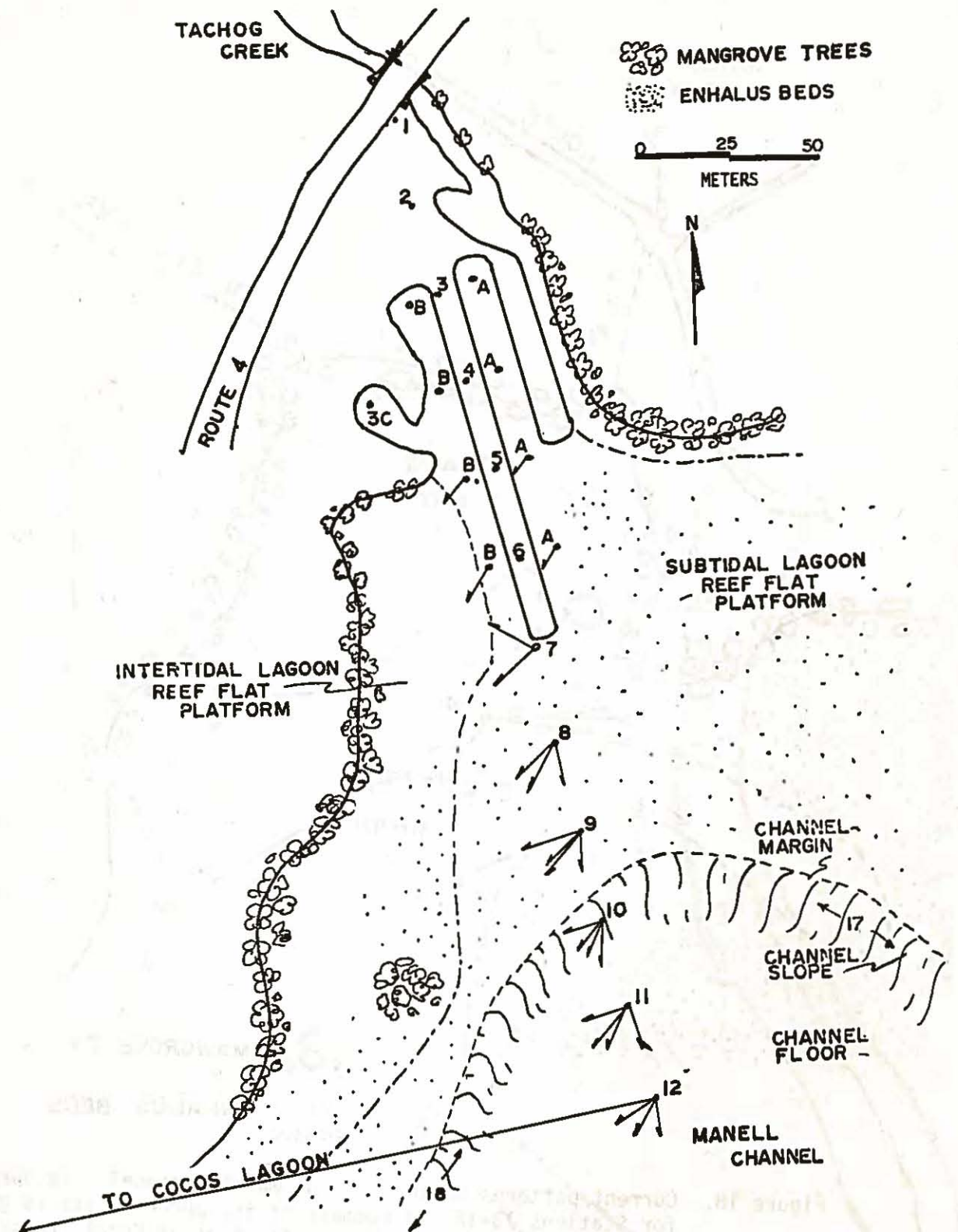
Figure 17. Current patterns on the fringing reef-flat platform (Biotope I, Facies E) for Stations 1-12. A summary of the current data is given in Table 9. Stations 17 and 18 are the locations of Coral Transects 30 and 31 respectively.
