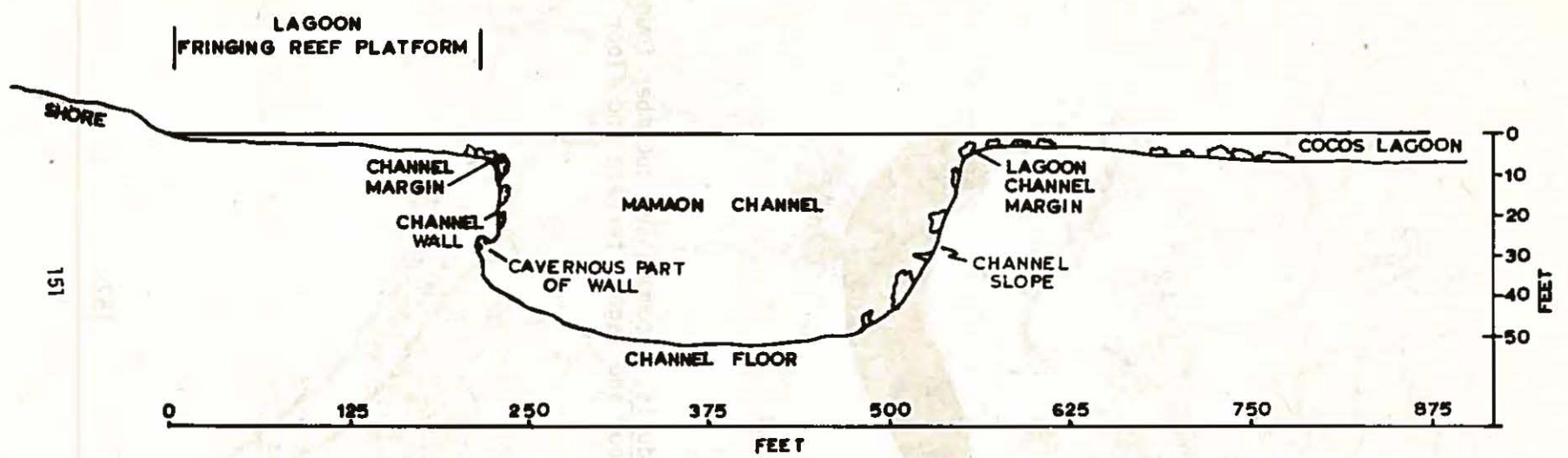
Figure 37. Vertical profile (Transect B) through Mamaon Channel showing the various facies of Biotope II. Facies A= channel margin, Facies B= channel slope, Facies C= channel wall, Facies D= cavernous parts of the channel slopes or walls, and Facies E= channel floor. See Figure 7 for the location of Transect B.
