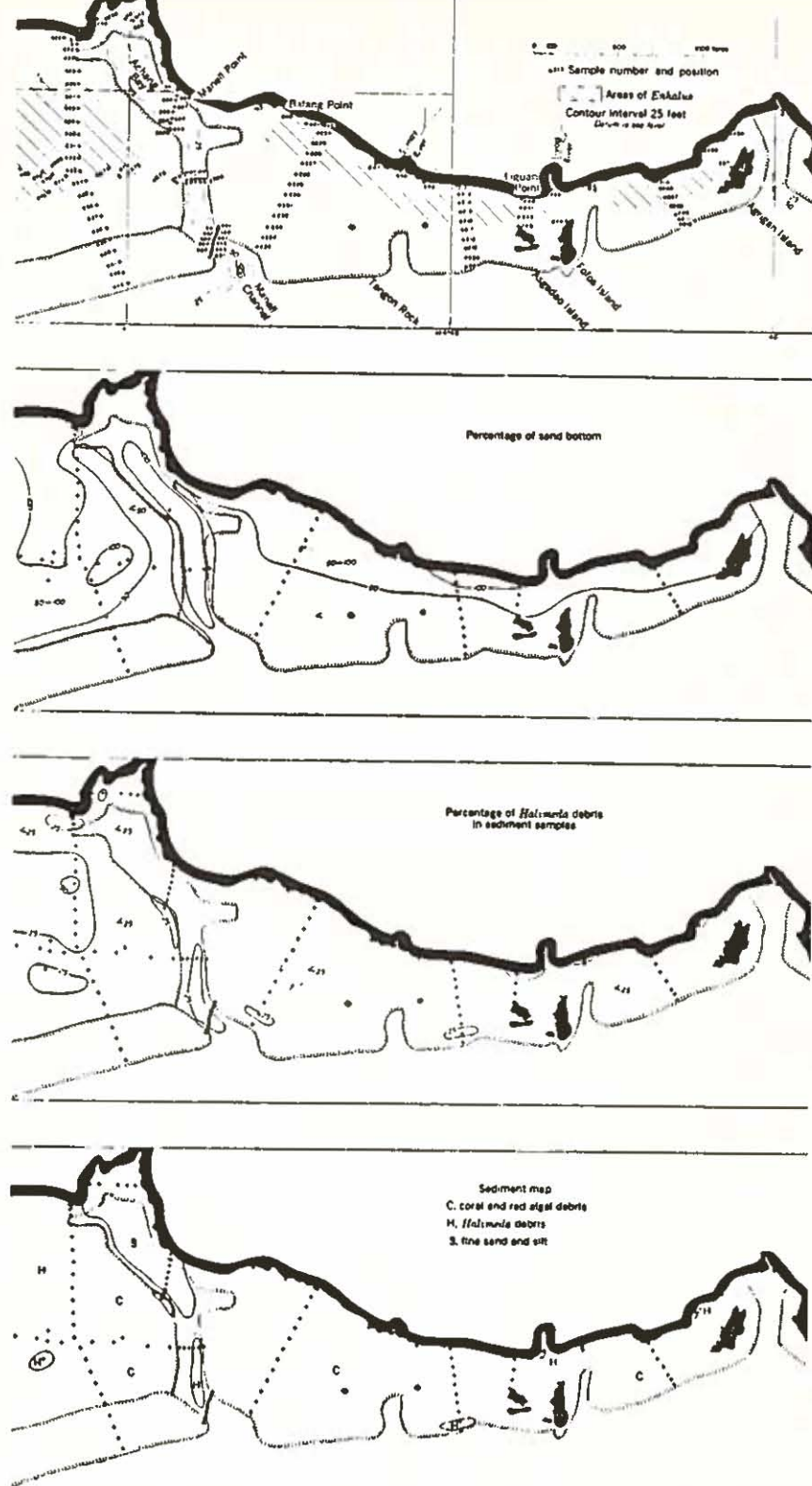
Figure 10. Eastern end of Cocos Lagoon, Manell Channel, and Achang reef flat platform showing topography and surface composition. Figure from Emery (1962).
