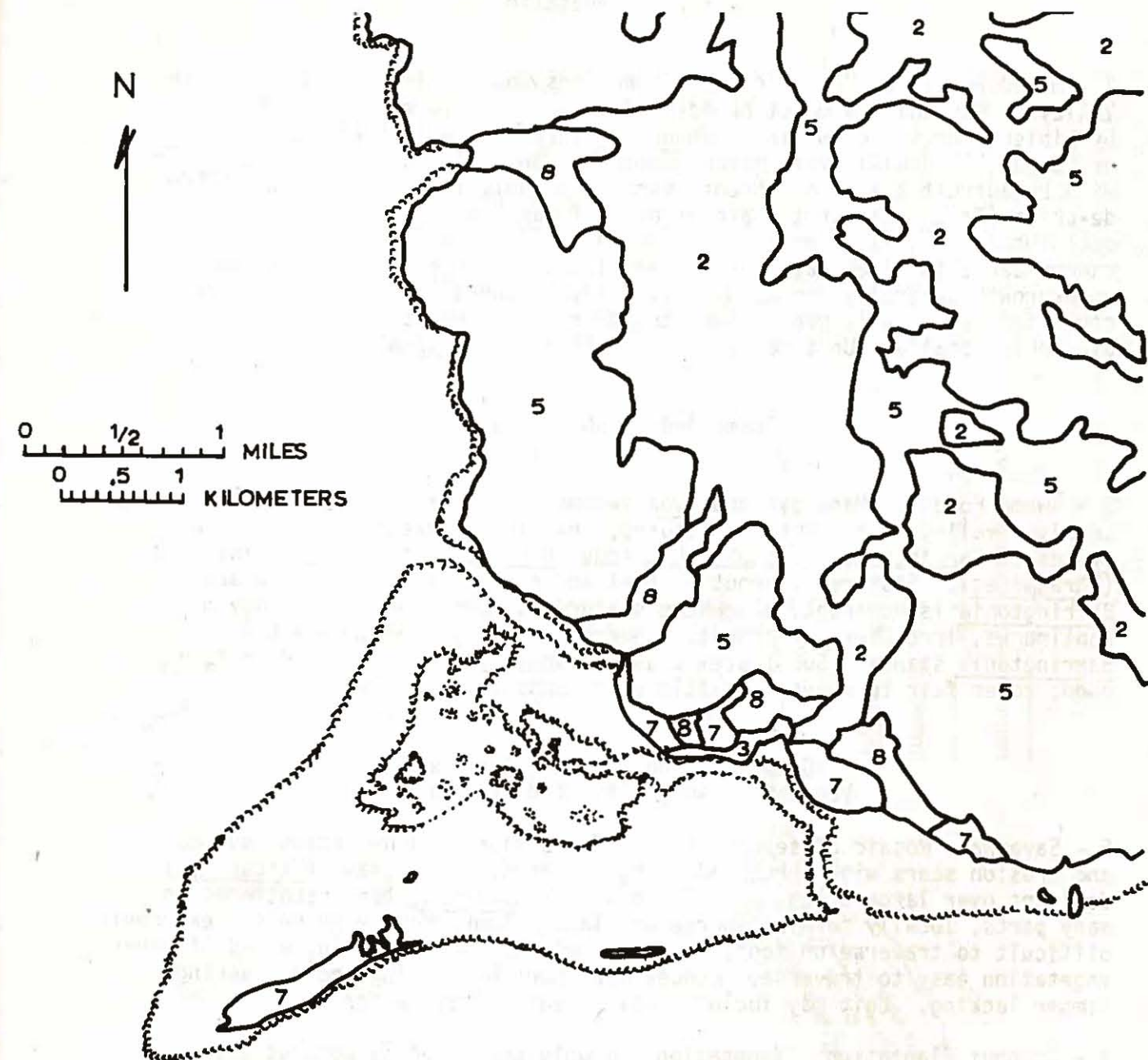
Figure 6. Vegetation map for the Cocos Lagoon study area. A legend explanation for the numbered vegetation units 2, 3, 5, 7, and 8 is given on the following page.
