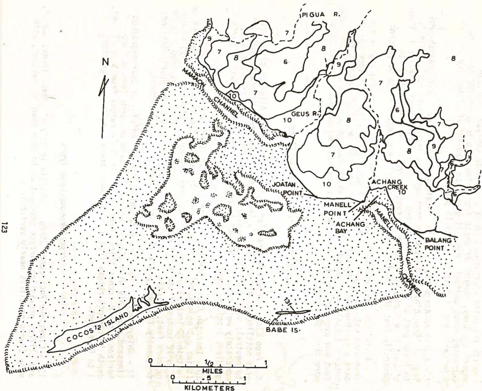
Figure 5. Soil map for the Cocos Lagoon study area. A soil unit explanation legend is given on the following page. Fringing reef-flat and shallow lagoon shelves are stippled.
