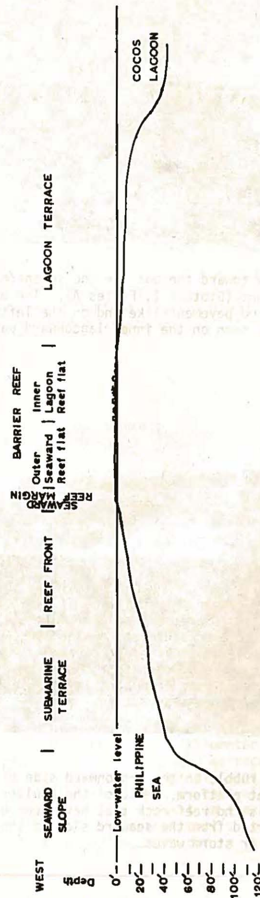
Figure 23. Vertical profile (A) of the northern barrier reef and lagoon. See Figure 7 for location of the transect.
