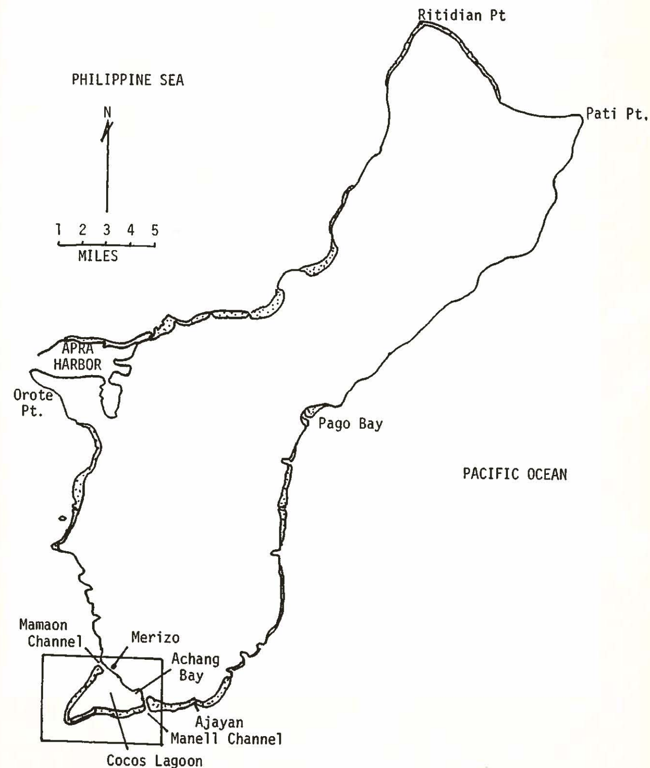
Figure 1. Map of Guam showing the location of the Cocos Lagoon Study area.
