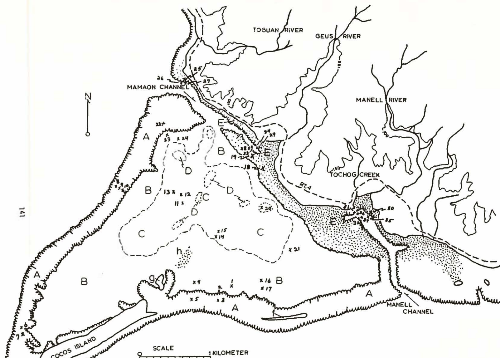
Figure 21. Map showing the distribution of Facies A-E for Biotope I. A= Biotope IA, B= Biotope IB, C= Biotope IC, D= Biotope ID, and E= Biotope IE. Mamaon and Manell Channels constitute Biotope II. See Figure 37 for the distribution of Facies A-E for Biotope II. Cocos Island= Biotope IIIA, Babe Island (f)= Biotope IIIB, and the landward border of Cocos Lagoon= Biotope IIIC. Sand islet= (g) and (h)= the location of a Halodule uninervis sea grass bed. The stippled area along the landward border of the lagoon shows the distribution of the Enhalus acoroides sea grass beds. Numbers 1-37 show the location of the coral transects (Table 13).
