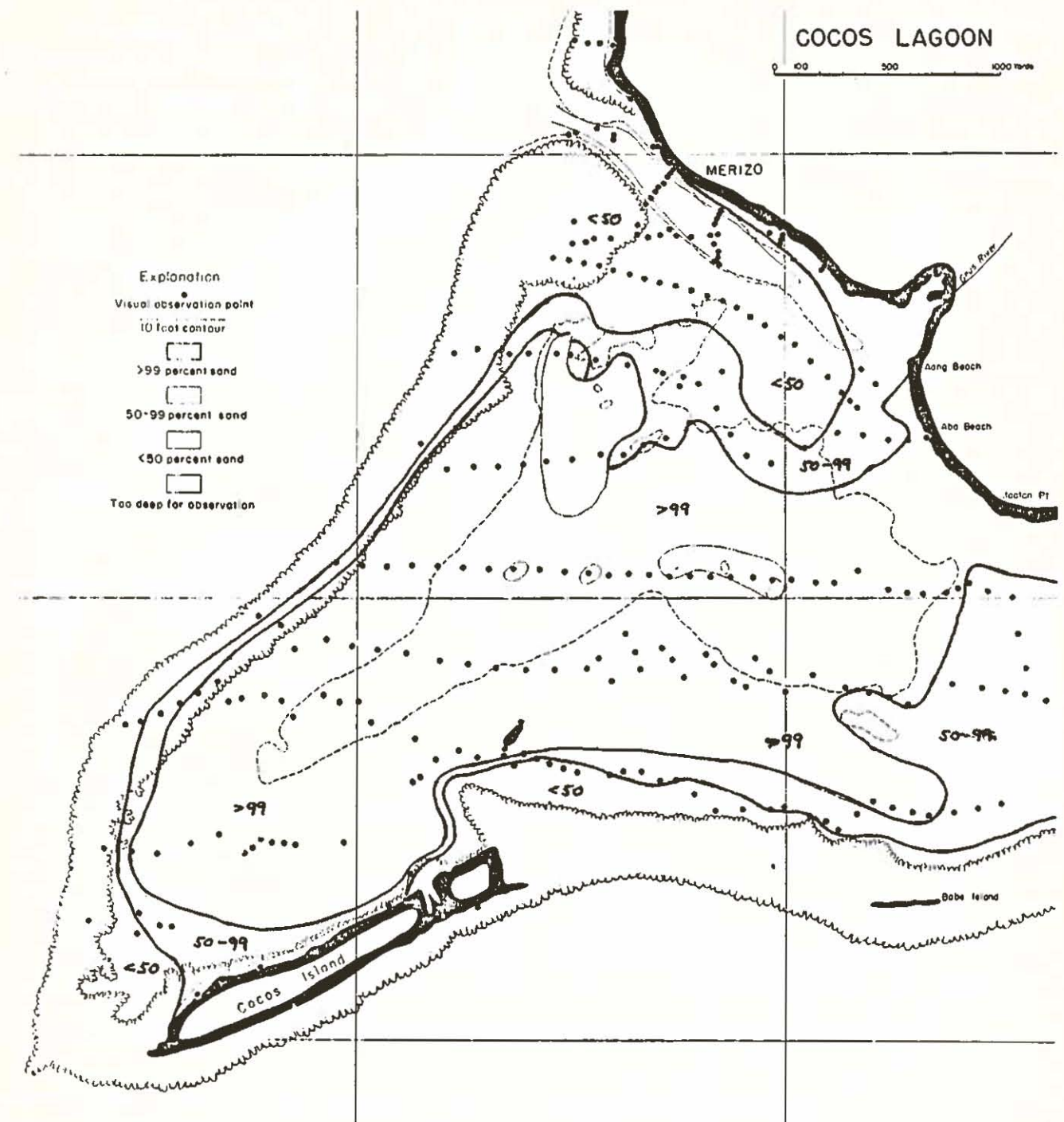
Figure 11. Percentage of sand and coral bottom on the floor of Cocos Lagoon as determined by visual observation, Figure from Emery (1962).
