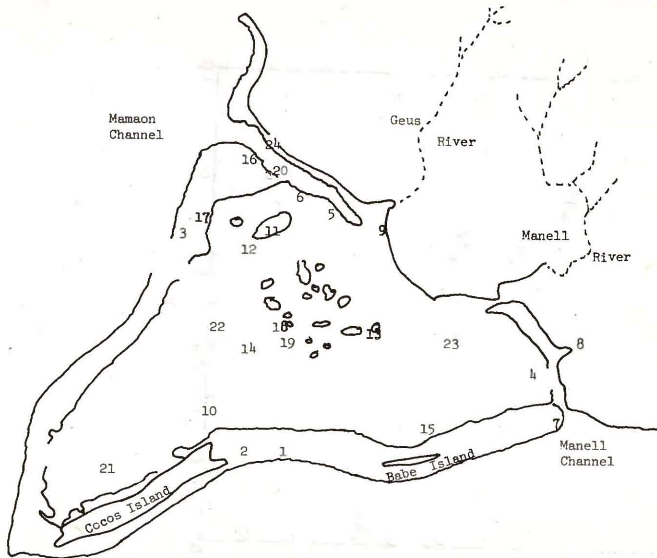
Figure 49. Location of the 24 algal stations.
