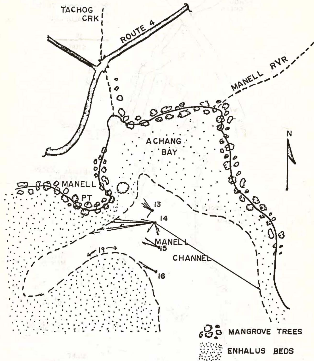
Figure 18. Current patterns at the head of Manell Channel (Biotope II) for Stations 13-16. A summary of the current data is given in Table 9. Station 19 is the location of Coral Transect No. 32.
