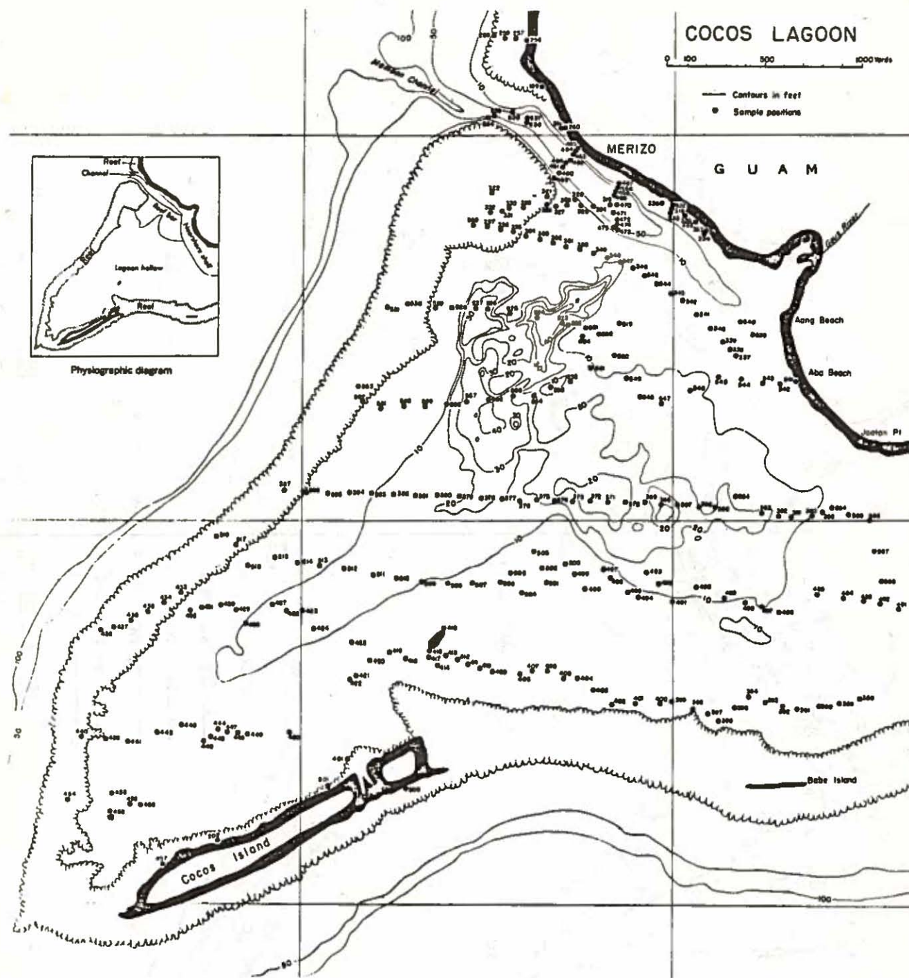
Figure 8. Topography map of Cocos Lagoon. Inset shows the location of the physiographic units. Map from Emery (1962),
