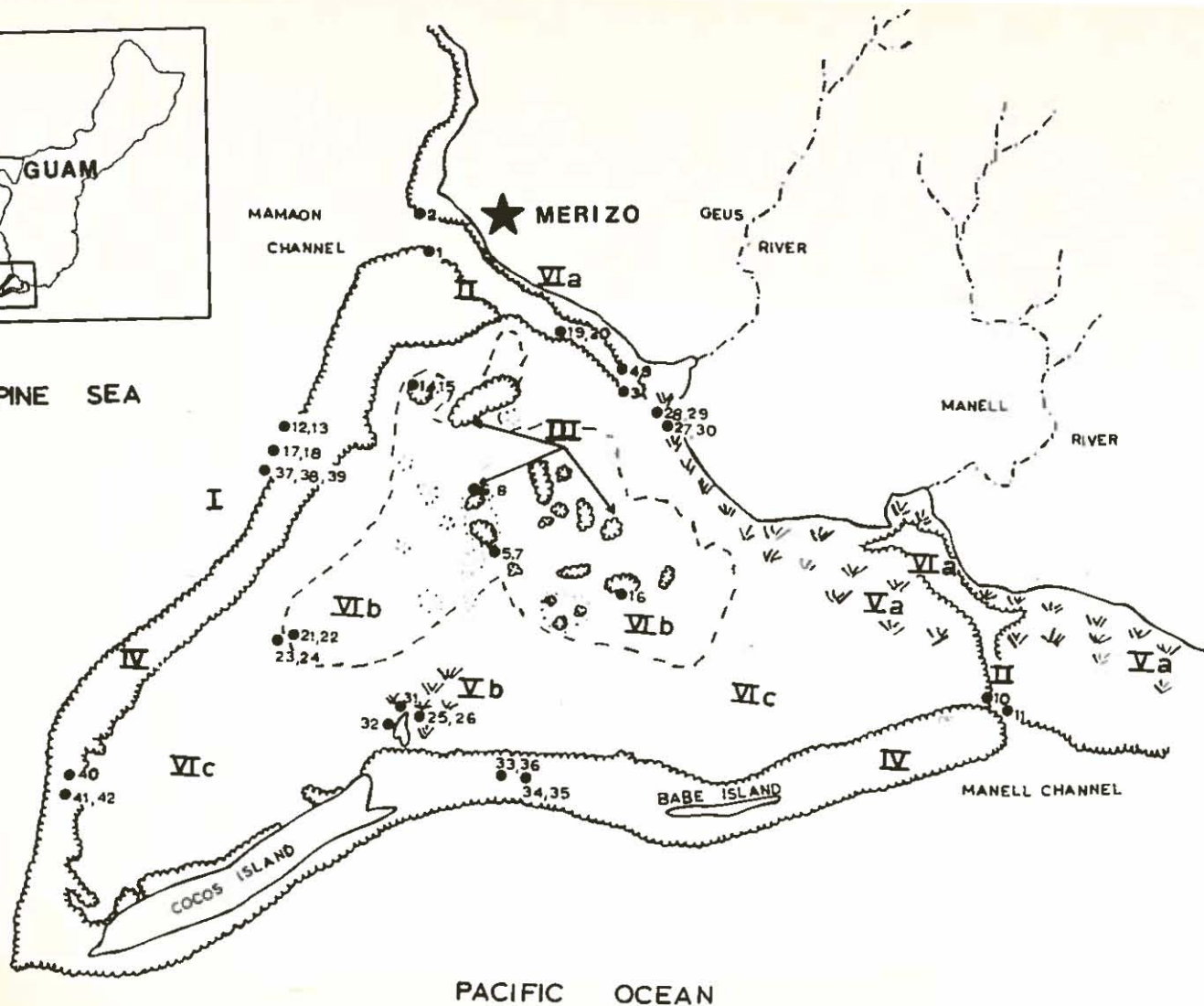
Figure 47. Map of Cocos Lagoon study area. The black spots show the approximate locations of the transect stations, the arabic numerals indicate the transect numbers, and the dashed line is the boundary between the lagoon terrace and the lagoon floor. The number of patch reefs and shoals shown is considerably less than the number that actually occurs in the lagoon. I-Biotope outside the barrier; II-Channel wall biotope; III-Lagoon patch reef biotope; IV-Barrier reef flat biotope; V-Seagrass biotope, a- Enhalus acoroides , b- Halodule uninervis ; and VI-Sand bottom biotope, a-channel bottoms, b-lagoon floor, and c-lagoon terrace.
