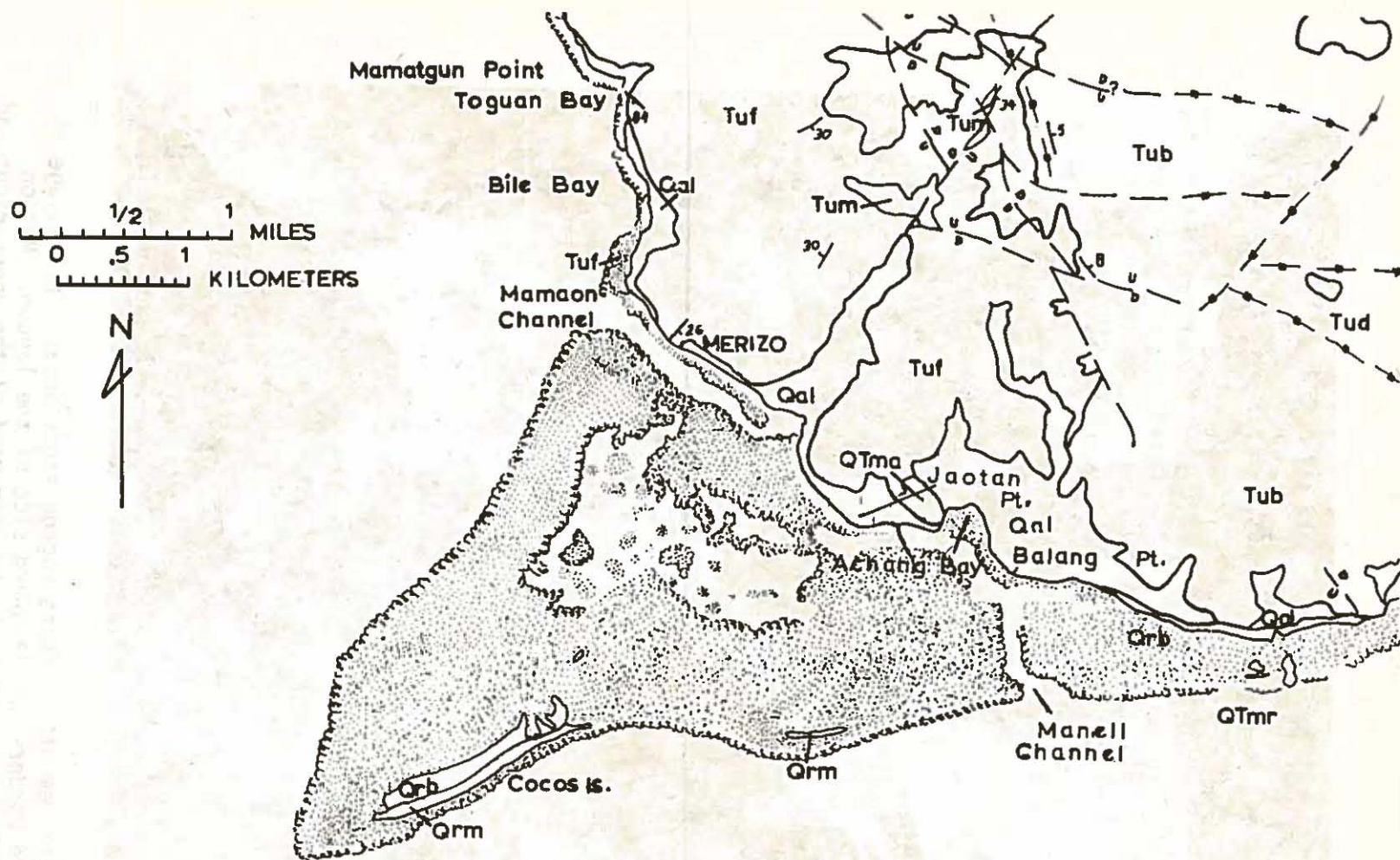
Figure 4. Geologic map for the Cocos Lagoon study area. Rock units designated are: Qal= alluvium, Orb= Beach Deposits, Qrm= Merizo Limestone, QTma= Agana Argillaceous Member of the Mariana Limestone, QTmr= Reef Facies of the Mariana Limestone, Tuf= Facpi Volcanic Member of the Umatac Formation, Tub= Bolanos Pyroclastic Member of the Umatac Formation, and Tum= Maemong Limestone Member of the Umatac Formation. Faults are shown as dashed lines where approximately known. The strike of vertical joints are shown with a (—●—●—) symbol and the strike and dip of beds are shown with a ( — 30° ) symbol.
