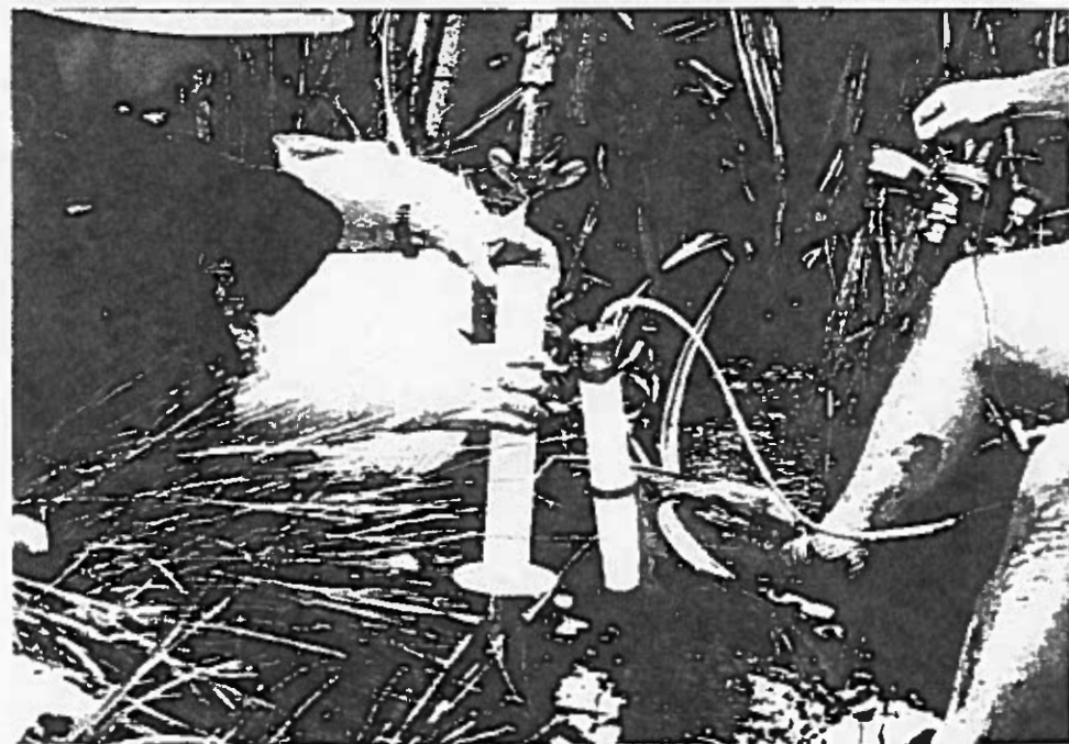
Plate 5: Water Sampling Photo 1: Lysimeter, with marking ribbon and clear tubing that introduces N_2 (tank behind legs). Graduated cylinder used to measure volume of pore waters in lysimeter.
