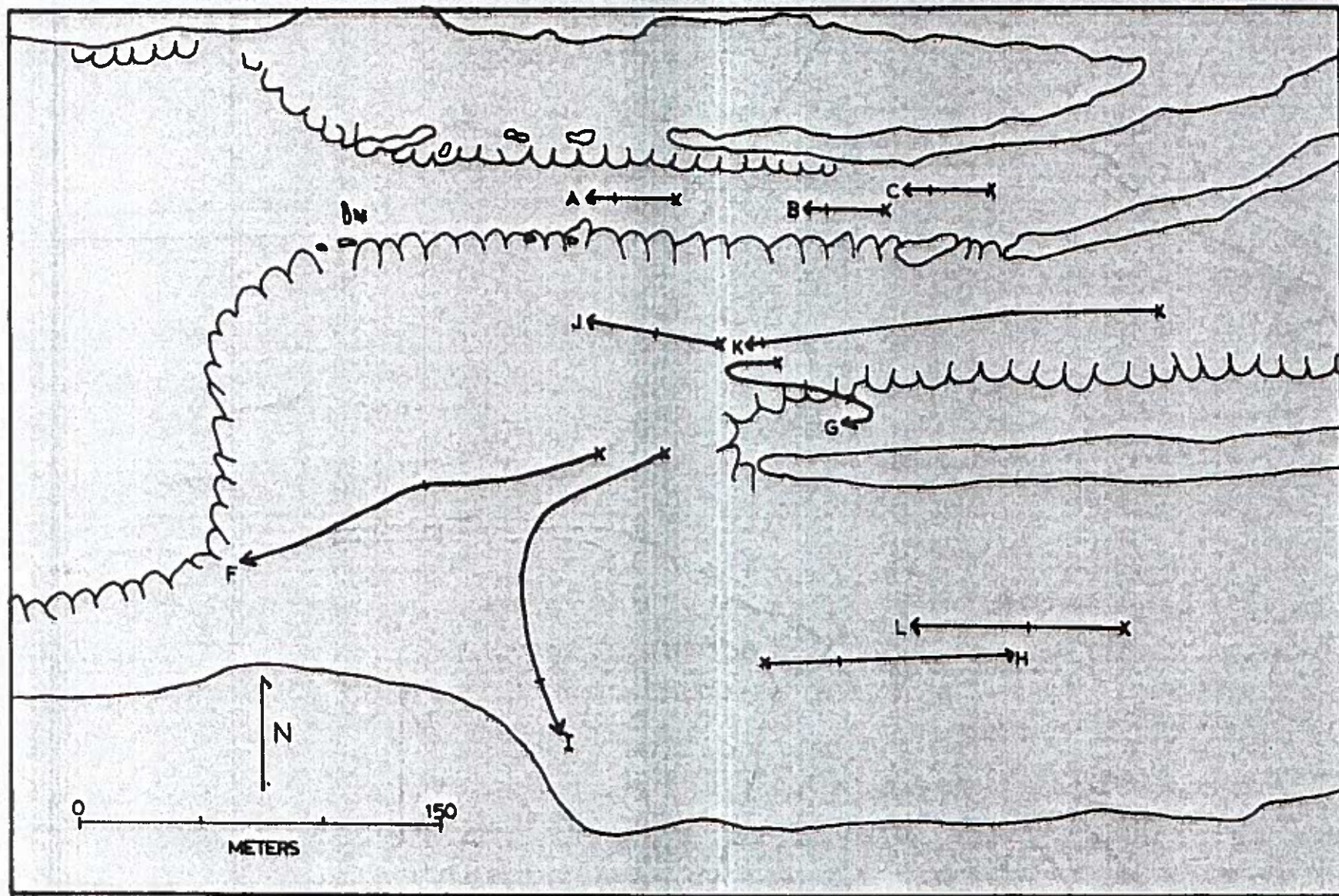
Figure 15. Dye paths in Lower Piti and Secondary Channels, Flat C and Flat D; Zone II. See Table 5 for detailed information.
