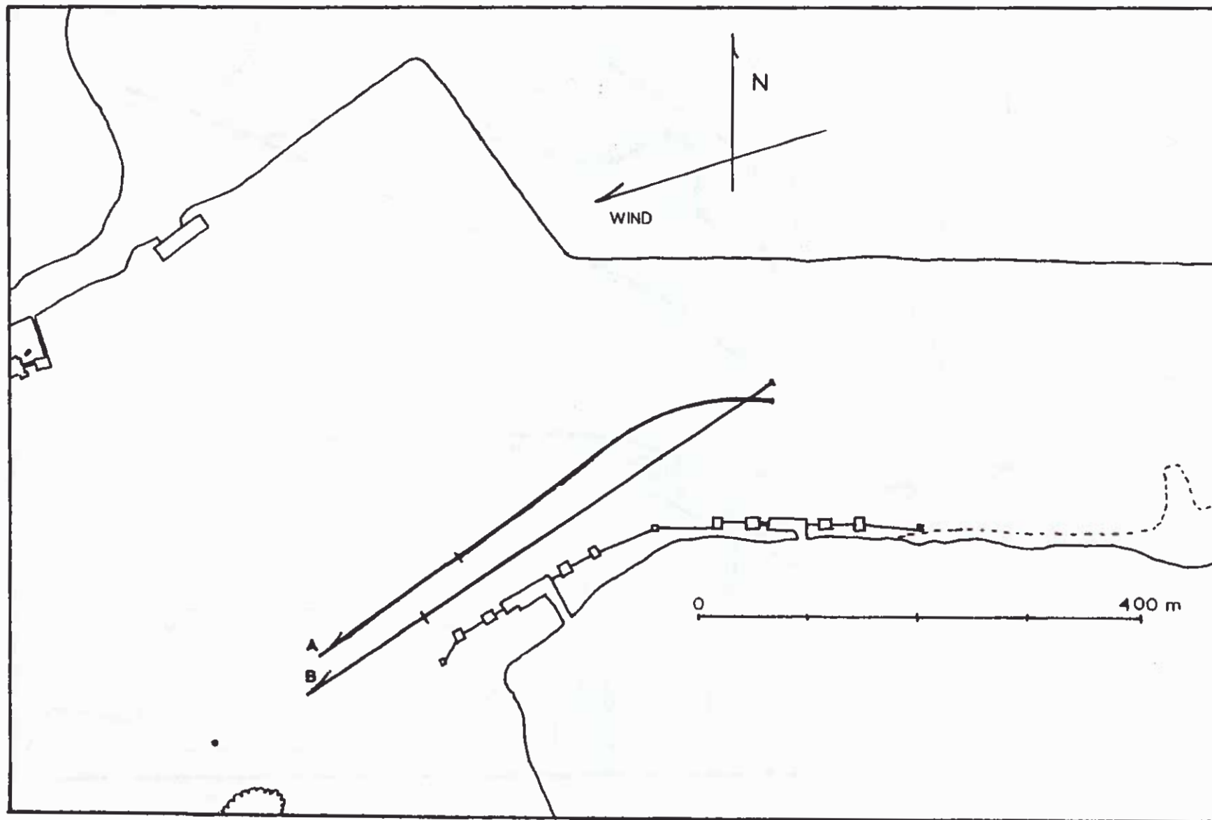
Figure 13. Inner drift drogues for 12 January, 1977, strong rising tide, 0836-1320. The wind was from the east at 3-4 knots, with gusts to 10 knots. A, 12 -m drogue; B, 6 and 7 -m drogue.
