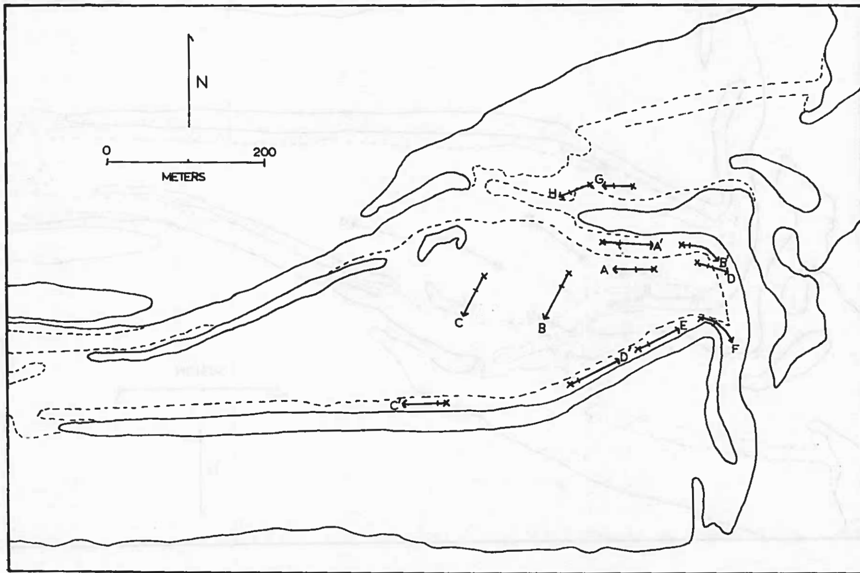
Figure 18. Dye paths of Upper Piti and Secondary Channels and Flat C; Zone III. See Table 6 for detailed information.
