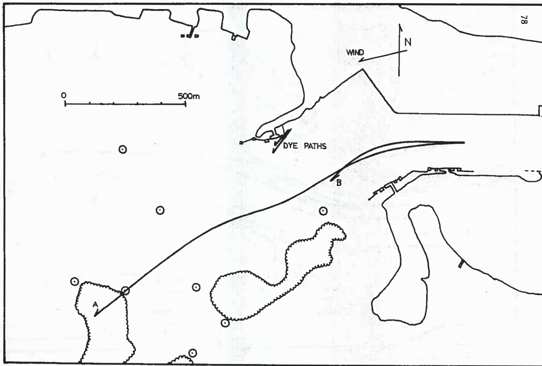
Figure 7. Inner drift drogue paths for 28 December, 1976, strong falling tide, 1530-1800. The wind was from the east and northeast at 8-12 knots. Dye paths under Gorco Pier at 1675-1730 had a velocity of .10-.08 m/sec and a direction of 245^{\circ} . A, 1-m drogue; B, 6-m drogue.
