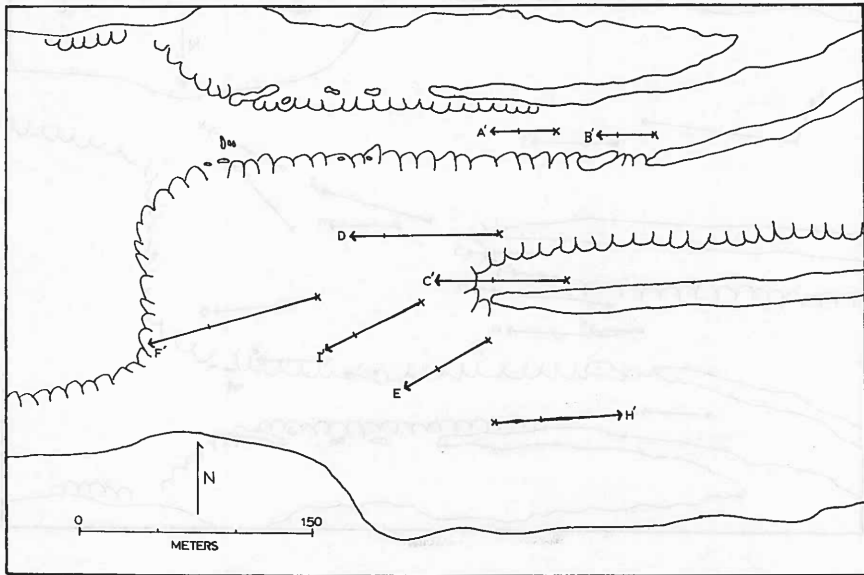
Figure 16. Dye paths in Lower Piti and Secondary Channels, Flat C and Flat D; Zone II. See Table 5 for detailed information.
