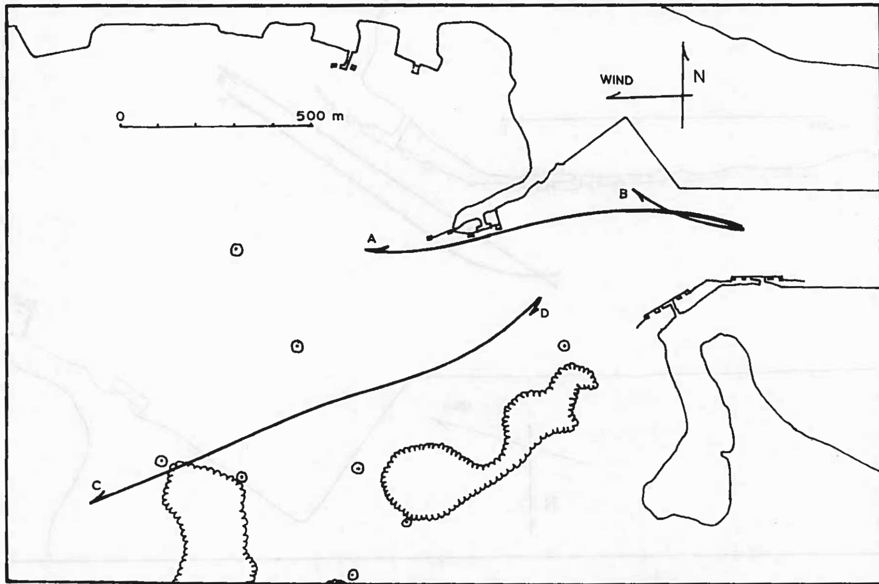
Figure 12. Inner and outer drift drogues for 4 January, 1977, weak rising tide, 1530-1730. The wind was from the east at 9-13 knots. A and C, 1 -m drogue; B, 6 -m drogue; D, sank.
