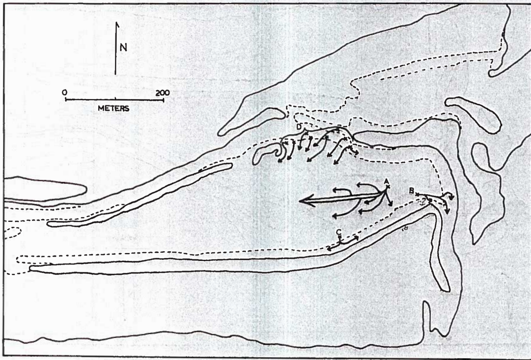
Figure 21. Qualitative study of dye patch movement for Fl at C and Upper Secondary Channel ; zone III.
