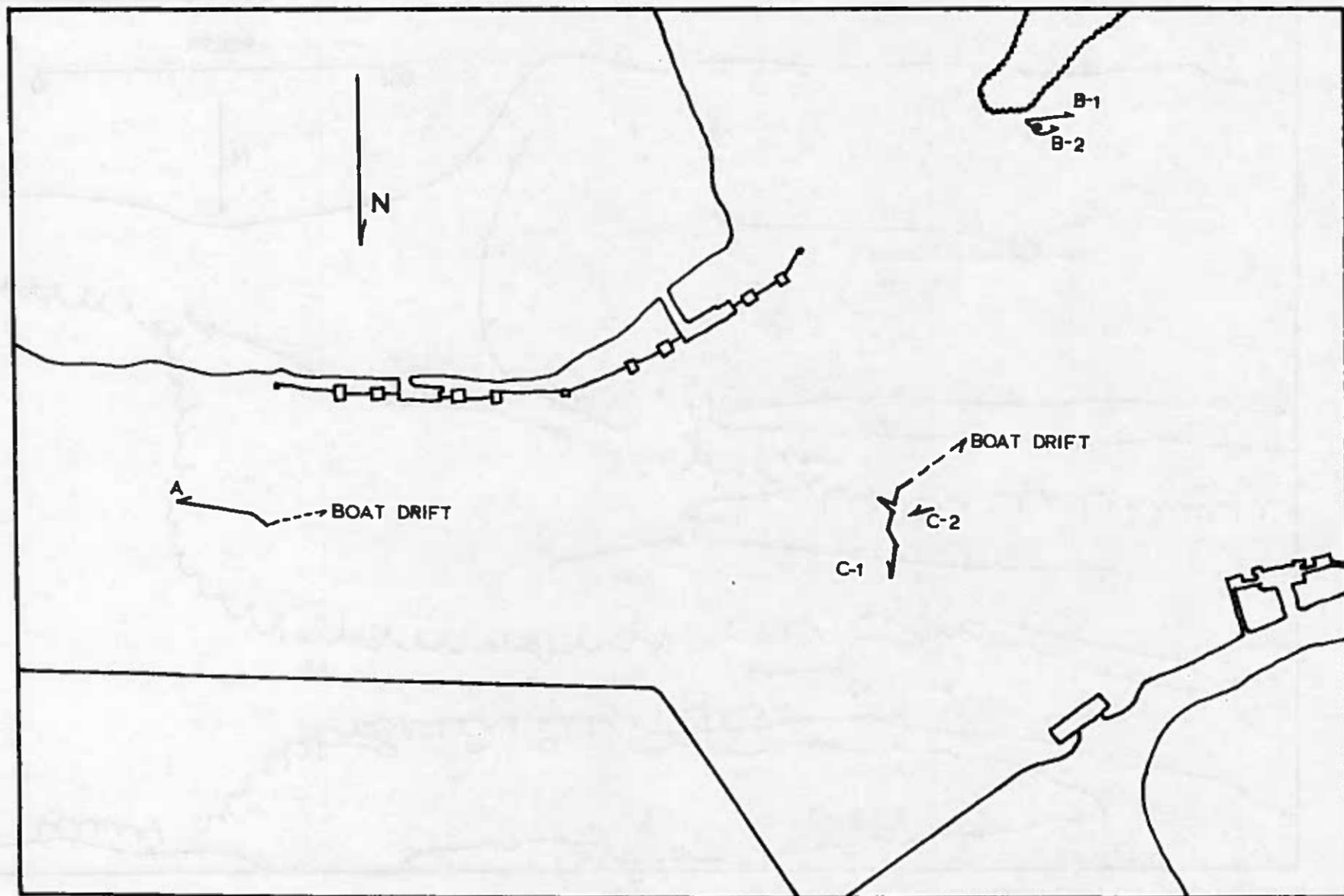
Figure 14. Subsurface dye studies 5, 10 and 12 January, 1977, strong rising and weak falling tides. See Table 3.
