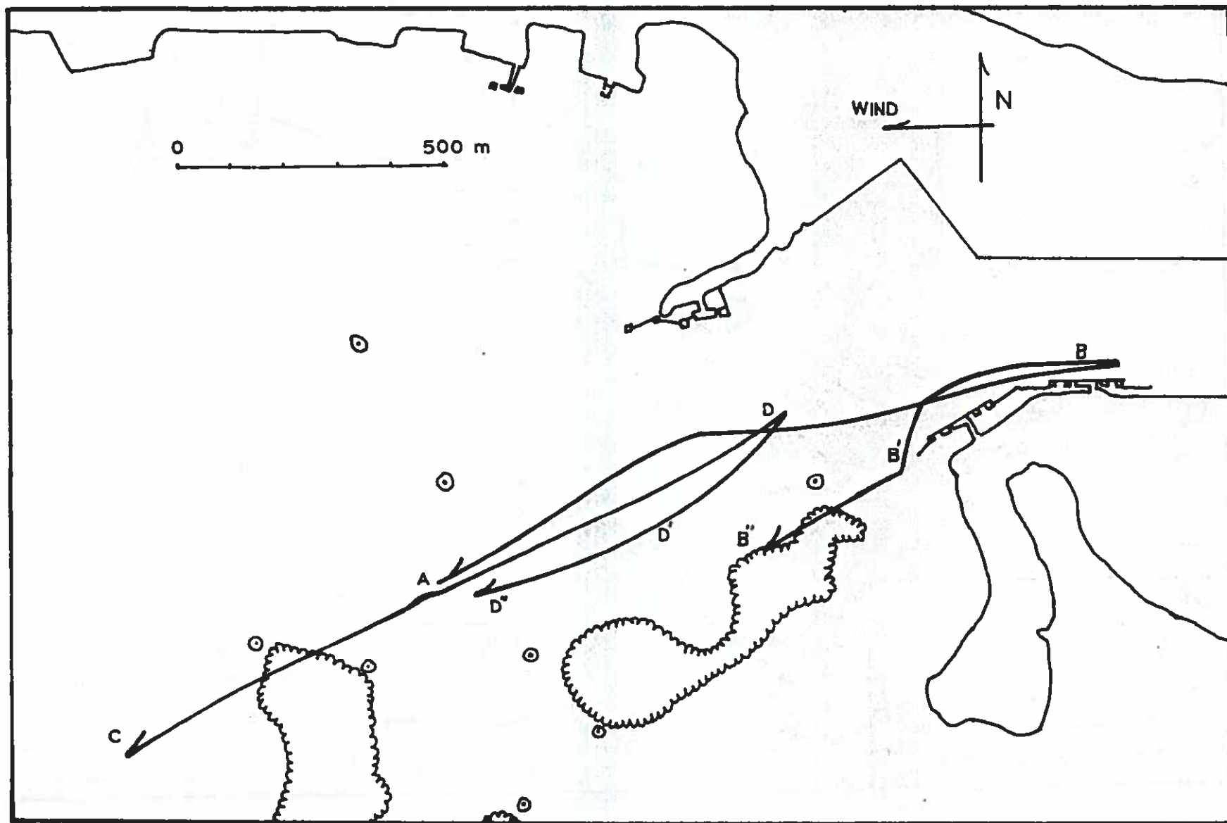
Figure 11. Inner and outer drift drogue paths for 4 January, 1977, weak rising and falling tides, 1140-1500. The wind was from the east at 5-13 knots. A and C, 1 - m drogue; B, 6 -m drogue; D, 12 -m drogue.
