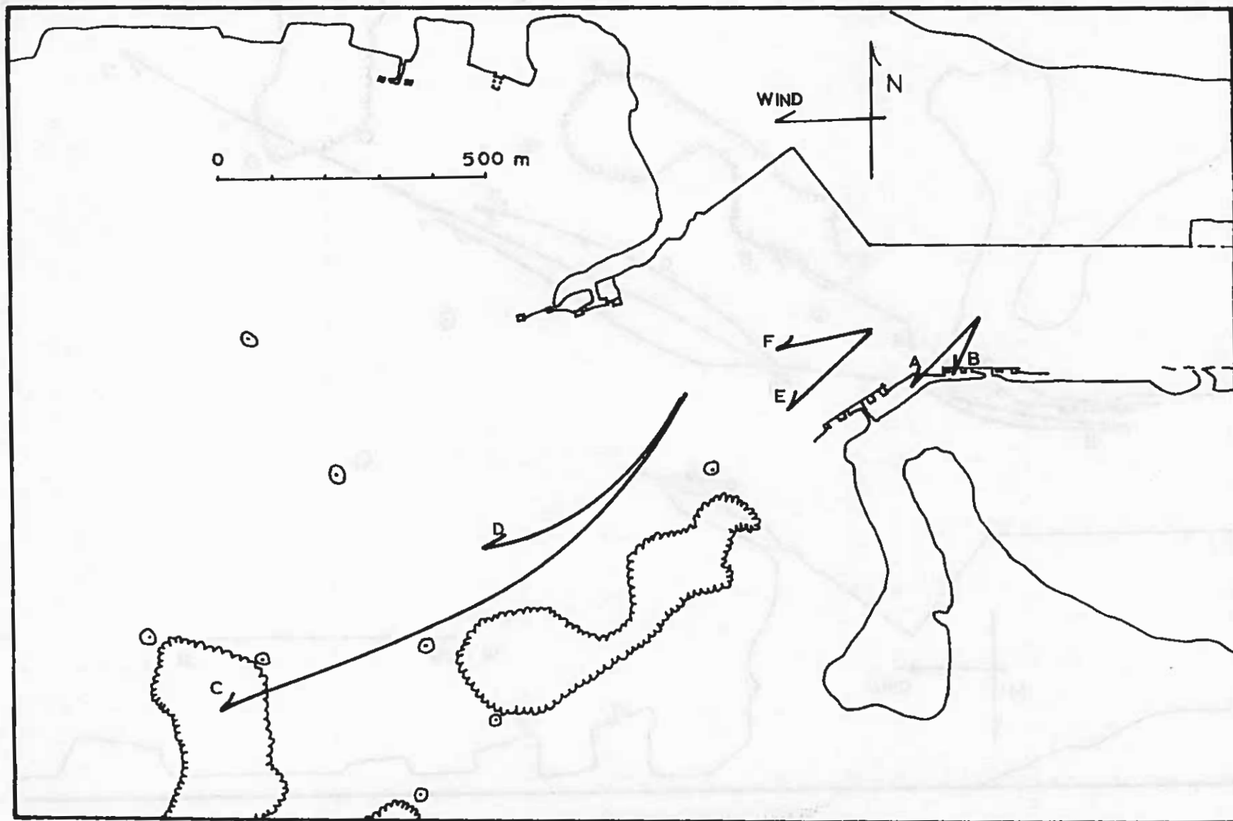
Figure 10. Inner and outer drift drogue paths for 4 January, 1977, weak falling tide, 0830-1055. The wind was from the east at 5-10 knots. A, C, E, 1-m drogue; B and F, 6-m drogue; D, 12-m drogue.
