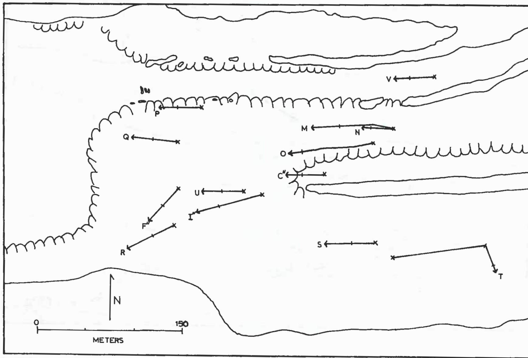
Figure 17. Dye paths in Lower Piti and Secondary Channels, Flat C and Flat D; Zone II. See Table 5 for detailed information.
