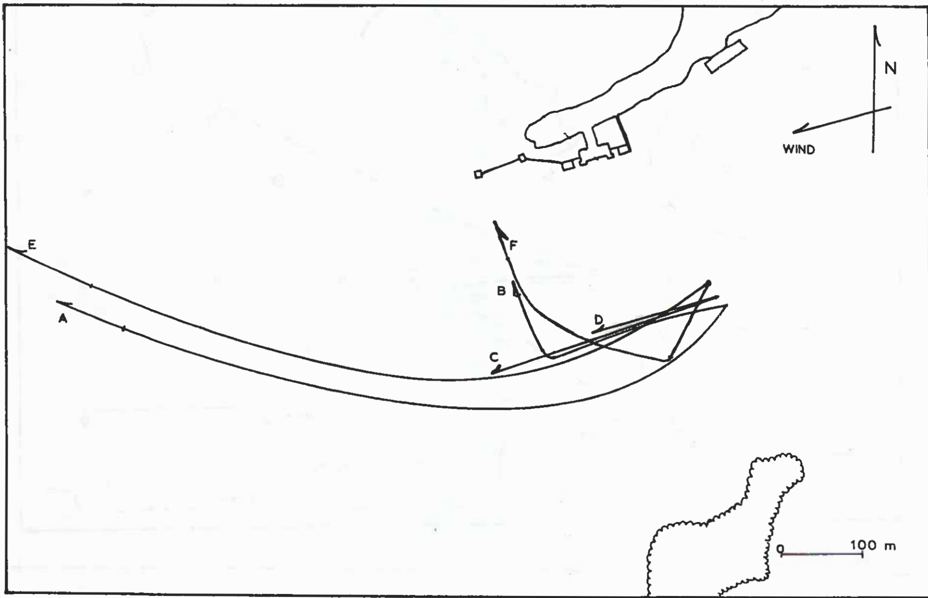
Figure 5. Outer drift drogue paths for 28 December, 1976, strong rising and weak falling tides, 0955-1522. The wind was from the east at 10 knots. E, A and C, 1-m drogue; F, B,
