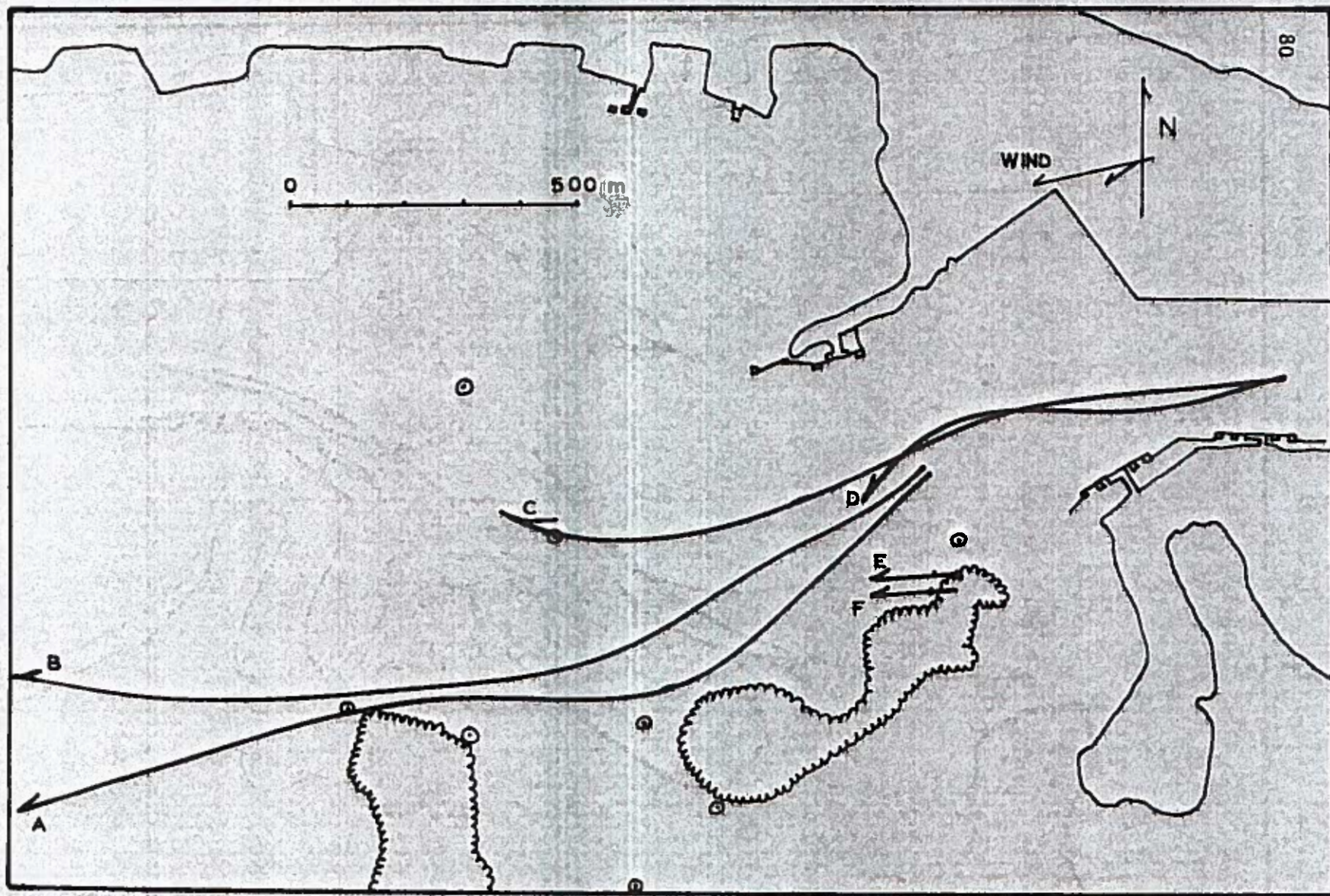
Figure 9. Inner and outer drift drogue paths for 29 December, 1976, weak falling tide, 1000-1315. The wind was from the east and northeast at 10-18 knots. Dye releases on Jade Shoals were at 1040 and 1115. A and C, 1-m drogue; B and D, 6-m drogue; E and F, Jade Shoals.
