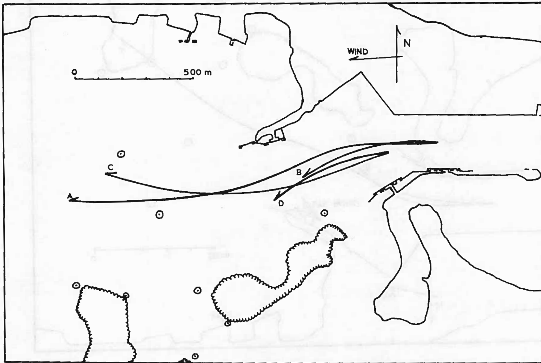
Figure 6. Inner drift drogue paths for 28 December, 1976, strong rising and weak falling tides, 1000-1530. The wind was predominantly from the east at 10-14 knots. A and C, 1 -m drogue; B and D, 6 -m drogue.
