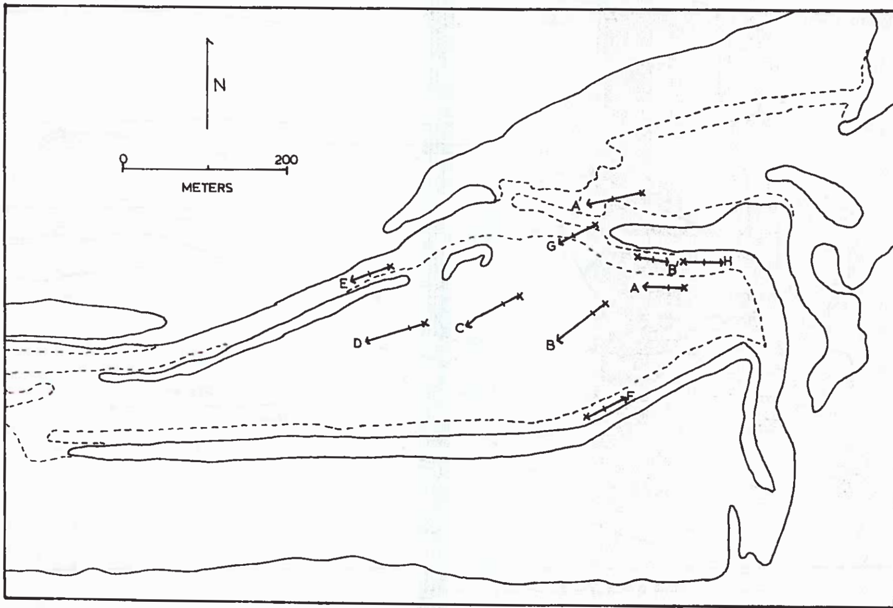
Figure 19. Dye paths of Upper Piti and Secondary Channels and Flat C; Zone III. See Table 6 for detailed information.
