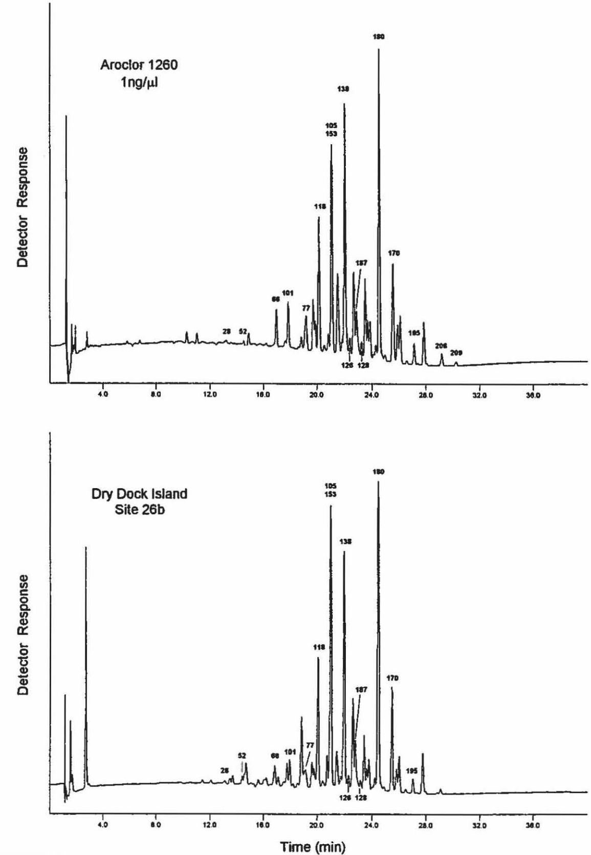
Figure 9: Polychlorinated Biphenyls in Sediments from Apra Harbor
