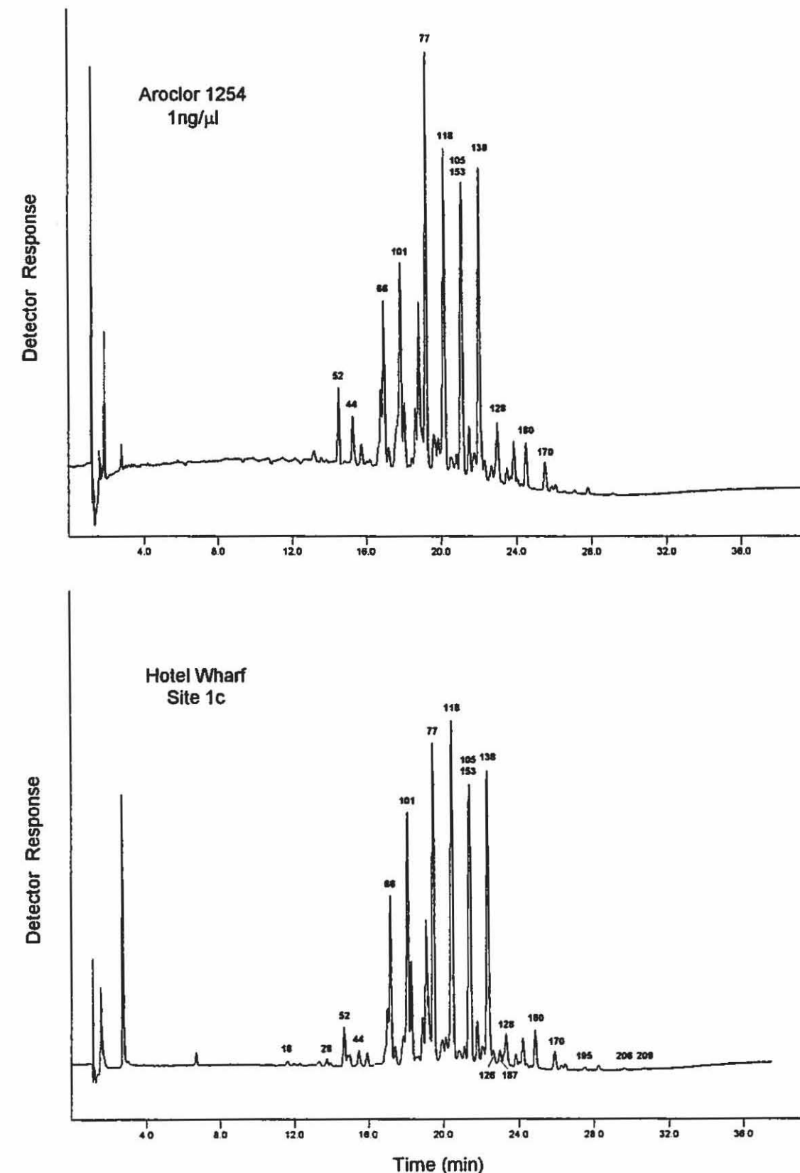
Figure 7: Polychlorinated Biphenyls in Sediments from Apra Harbor
