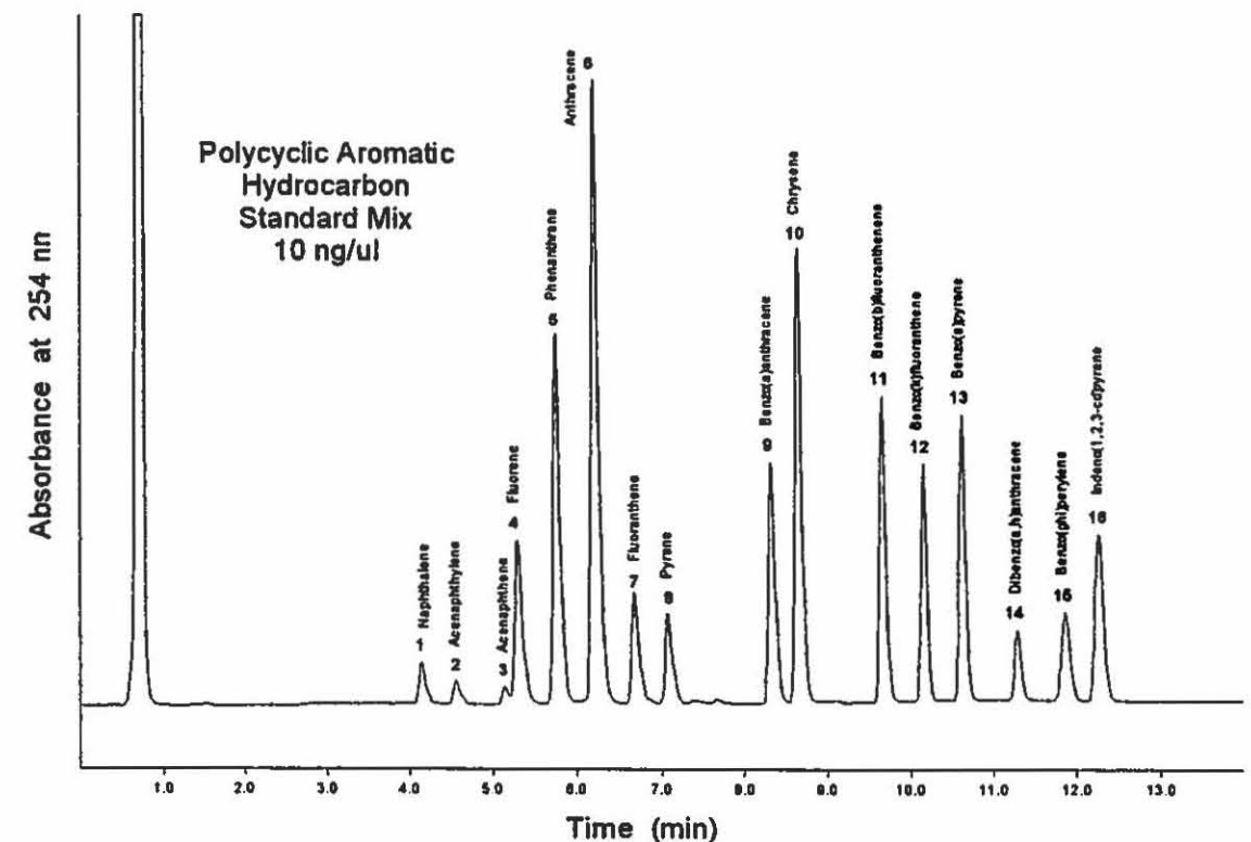
Figure 11: Polycyclic Aromatic Hydrocarbons in Sediments from Apra Harbor
