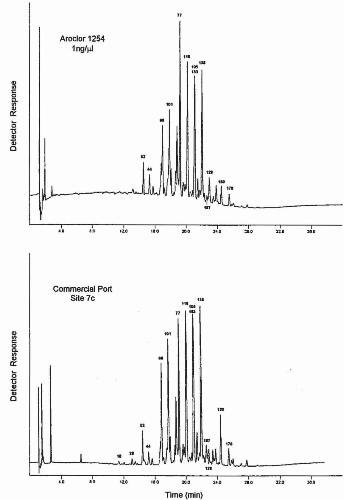
Figure 8: Polychlorinated Biphenyls in Sediments from Apra Harbor
