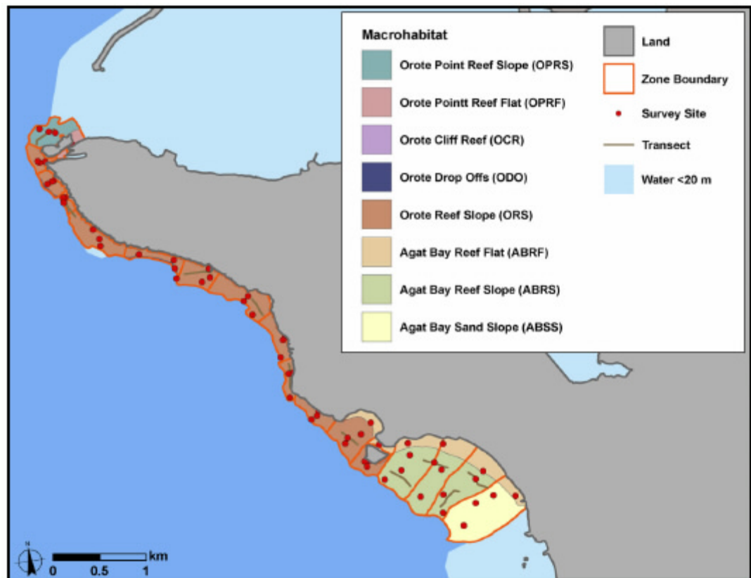
Figure 12. Macrohabitat zones, transect sites, and survey sites in the Orote Peninsula ERA. Map: Waddell, 2005. Source Paulay et al., 2001.
