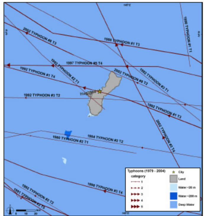
Figure 2. The path and intensity of typhoons passing near Guam from 1979-2004. Four major storms (sustained winds >150 mph) have hit Guam in the past 10 years. Map: Waddell, 2005. Data: Unisys, http://weather.unisys.com/hurricane .
