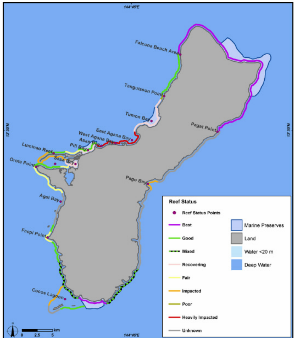
Figure 28. Summary map showing the overall condition of Guam's coral reef ecosystems. Map: Waddell, 2005. Source: DAWR.
