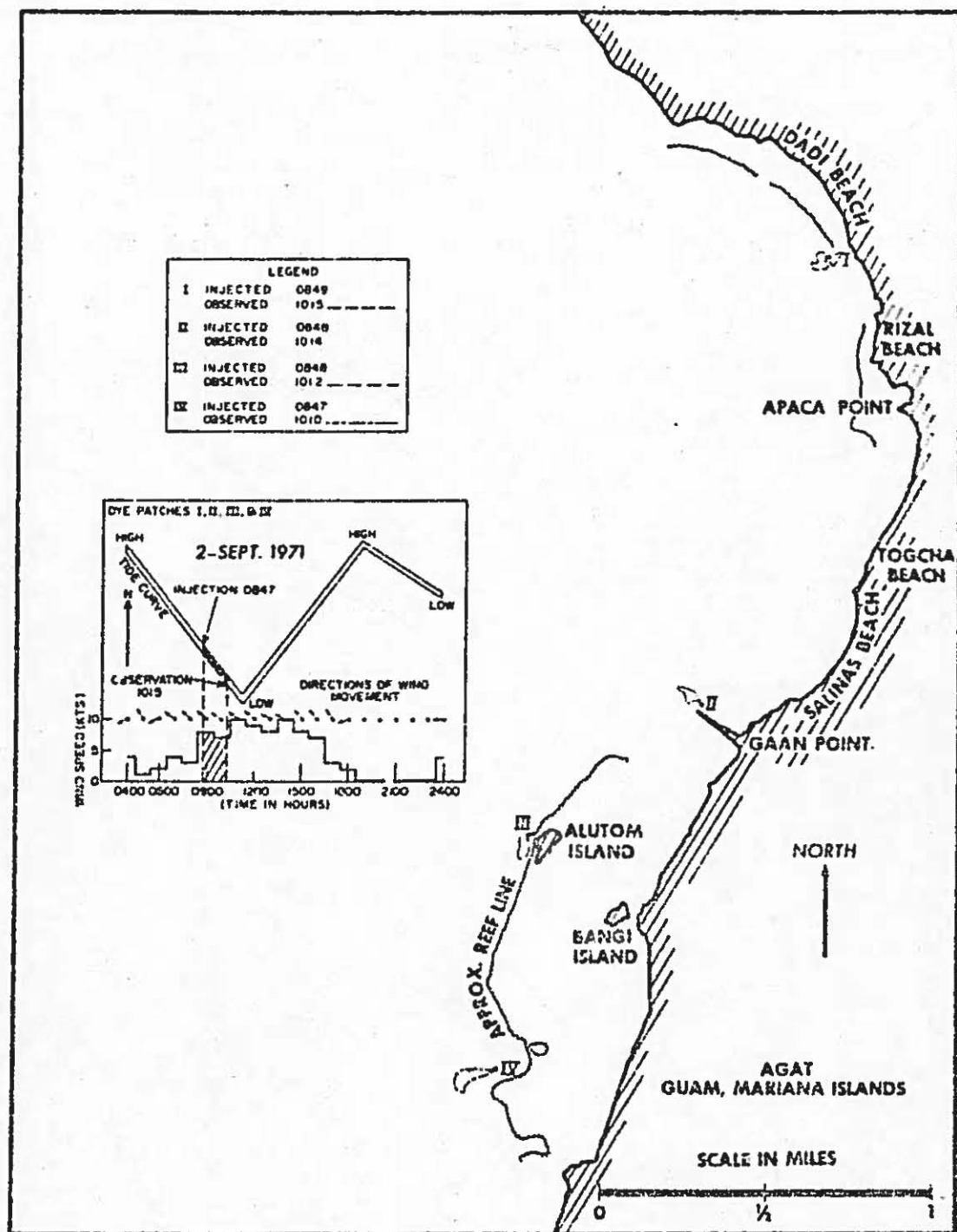
Figure 44. Dye movement at Agat Bay on 2 September 1971.
