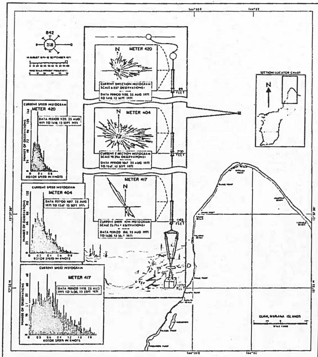
Figure 106. Current speed histograms and current direction histograms for the Ritidian Section in summer including meters #420, #404, and #417 and a wind rose for the data period.
