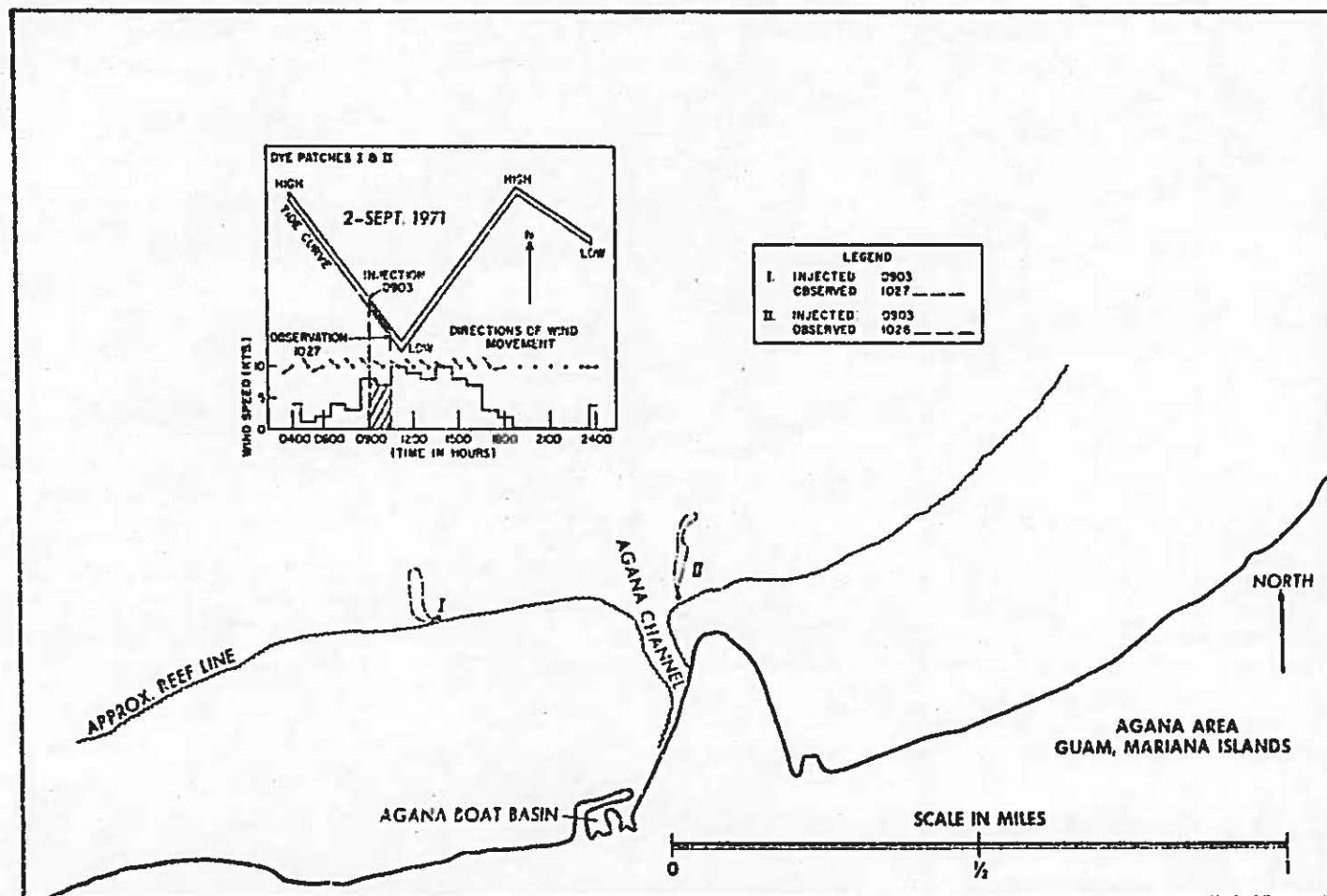
Figure 83. Dye movement at Agana Bay on 2 September 1971.
