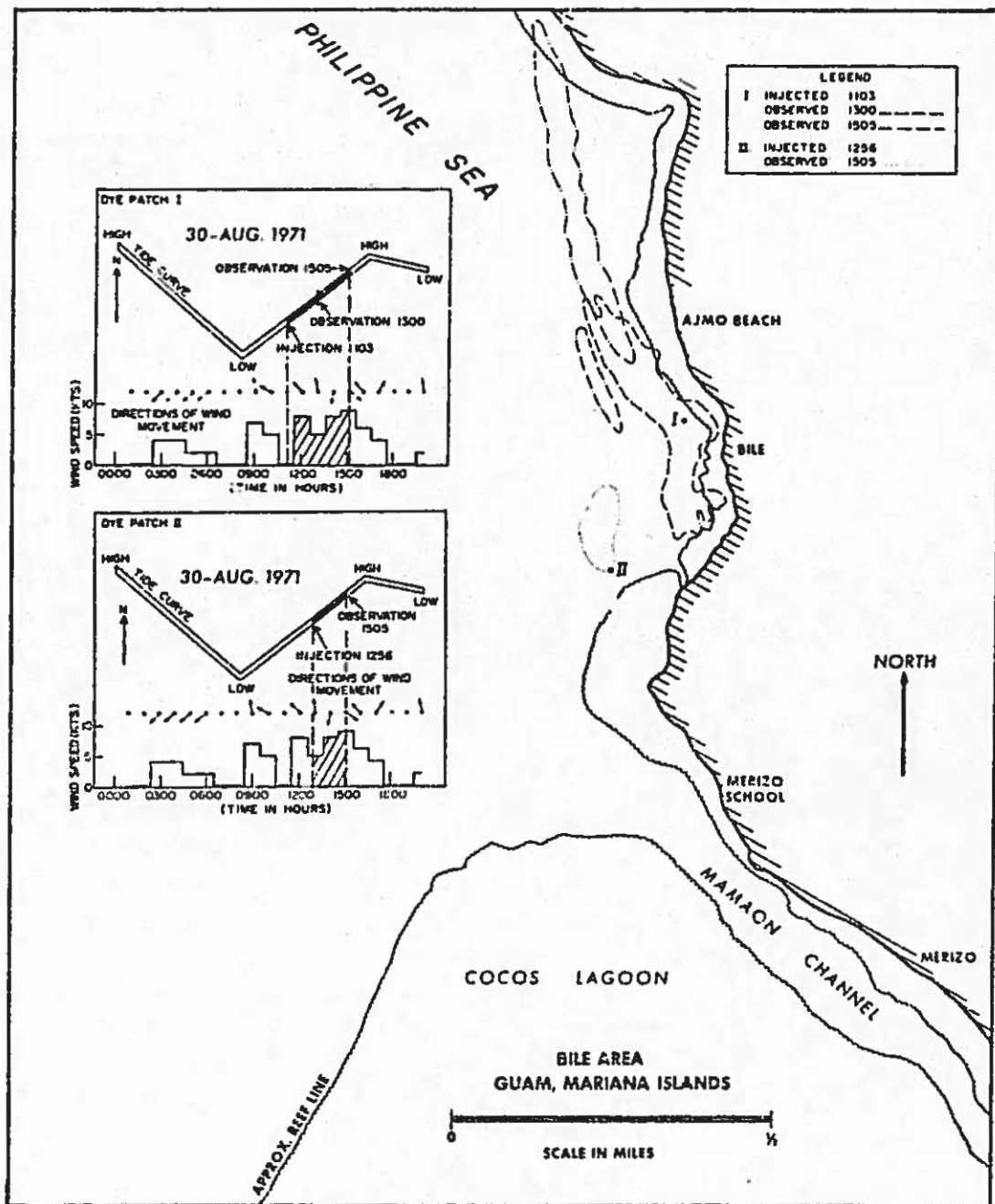
Figure 16. Dye movement at Bile Bay on 30 August 1971.
