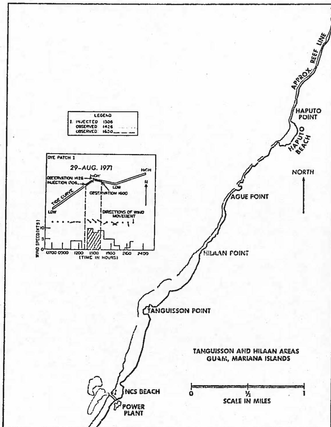
Figure 96. Dye movement at Tanguisson Point on 29 August 1971.
