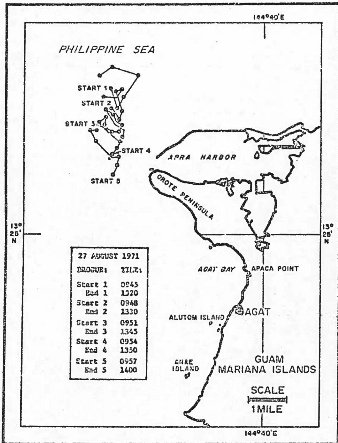
Figure 57. Drogue observations in Agat Section, 27 August 1971.
