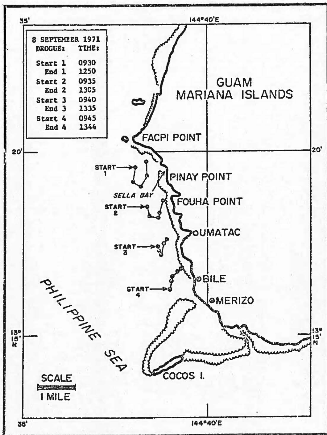
Figure 33. Drogue observations in Bile Section, 8 September 1971.
