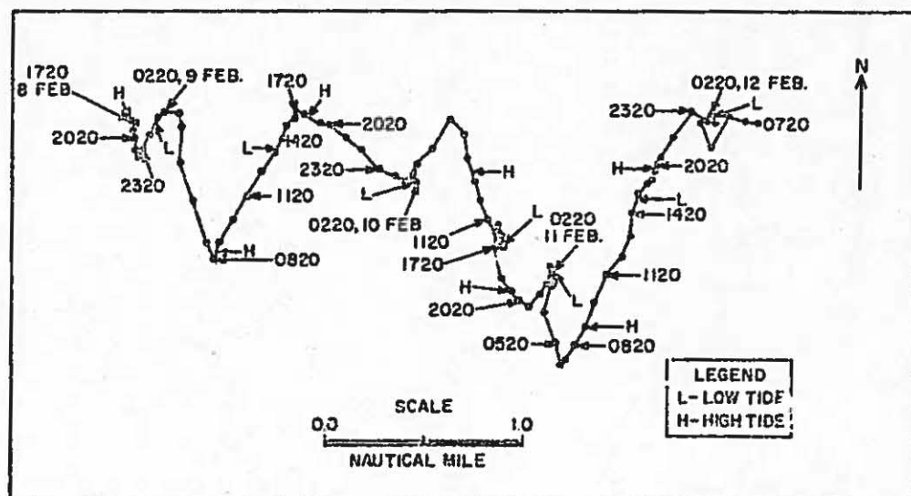
Figure 6. Progressive vector diagram of current from meter #223, 8 - 12 February 1971.
