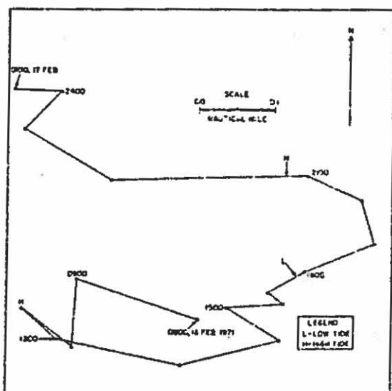
Figure 74. Progressive vector diagram of current from meter #346, 0800, 16 February to 0100, 17 February 1971.
