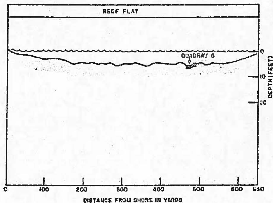
Figure 128. Area chart and reef profile for Bangi Island ecological study.
