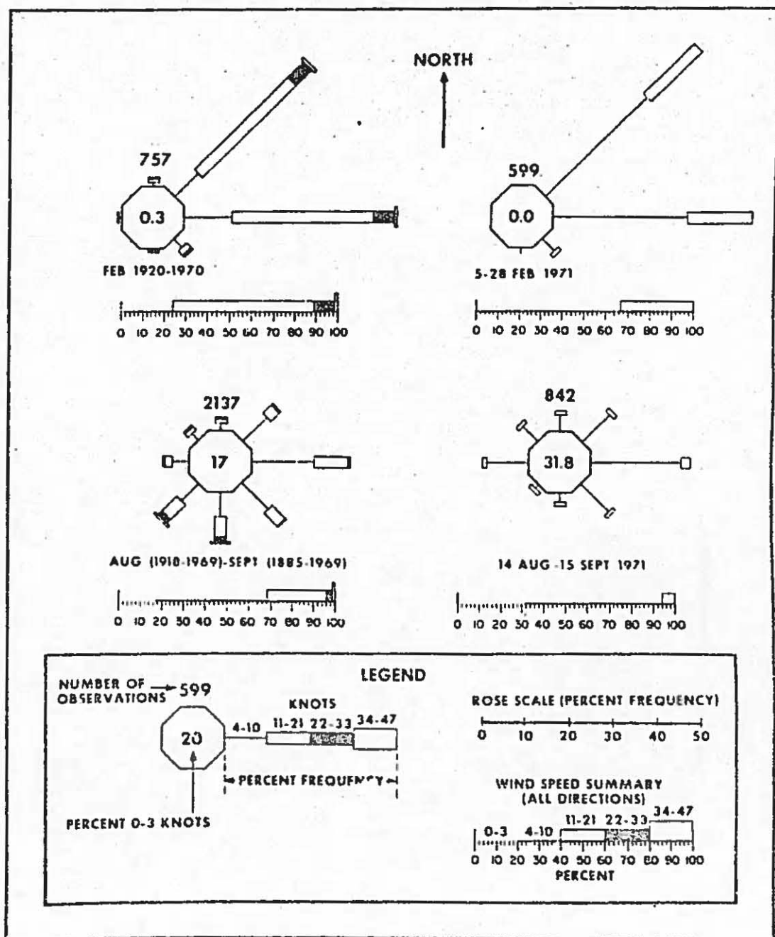
Figure 3. Wind roses of historical data and 1971 data.
