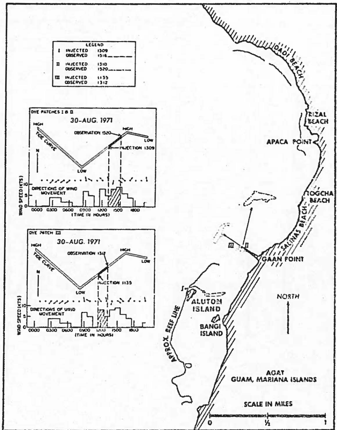
Figure 41. Dye movement at Agat Bay on 30 August 1971.
