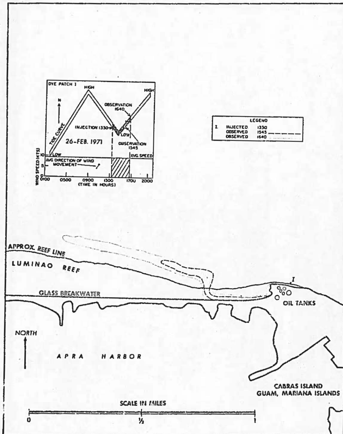
Figure 67. Dye movement at Cabras Island on 26 February 1971, P.M.
