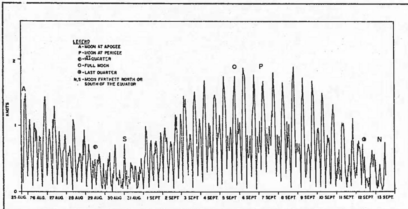
Figure 107. Current speed plot from meter #417, 25 August to 13 September 1971.
