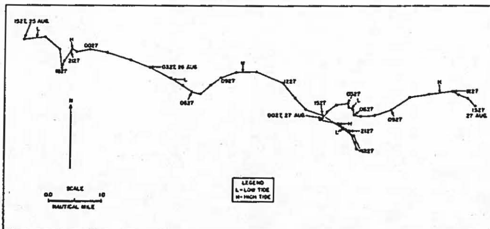
Figure 109. Progressive vector diagram of current from meter #420, 1527, 25 August to 1527, 27 August 1971.
