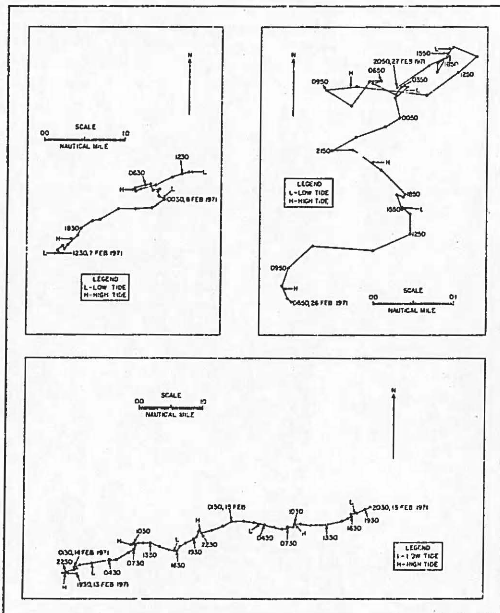
Figure 76. Progressive vector diagrams of current from meter #103, 1230, 7 February to 1330, 8 February; 0650, 26 February to 2050, 27 February; and 1930, 13 February to 2030, 15 February 1971.
