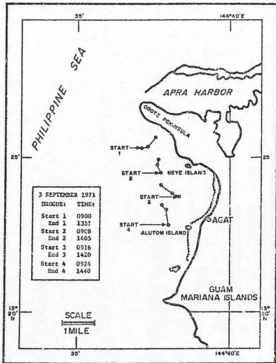
Figure 59. Drogue observations in Agat Section, 3 September 1971.
