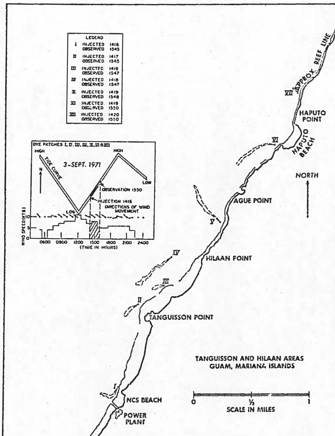
Figure 103. Dye movement at Tanguisson Point on 3 September 1971, P.M.
