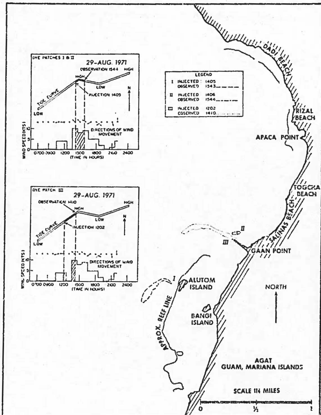
Figure 40. Dye movement at Agat Bay on 29 August 1971.
