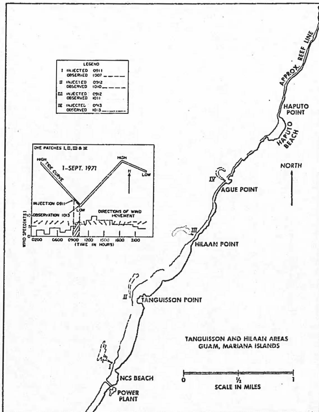
Figure 95. Dye movement at Tanguisson Point on 1 September 1971.
