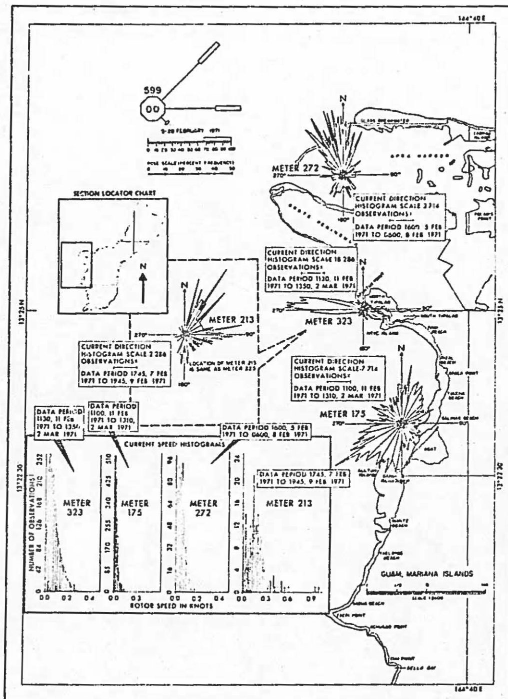
Figure 34. Current speed histograms and current direction histograms for the Agat Section in winter including meters #323, #175, #272, and #213 and a wind rose for the data period.
