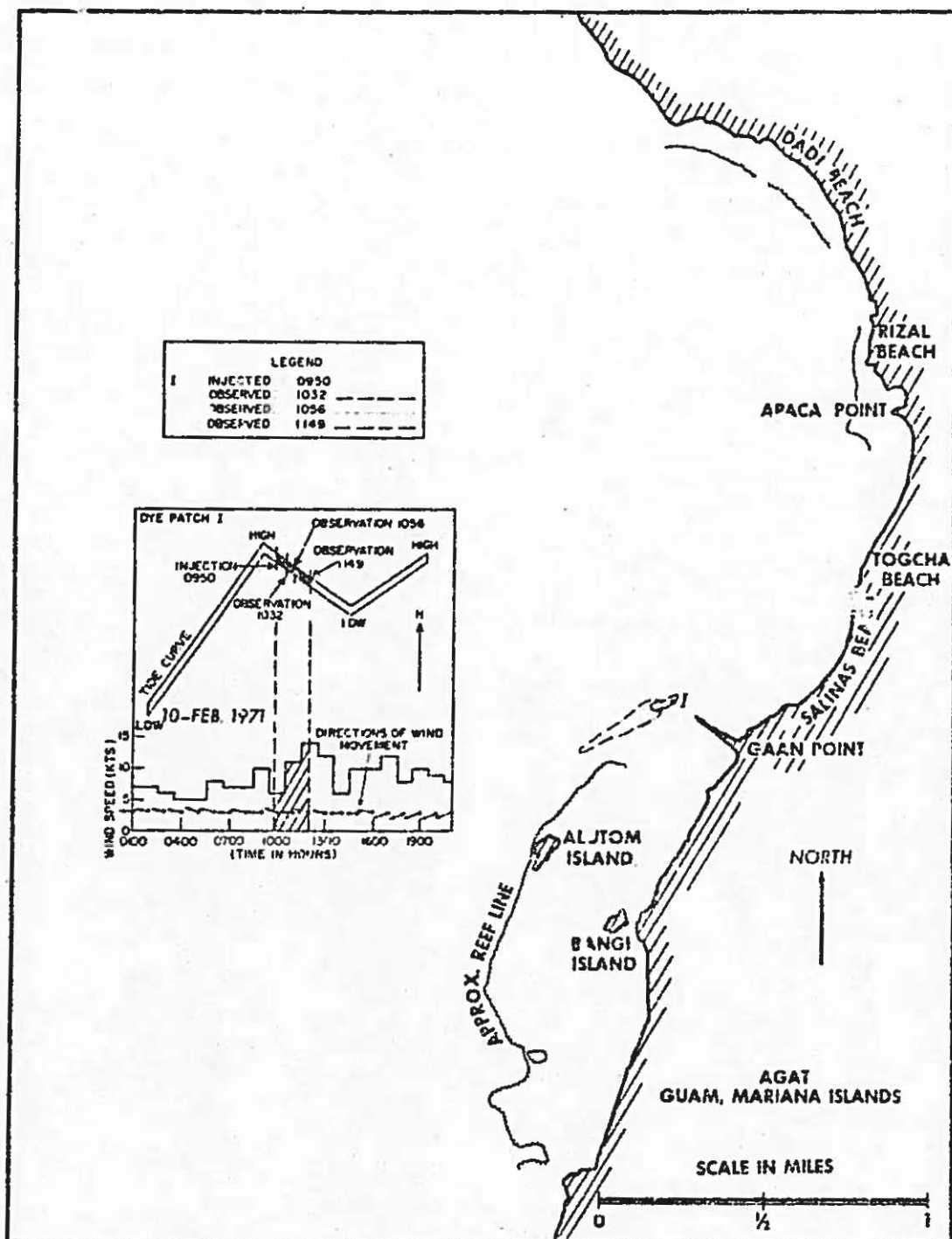
Figure 37. Dye movement at Agat Bay on 10 February 1971, A.M.
