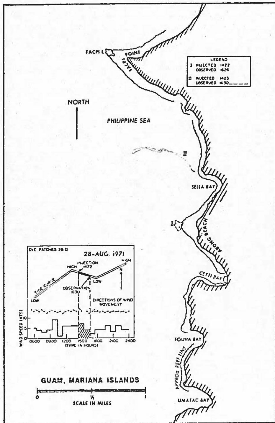
Figure 23. Dye movement at Sella Bay on 28 August 1971.
