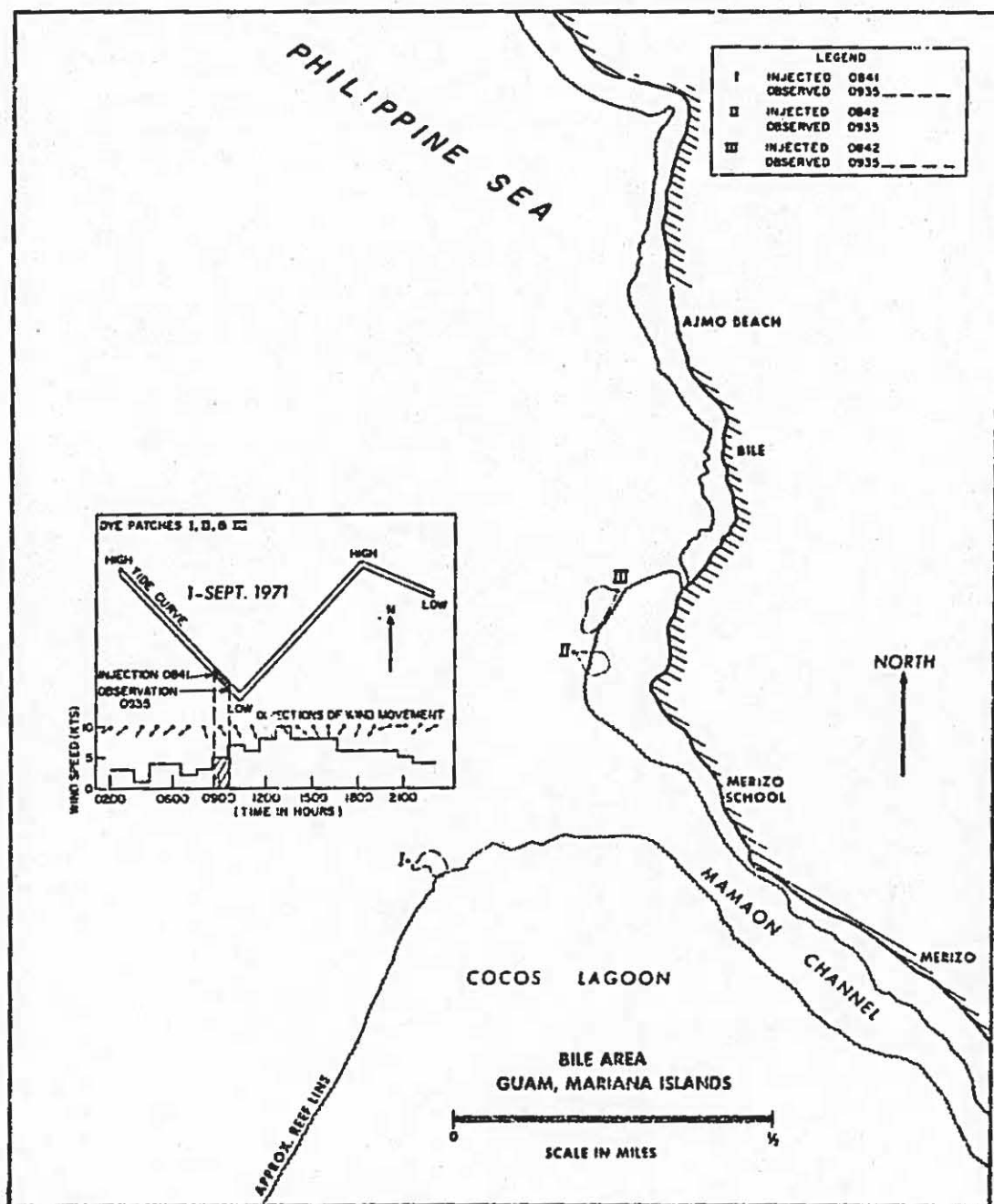
Figure 18. Dye movement at Bile Bay on 1 September 1971.
