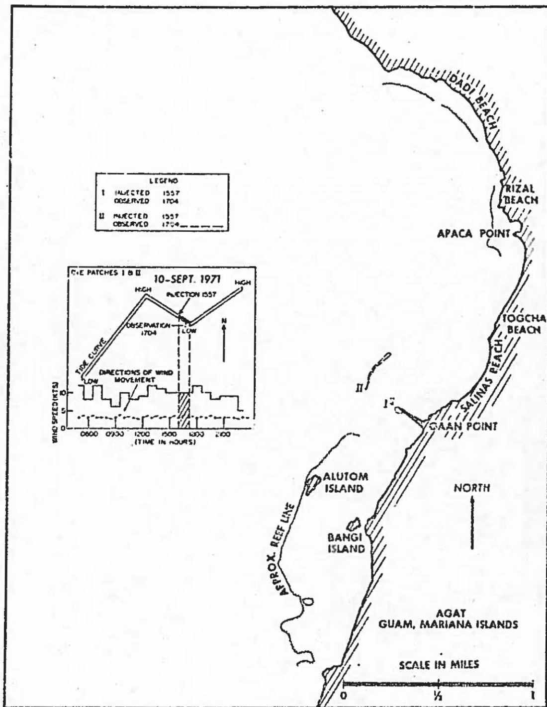
Figure 46. Dye movement at Agat Bay on 10 September 1971.
