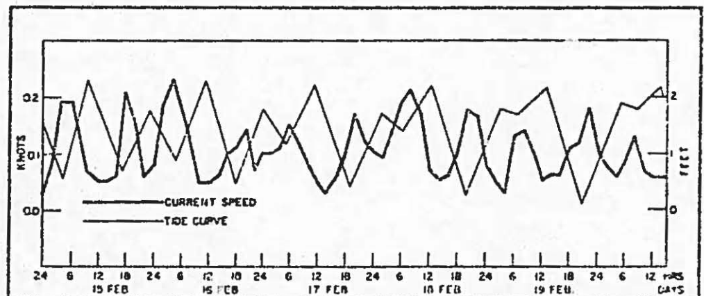
Figure 47. Current speeds versus tides from meter #323, 0000, 15 February to 1400, 20 February 1971.
