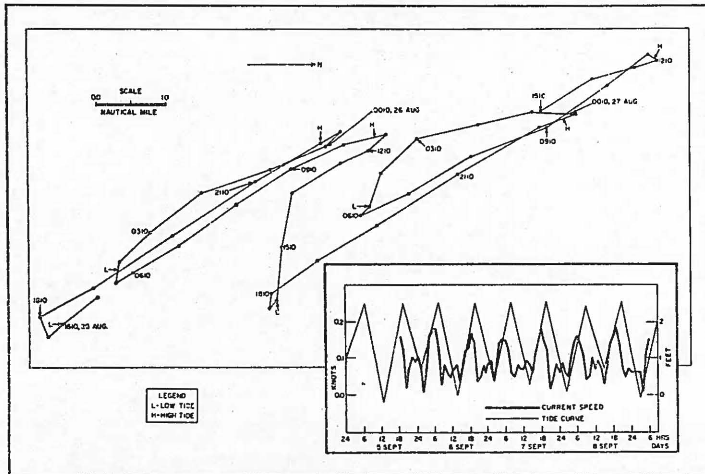
Figure 108. Progressive vector diagram of current from meter #417, 1610, 25 August to 1510, 27 August 1971, and current speeds versus tides, 0000, 5 September to 1200, 9 September 1971.
