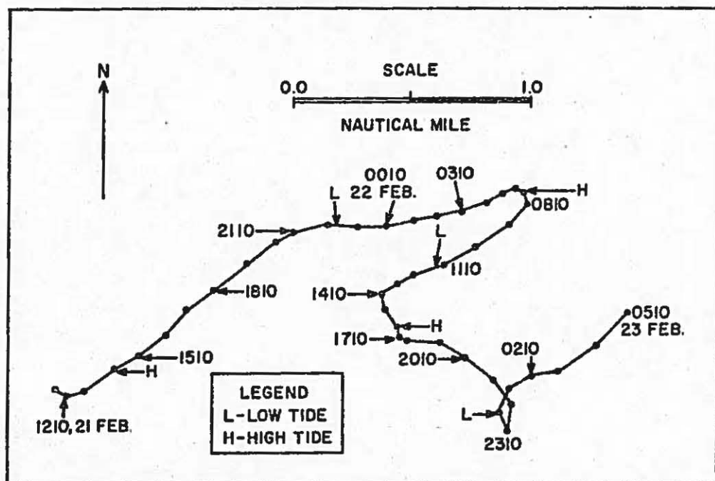
Figure 5. Progressive vector diagram of current from meter #223, 1210, 21 February to 0510, 23 February 1971.
