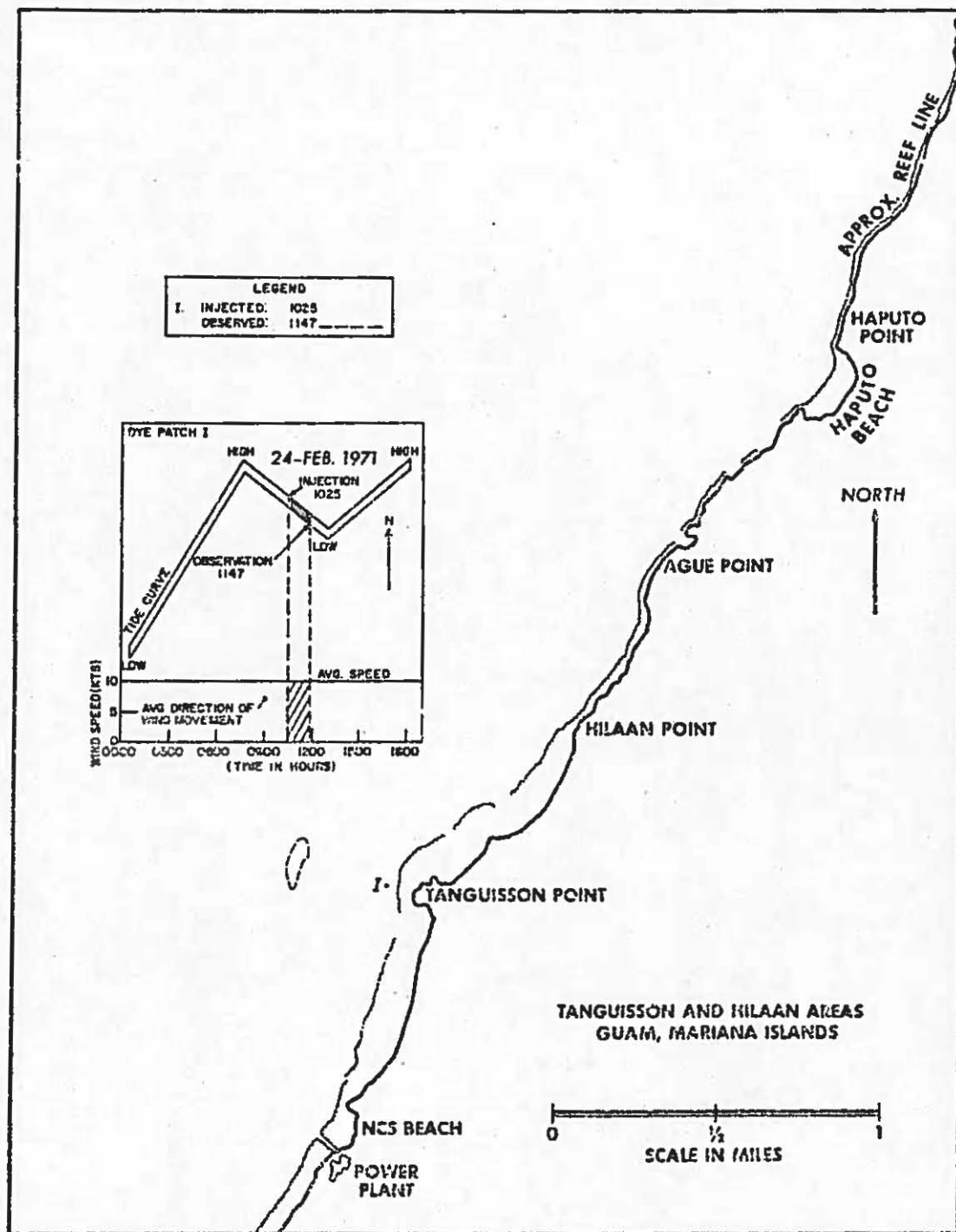
Figure 91. Dye movement at Tanguisson Point on 24 February 1971.
