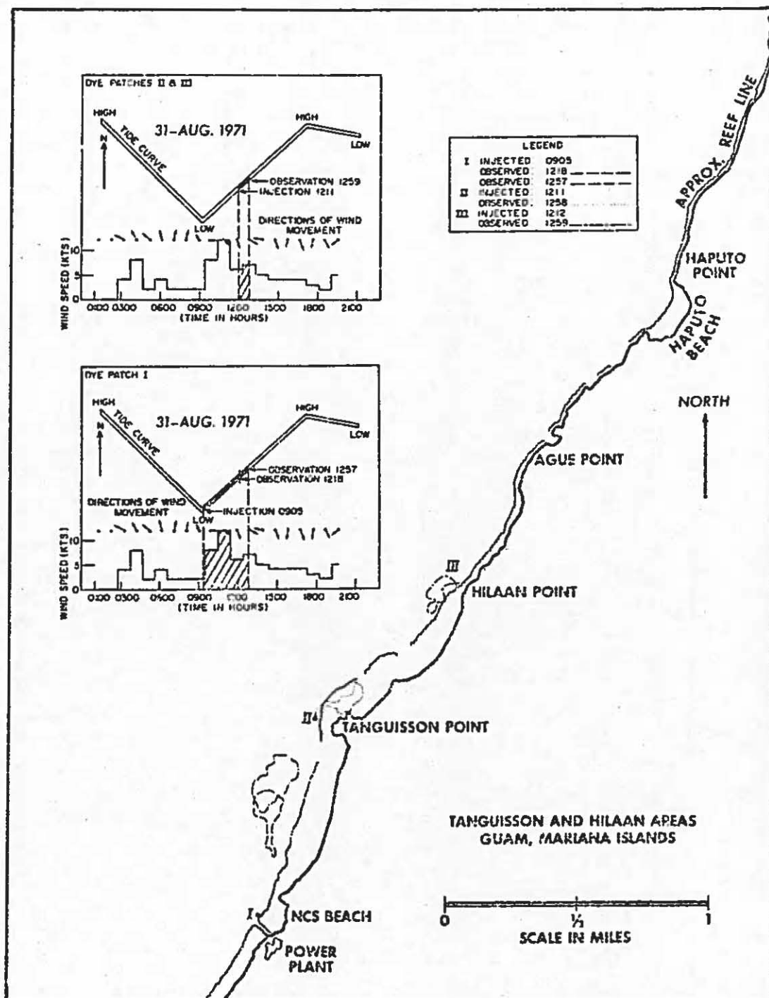
Figure 98. Dye movement at Tanguisson Point on 31 August 1971.
