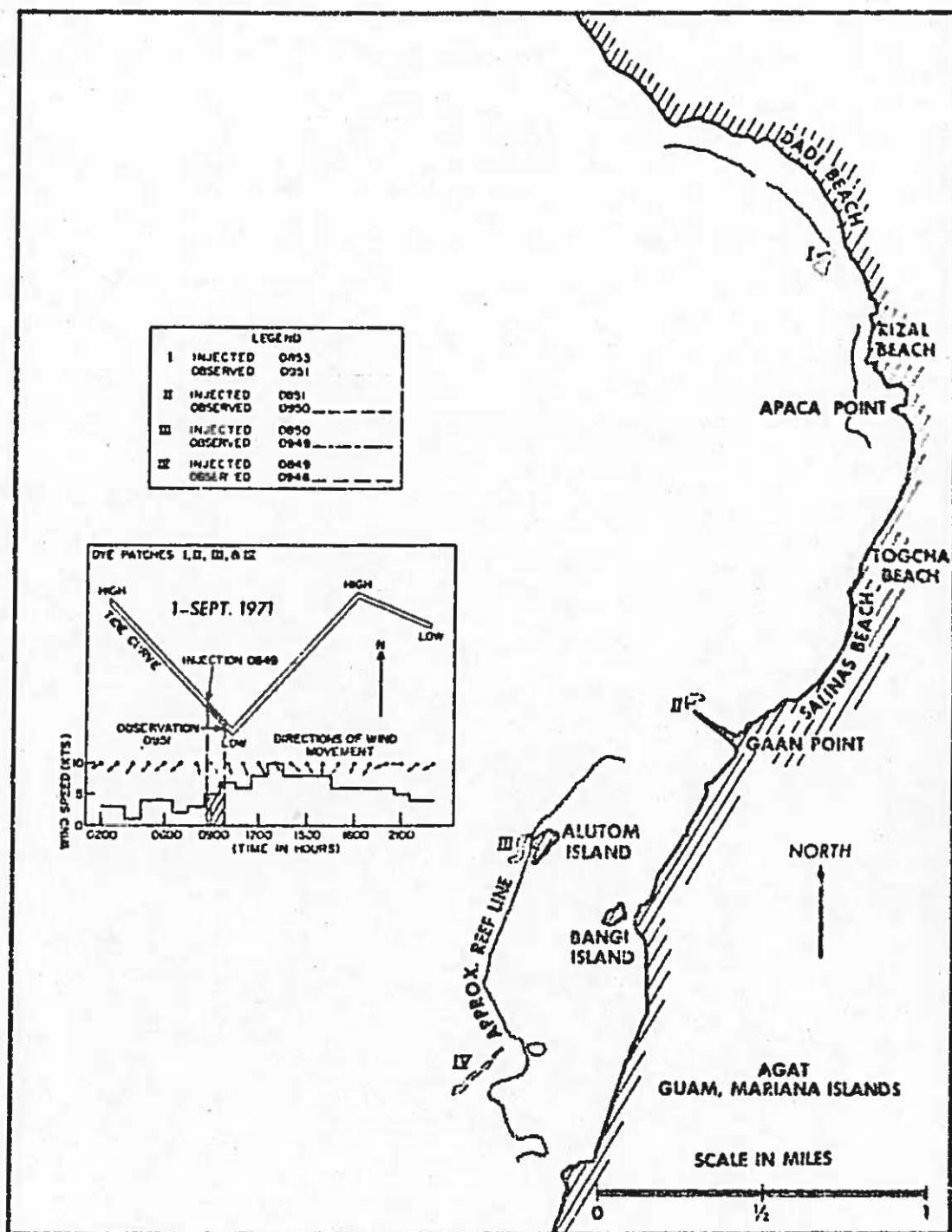
Figure 43. Dye movement at Agat Bay on 1 September 1971.
