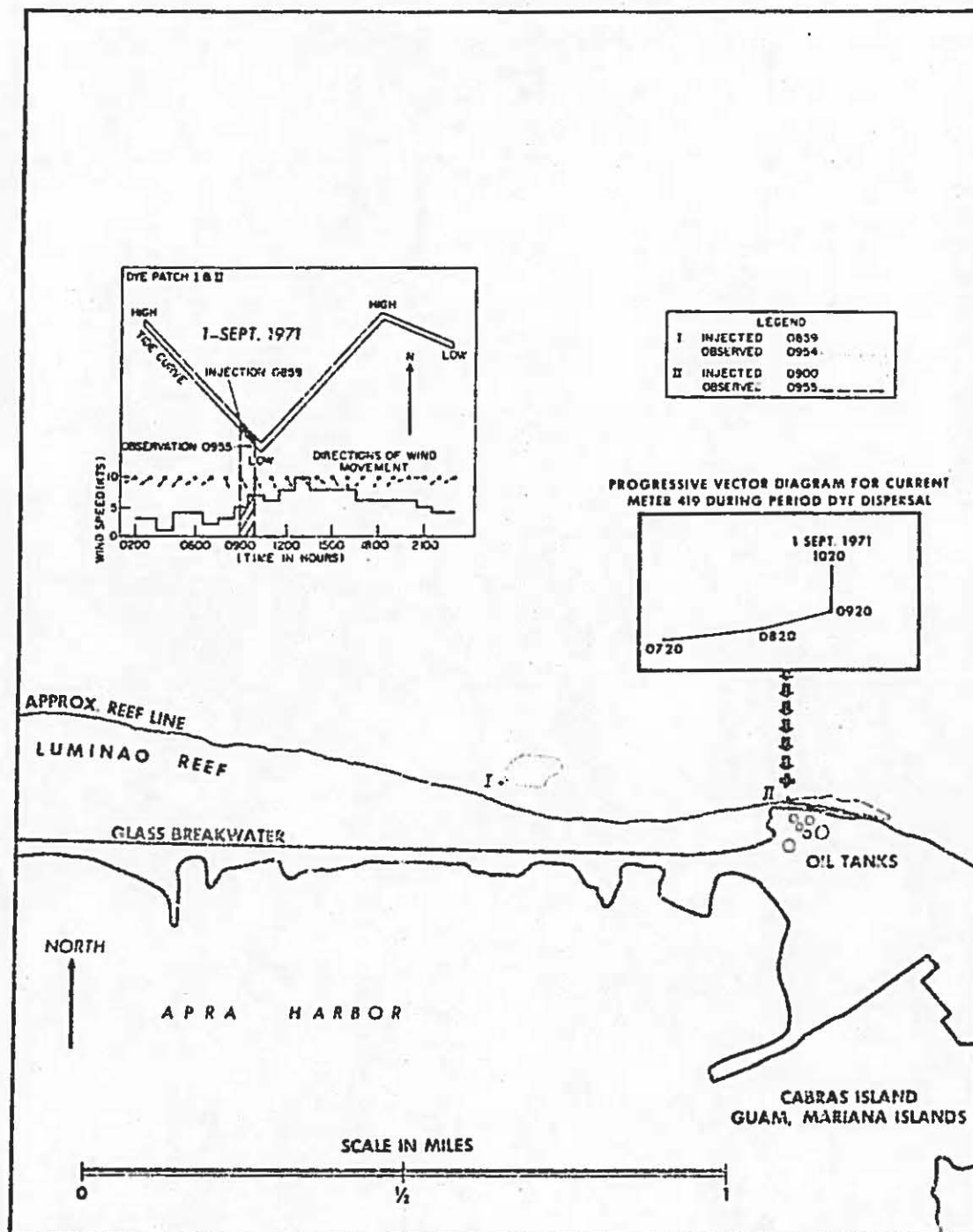
Figure 71. Dye movement at Cabras Island on 1 September 1971.
