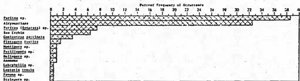
Figure 133. Frequency of occurrence of coral in quadrat 7, Piti Bay.
