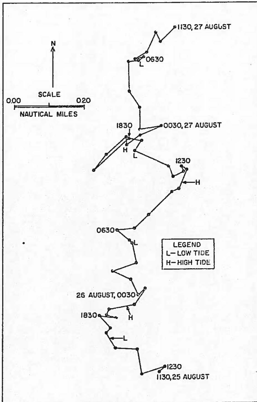
Figure 89. Progressive vector diagram of current from meter #424, 1130, 25 August to 1130, 27 August 1971.
