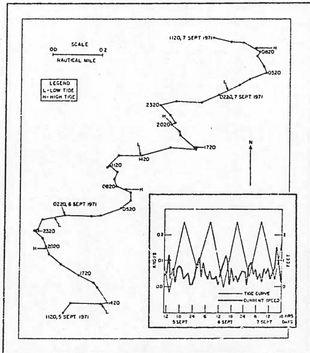
Figure 63. Progressive vector diagram of current from meter #419, 1120, 5 September to 1120, 7 September 1971, and current speeds versus tides for the same period.
