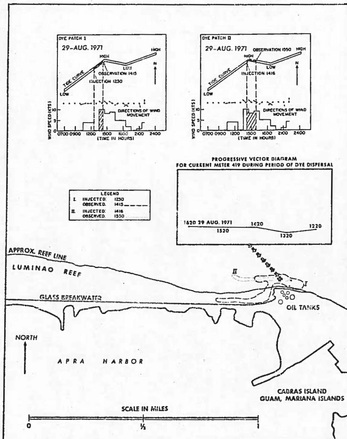
Figure 68. Dye movement at Cabras Island on 29 August 1971.
