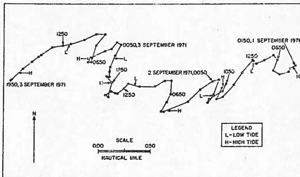
Figure 90. Progressive vector diagram of current from meter #410, 0150, 1 September to 1950, 3 September 1971.
