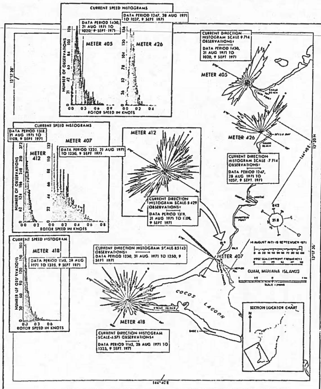
Figure 7. Current speed histograms and current direction histograms for the Bile Section in summer including meters #405, #426, #412, #407, and #418 and a wind rose for the data period.
