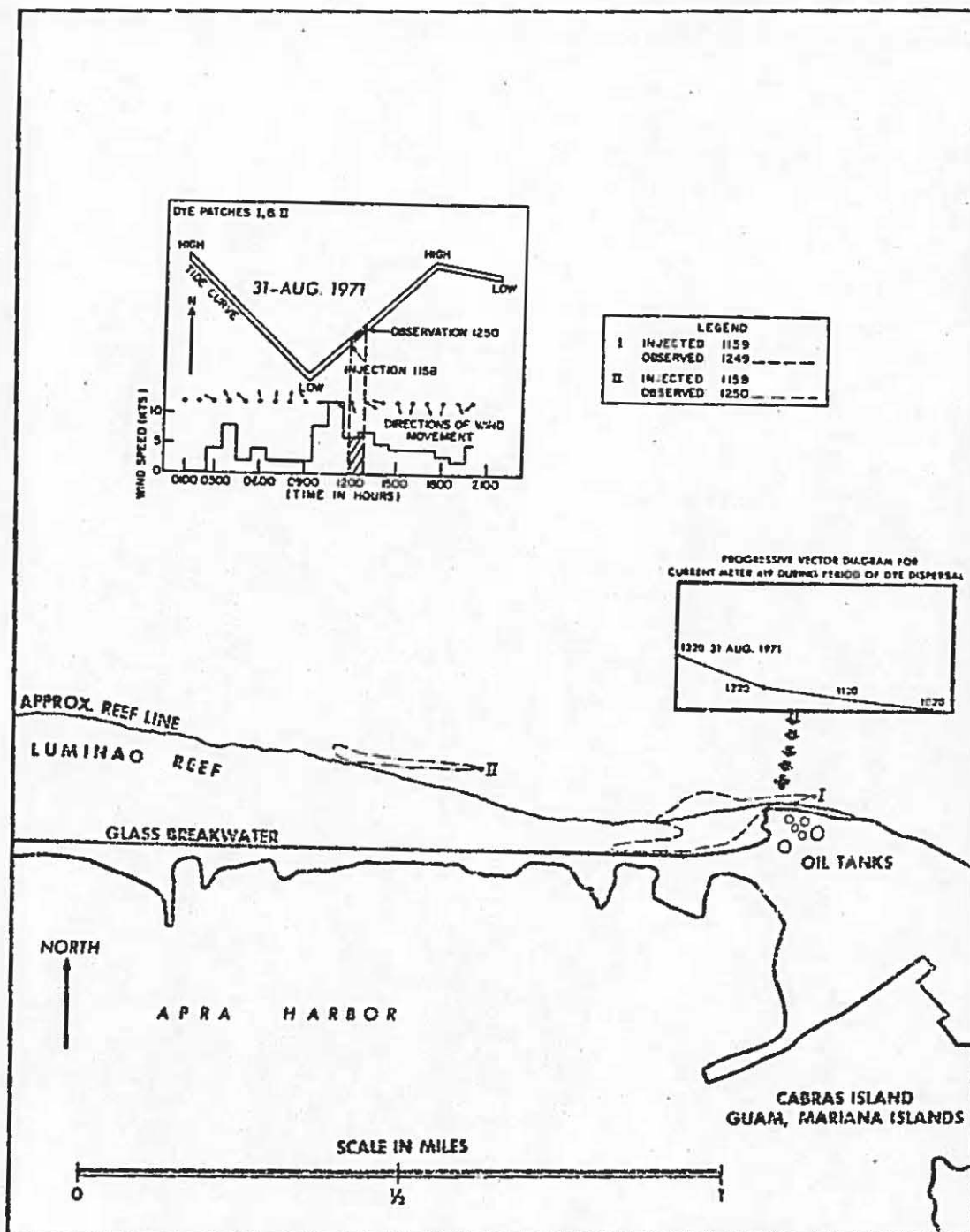
Figure 70. Dye movement at Cabras Island on 31 August 1971.
