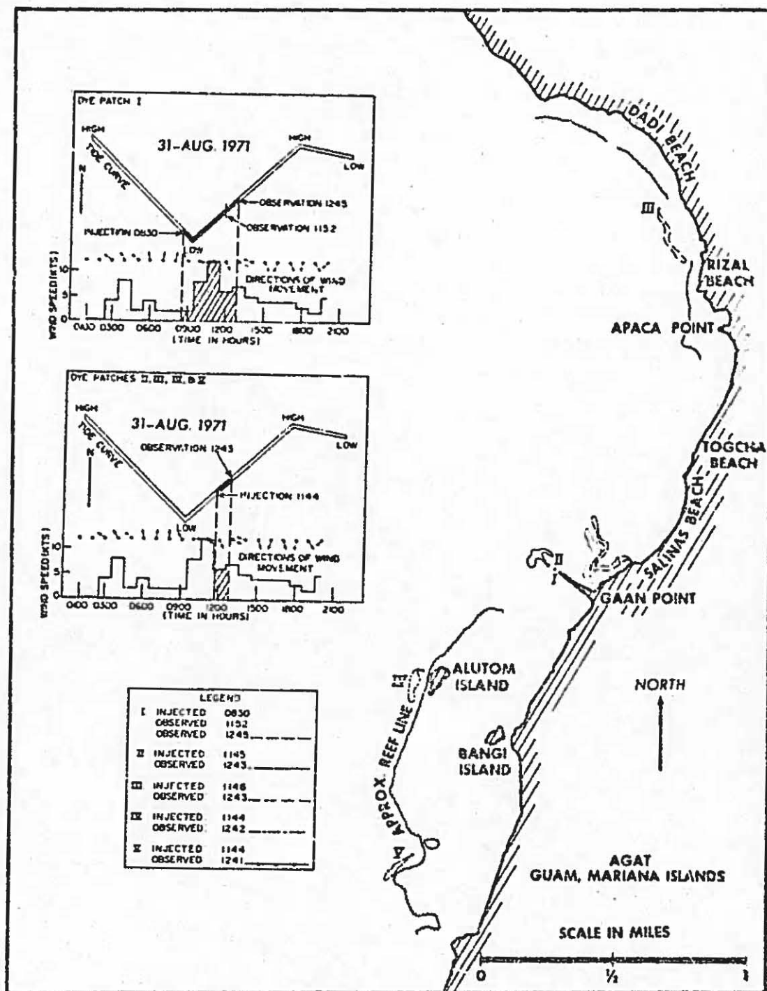
Figure 42. Dye movement at Agat Bay on 31 August 1971.
