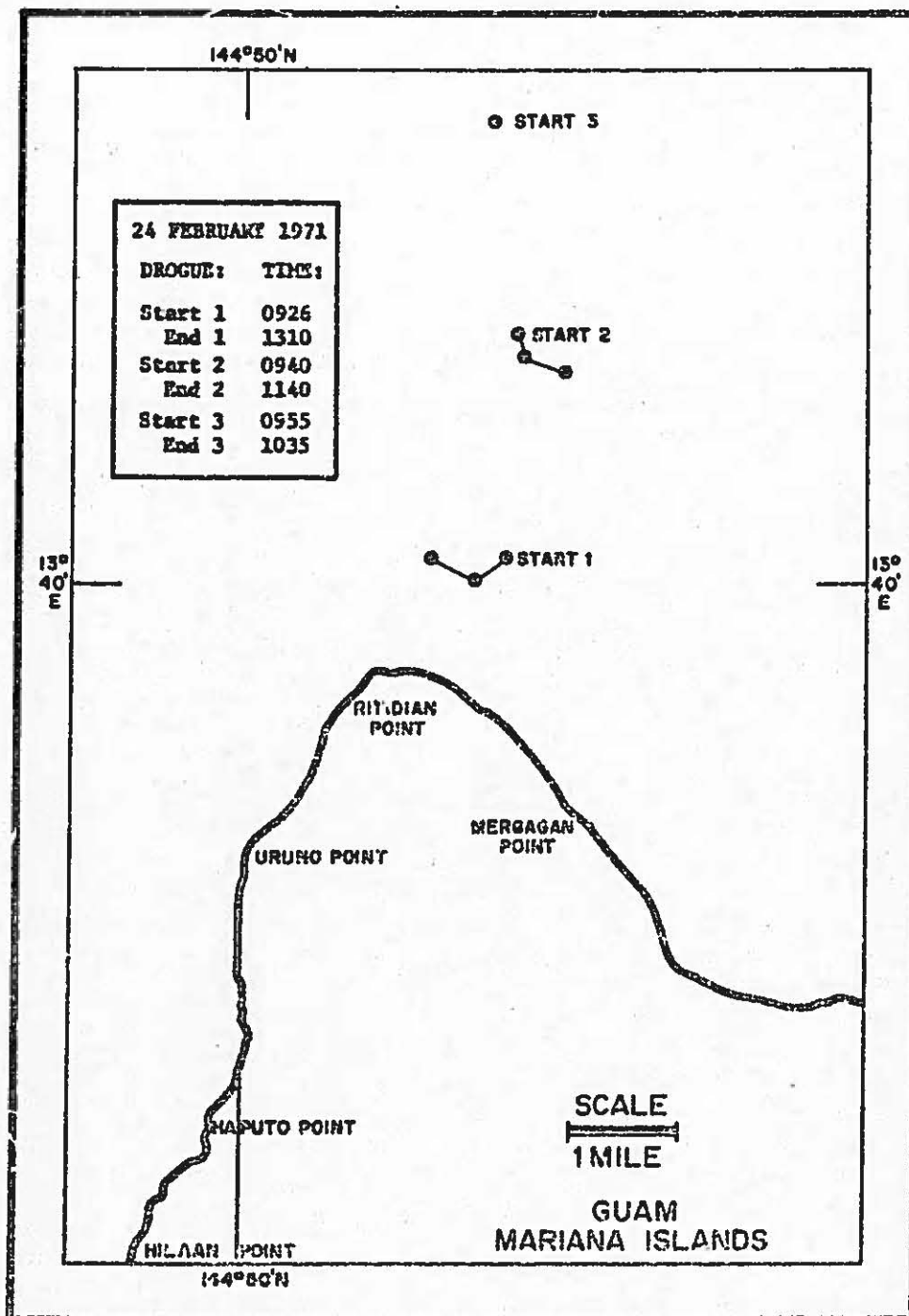
Figure 111. Drogue observations in Ritidian Section, 24 February 1971.
