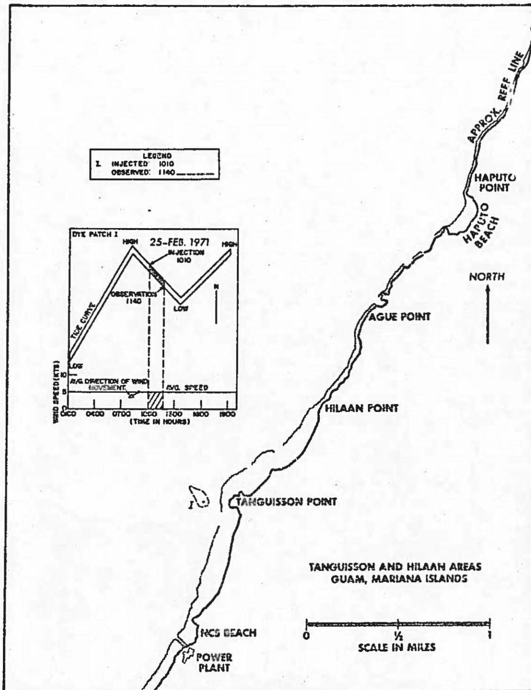
Figure 92. Dye movement at Tanguisson Point on 25 February 1971, A.M.
