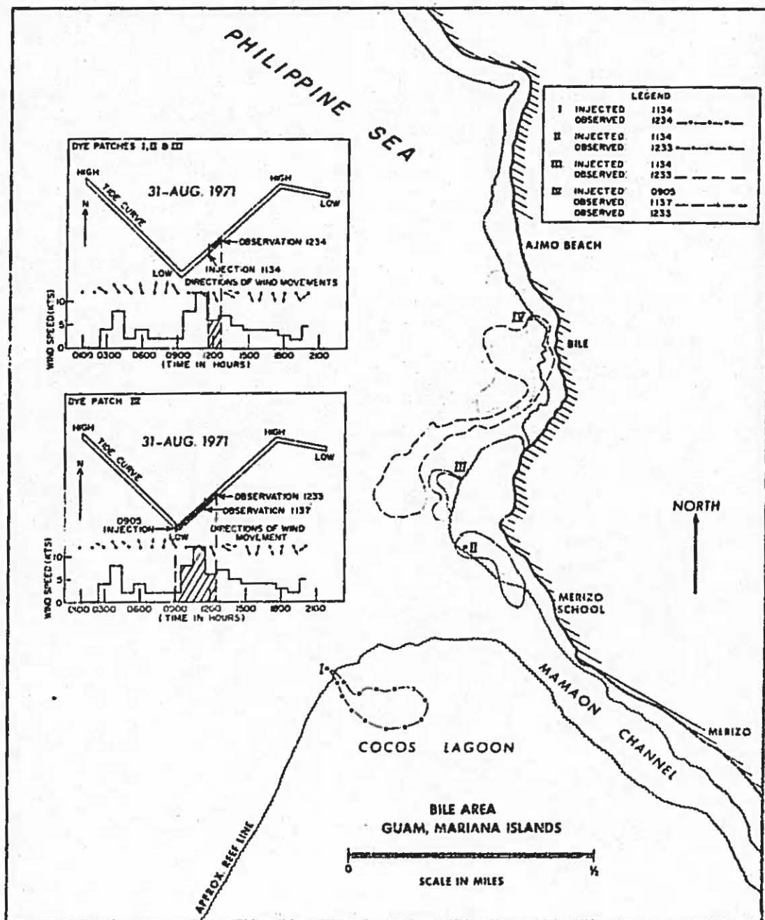
Figure 17. Dye movement at Bile Bay on 31 August 1971.
