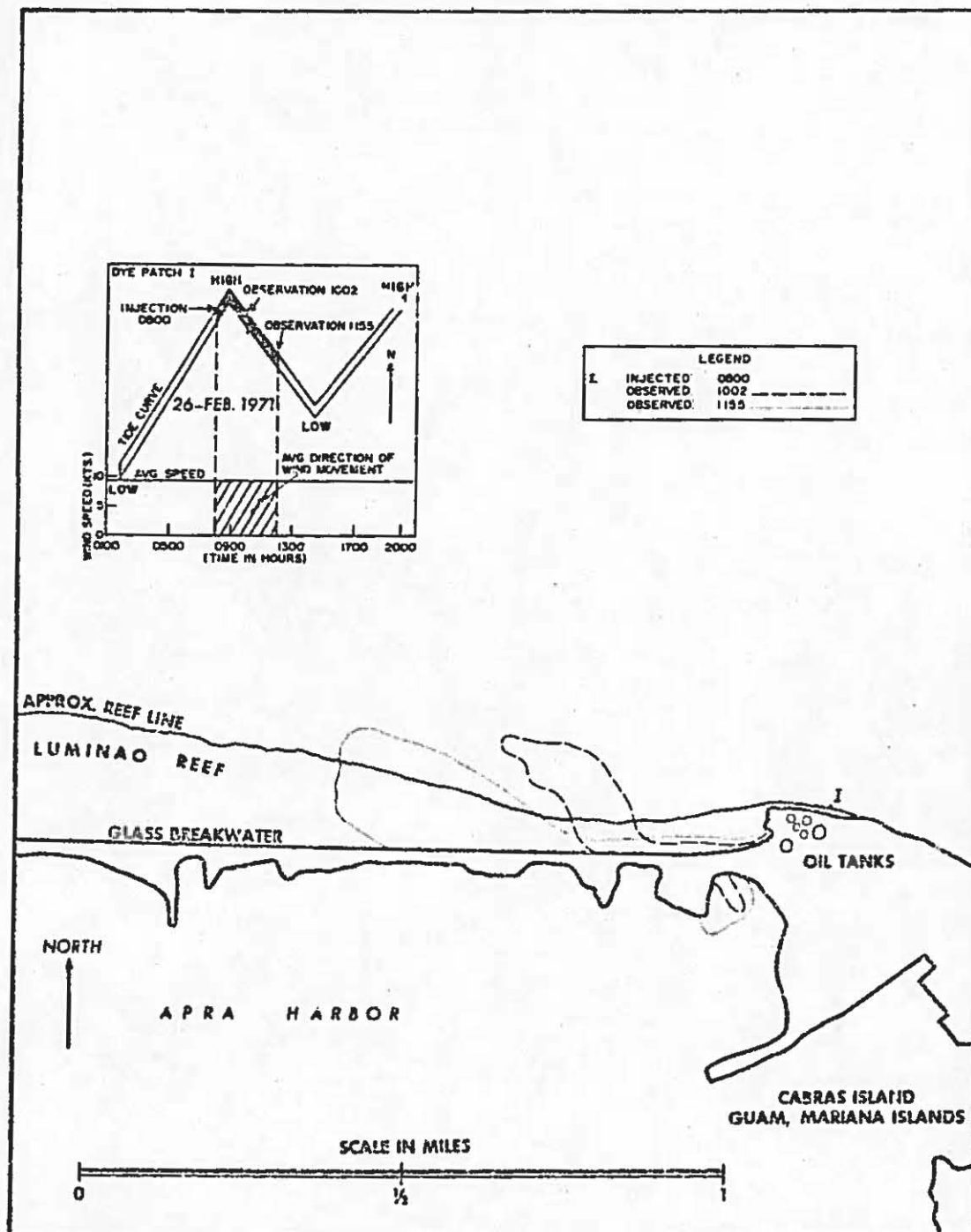
Figure 66. Dye movement at Cabras Island on 26 February 1971, A.M.
