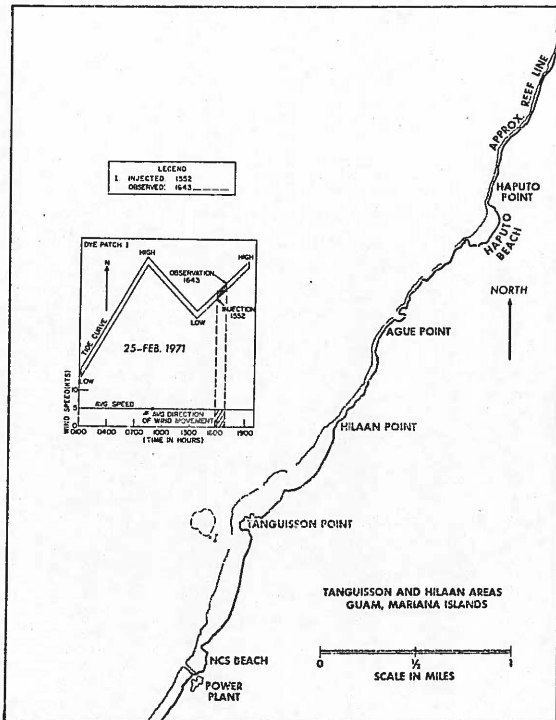
Figure 93. Dye movement at Tanguisson Point on 25 February 1971, P.M.
