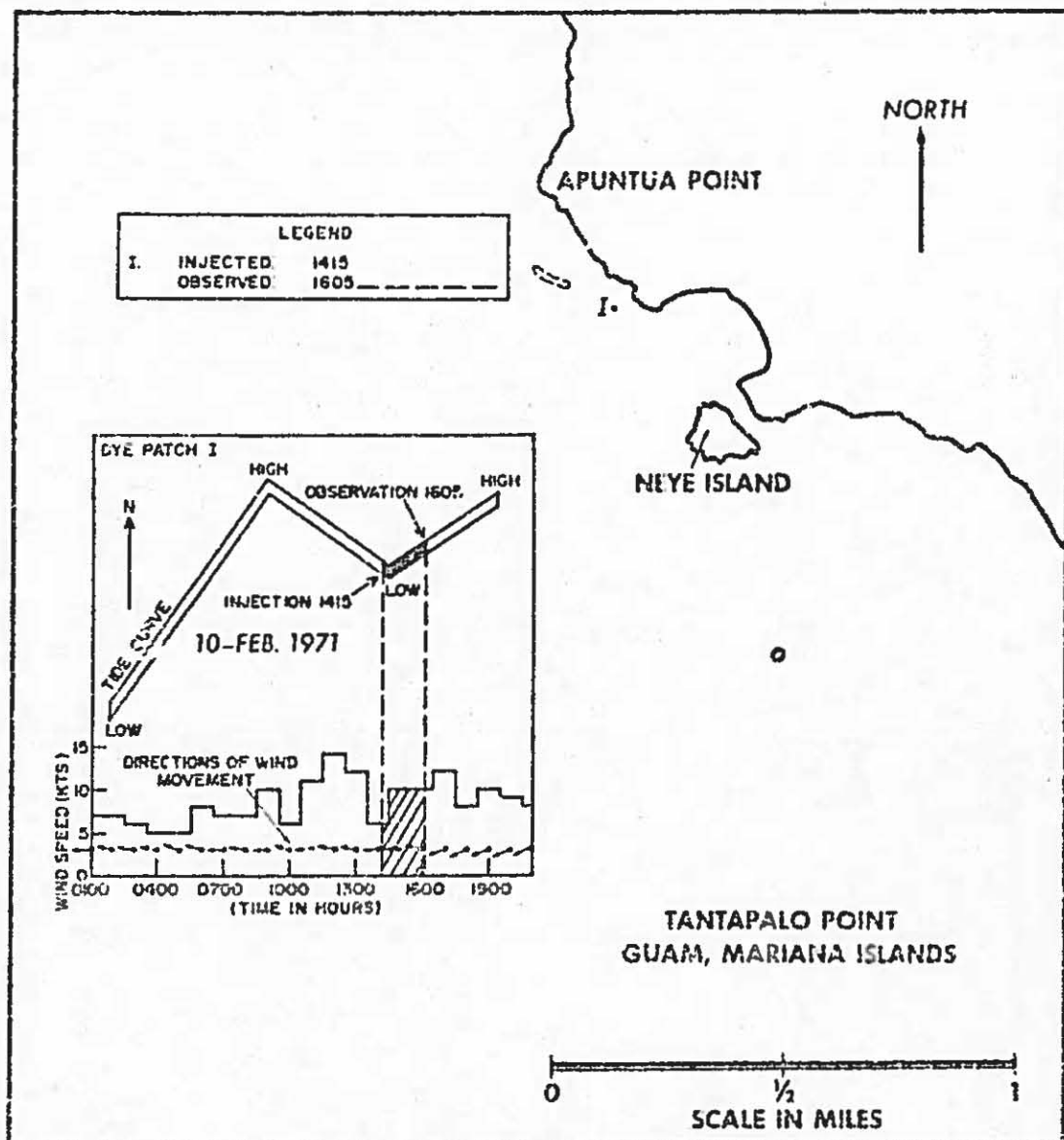
Figure 51. Dye movement at Tantapalo Point on 10 February 1971, P.M.
