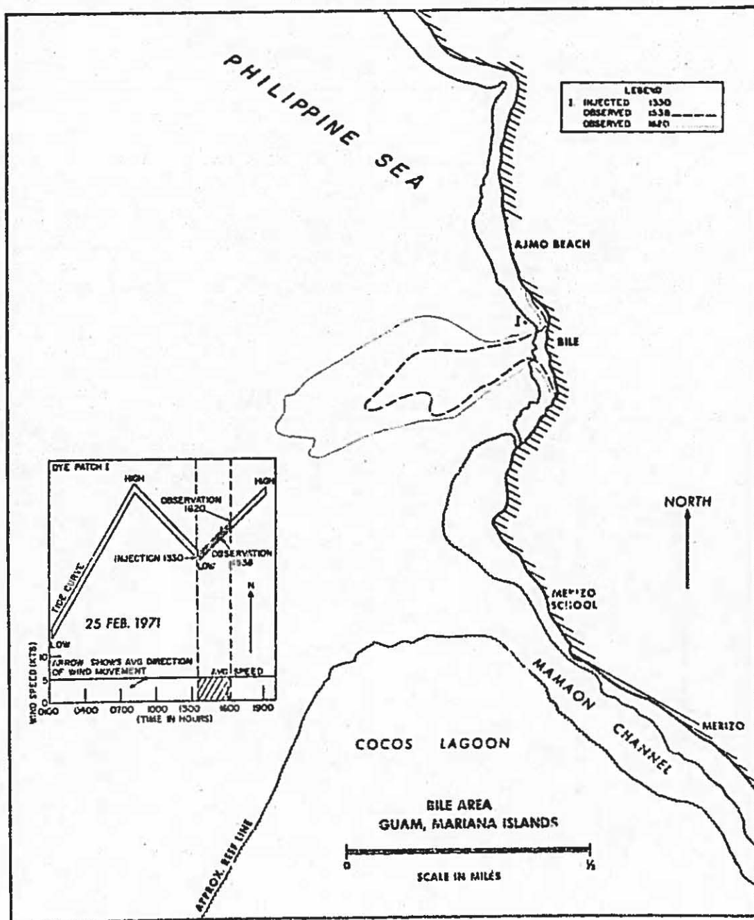
Figure 11. Dye movement at Bile Bay on 25 February 1971, P.M.
