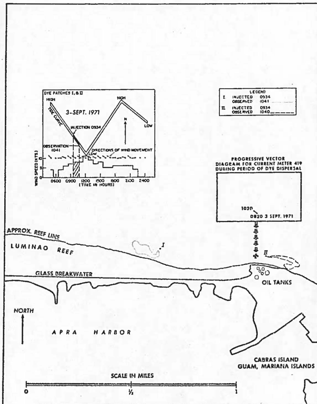
Figure 73. Dye movement at Cabras Island on 3 September 1971.
