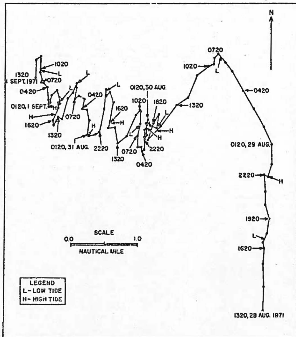
Figure 32. Progressive vector diagram of current from meter #405, 1320, 28 August to 1320, 1 September 1971.
