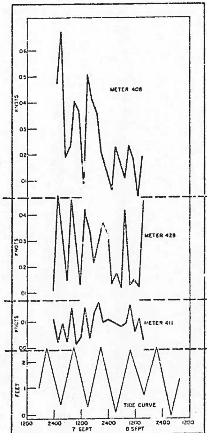
Figure 54. Current speeds versus tides from meters #408, #428, and #411.
