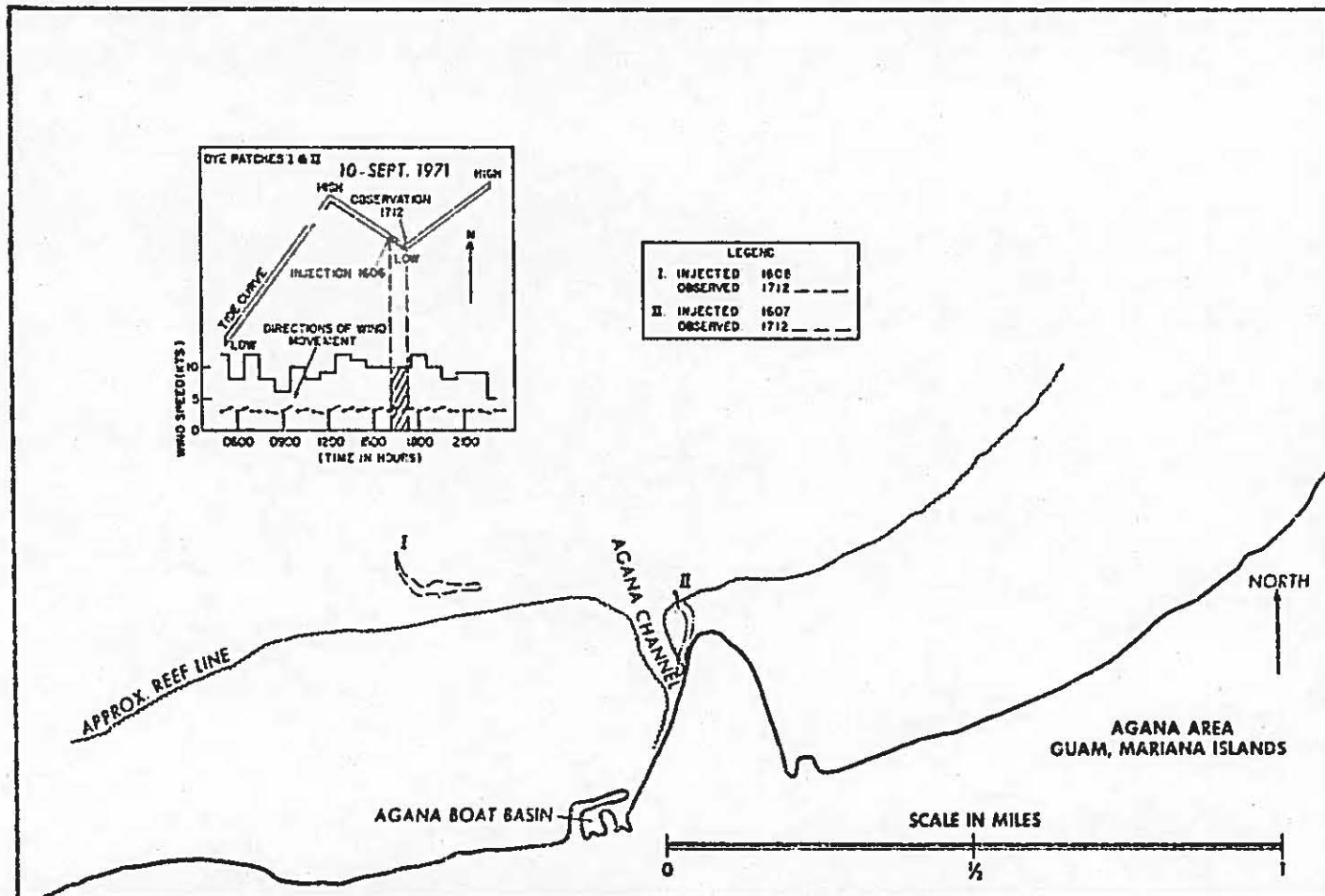
Figure 85. Dye movement at Agana Bay on 10 September 1971.
