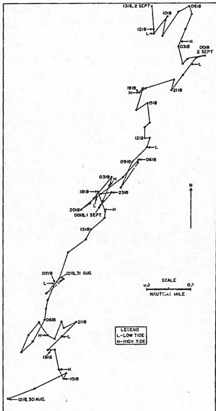
Figure 8. Progressive vector diagram of current from meter #412, 1218, 30 August to 1318, 2 September 1971.
