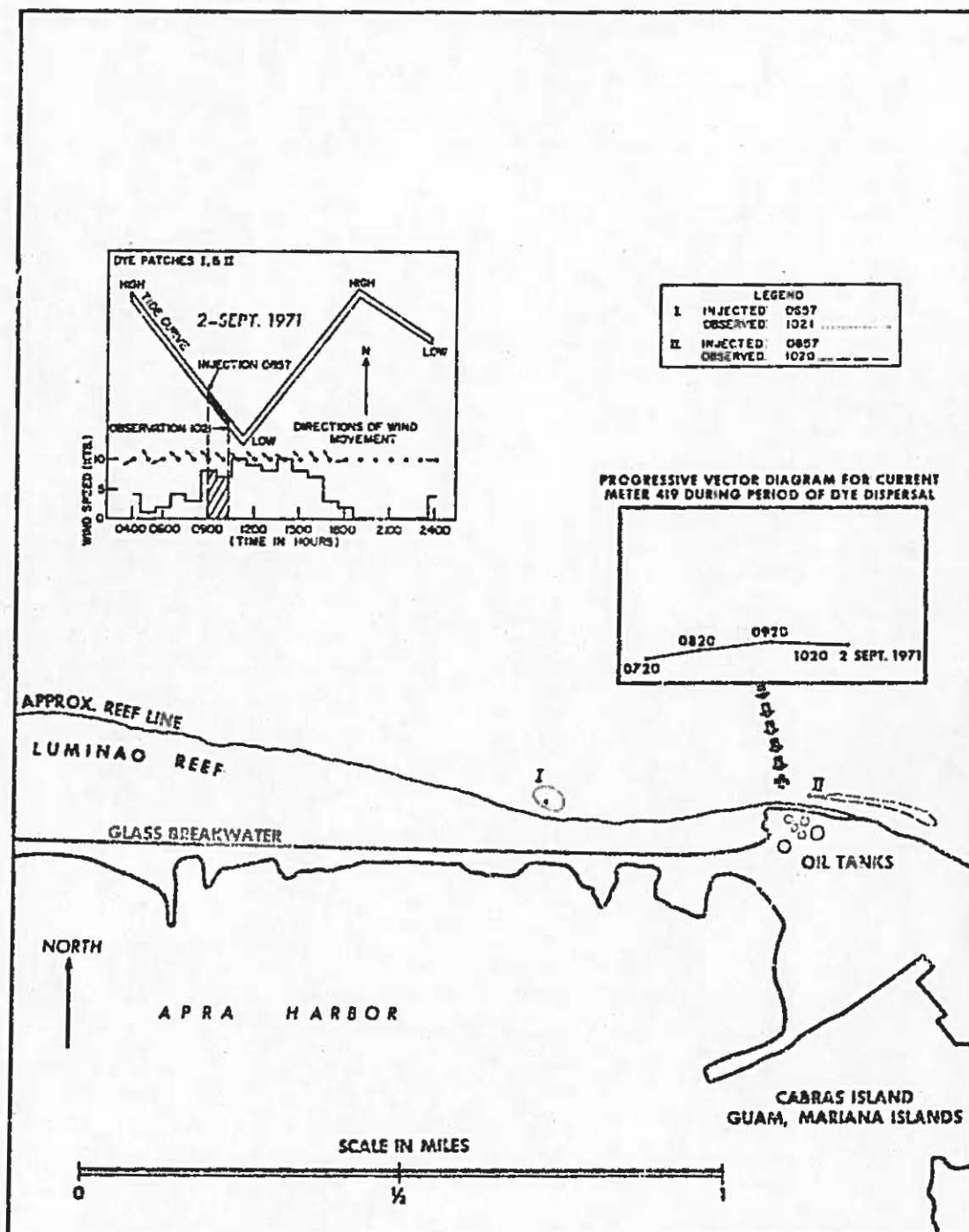
Figure 72. Dye movement at Cabras Island on 2 September 1971.
