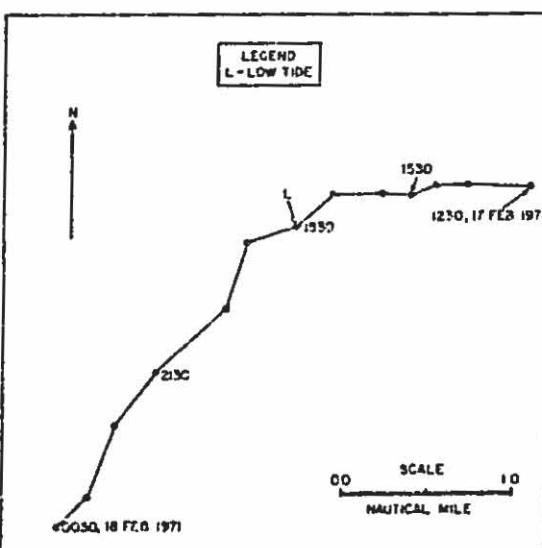
Figure 75. Progressive vector diagram of current from meter #346, 1230, 17 February to 0030, 18 February 1971.
