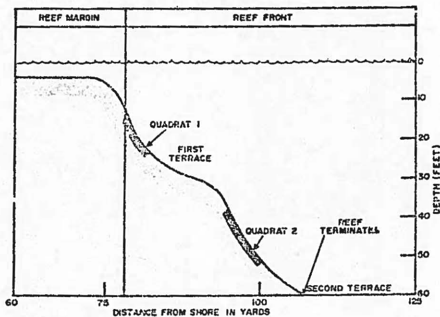
Figure 115. Area chart and reef profile for Bile Bay ecological study.
