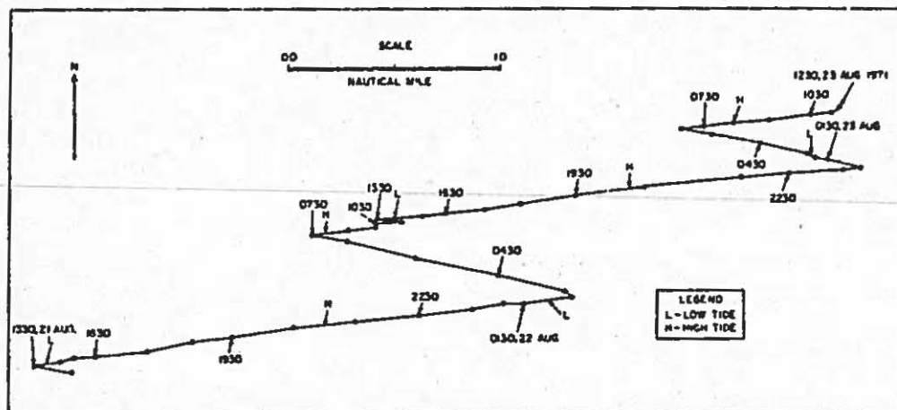
Figure 21. Progressive vector diagram of current from meter #407, 21 - 23 August 1971.
