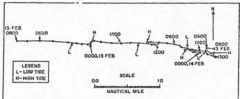
Figure 48. Progressive vector diagram of current from meter #323, 0800, 13 February to 0800, 15 February 1971.
