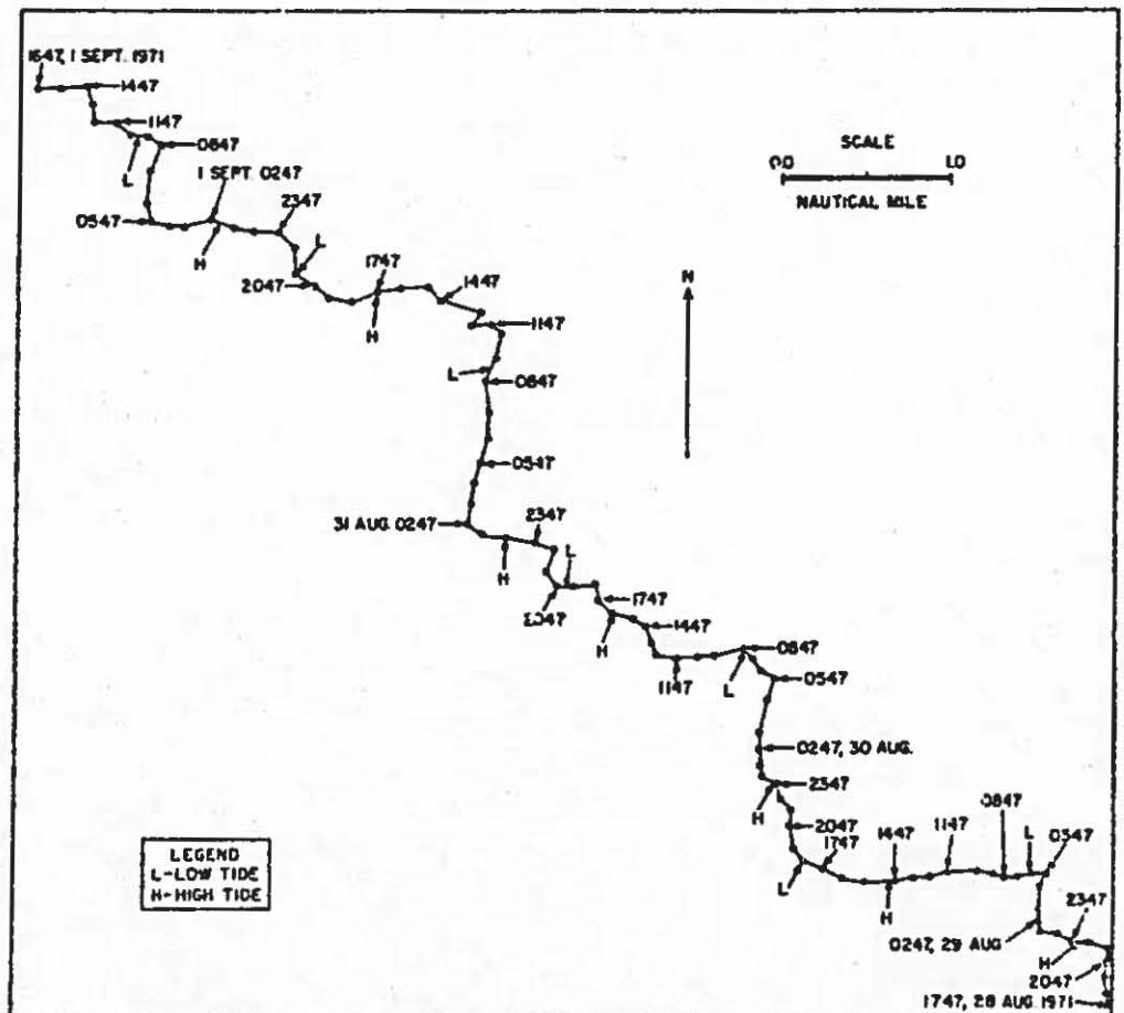
Figure 31. Progressive vector diagram of current from meter #426, 1747, 28 August to 1647, 1 September 1971.
