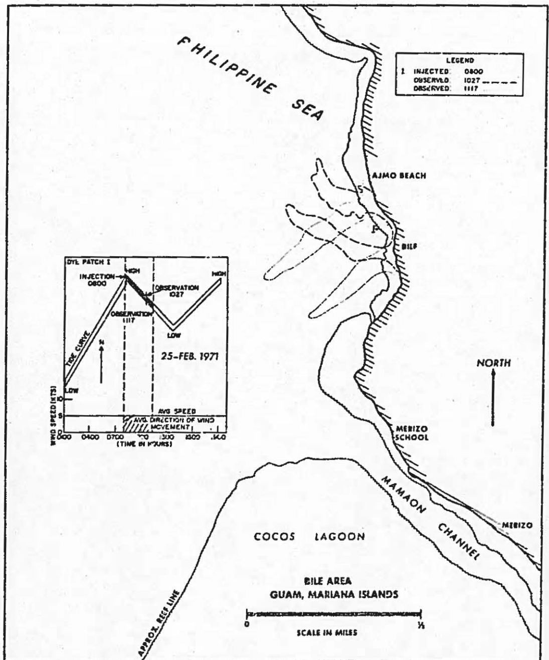
Figure 10. Dye movement at Bile Bay on 25 February 1971, 1 A.
