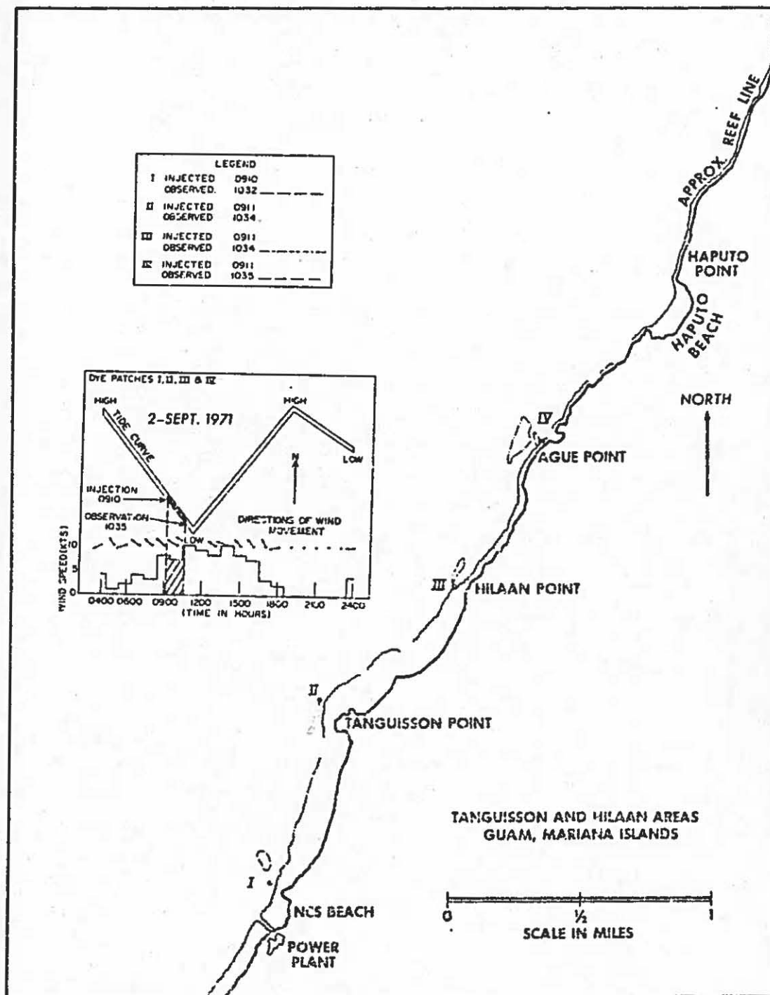
Figure 100. Dye movement at Tanguisson Point on 2 September 1971, A.M.
