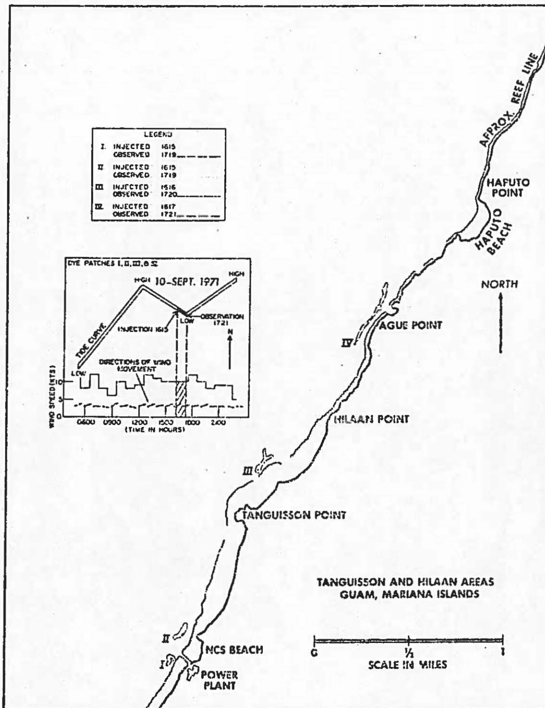
Figure 104. Dye movement at Tanguisson Point on 10 September 1971.
