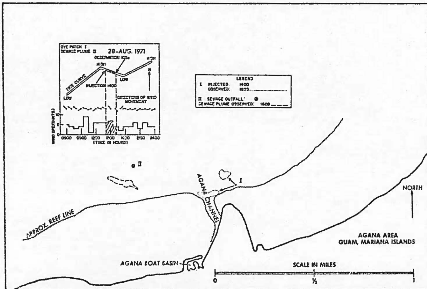
Figure 78. Dye movement at Agana Bay on 28 August 1971.
