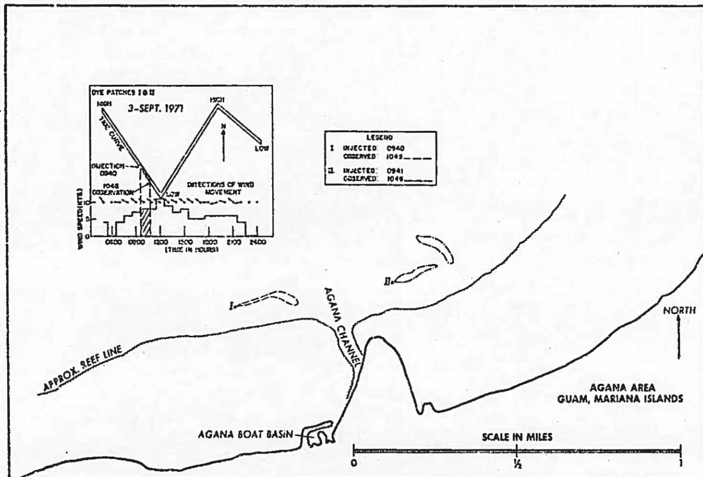
Figure 84. Dye movement at Agana Bay on 3 September 1971.
