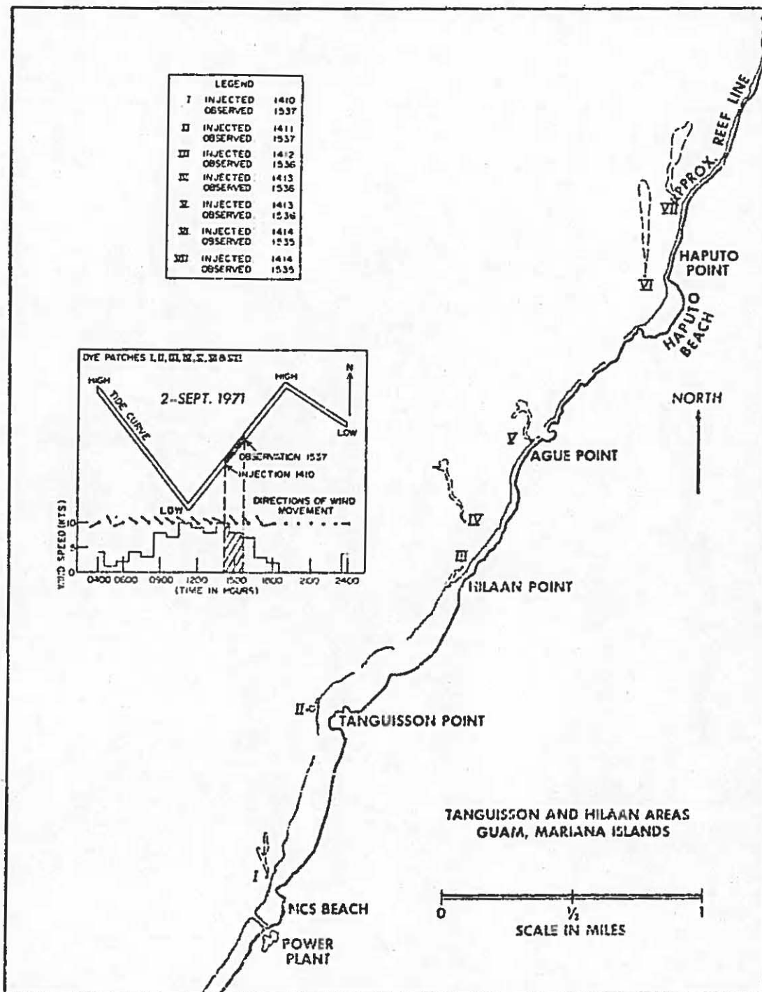
Figure 101. Dye movement at Tanguisson Point on 2 September 1971, P.M.
