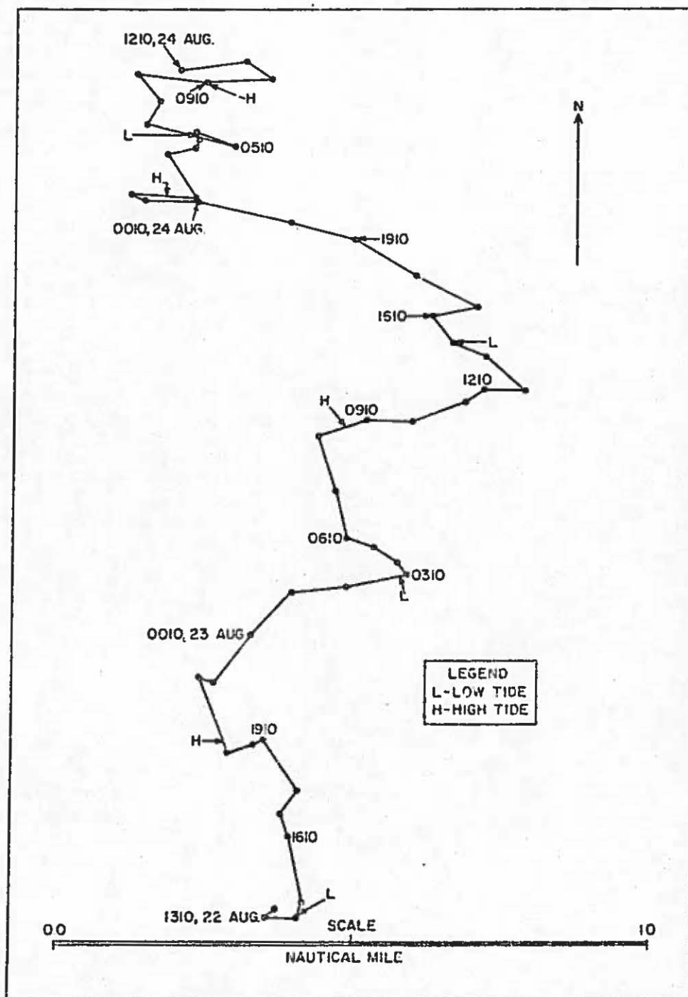
Figure 77. Progressive vector diagram of current from meter #406, 1210, 22 August to 1210, 24 August 1971.
