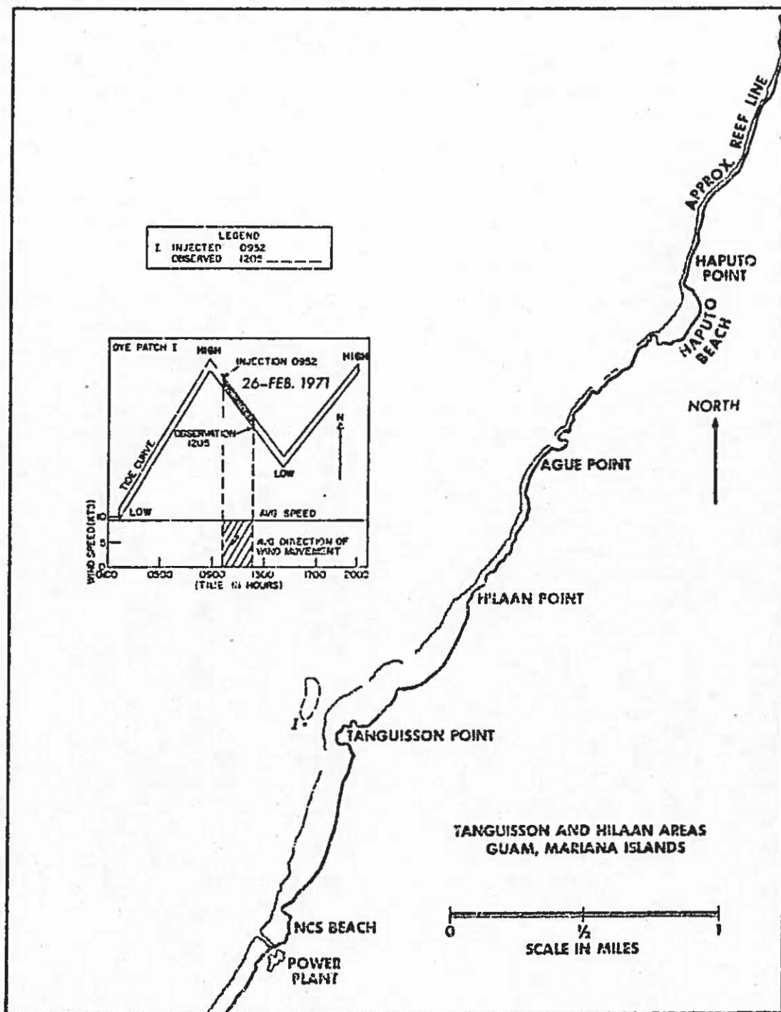
Figure 94. Dye movement at Tanguisson Point on 26 February 1971, A.M.
