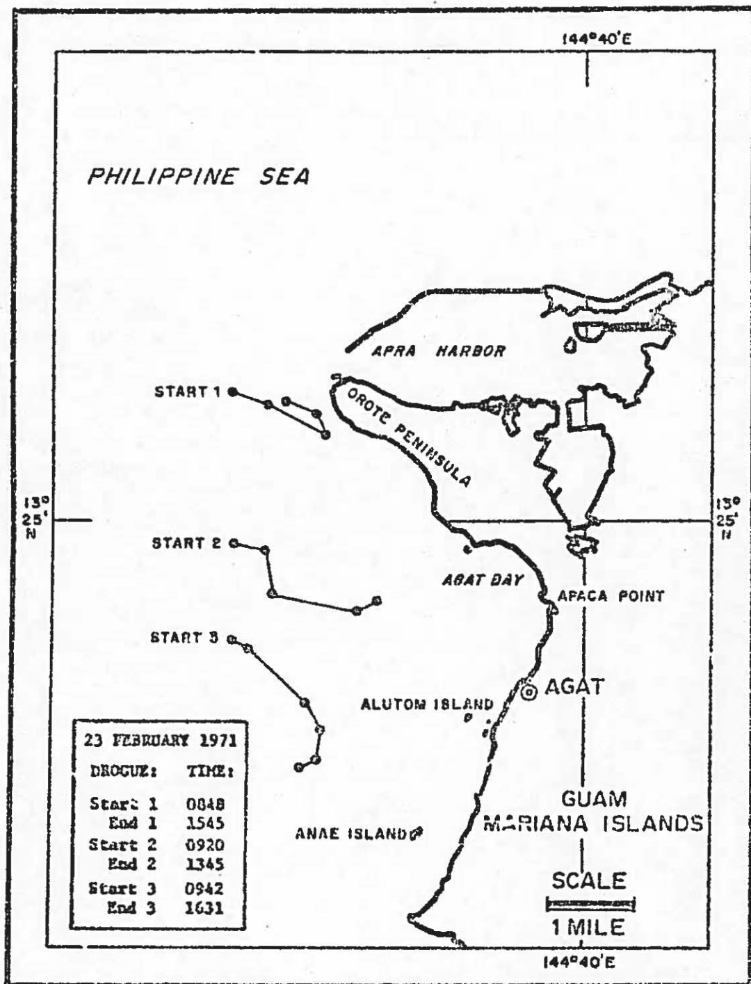
Figure 56. Drogue observations in Agat Section, 23 February 1971.
