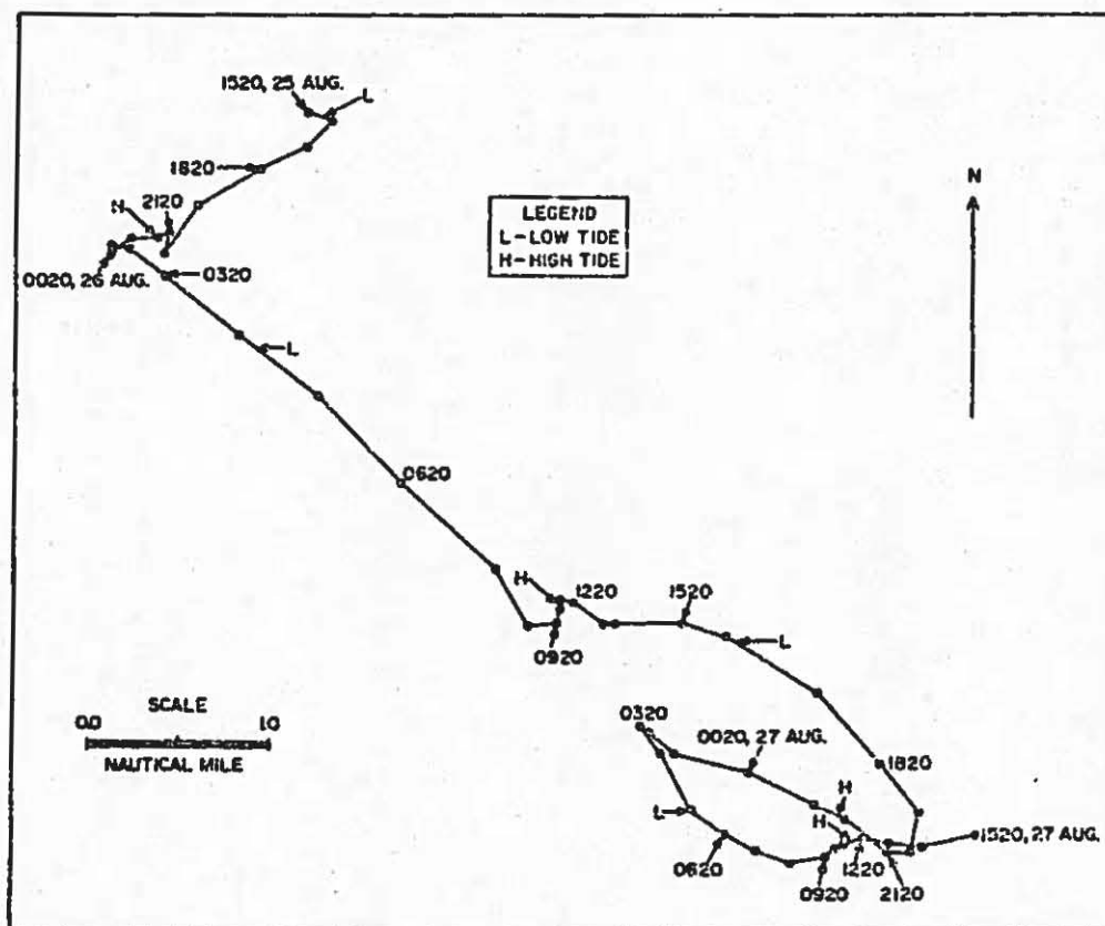
Figure 110. Progressive vector diagram of current from meter #404, 1520, 25 August to 1520, 27 August 1971.
