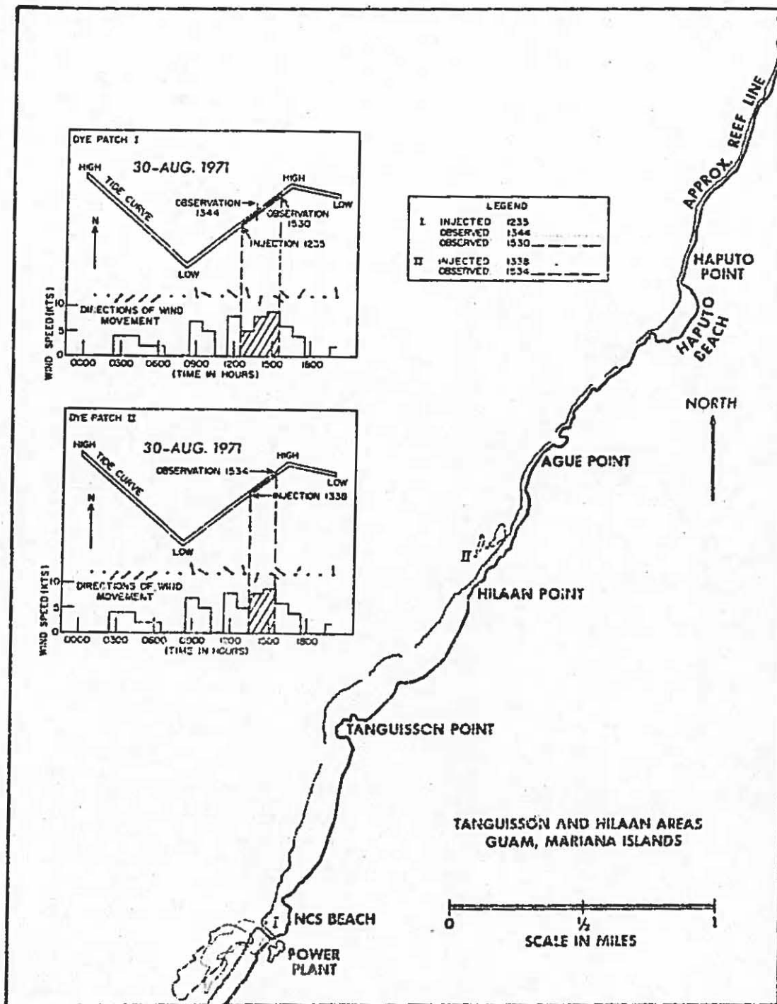
Figure 97. Dye movement at Tanguisson Point on 30 August 1971.
