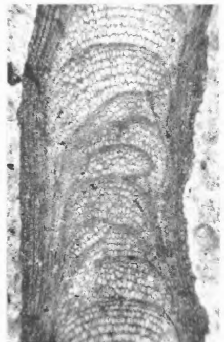
MIOCENE DERMATOLITHON , LITHOPORELLA , MELOBESIA , ARCHAEOLITHOTHAMNIUM , AND AETHESOLITHON ; AND PLIOCENE AND PLEISTOCENE DERMATOLITHON
