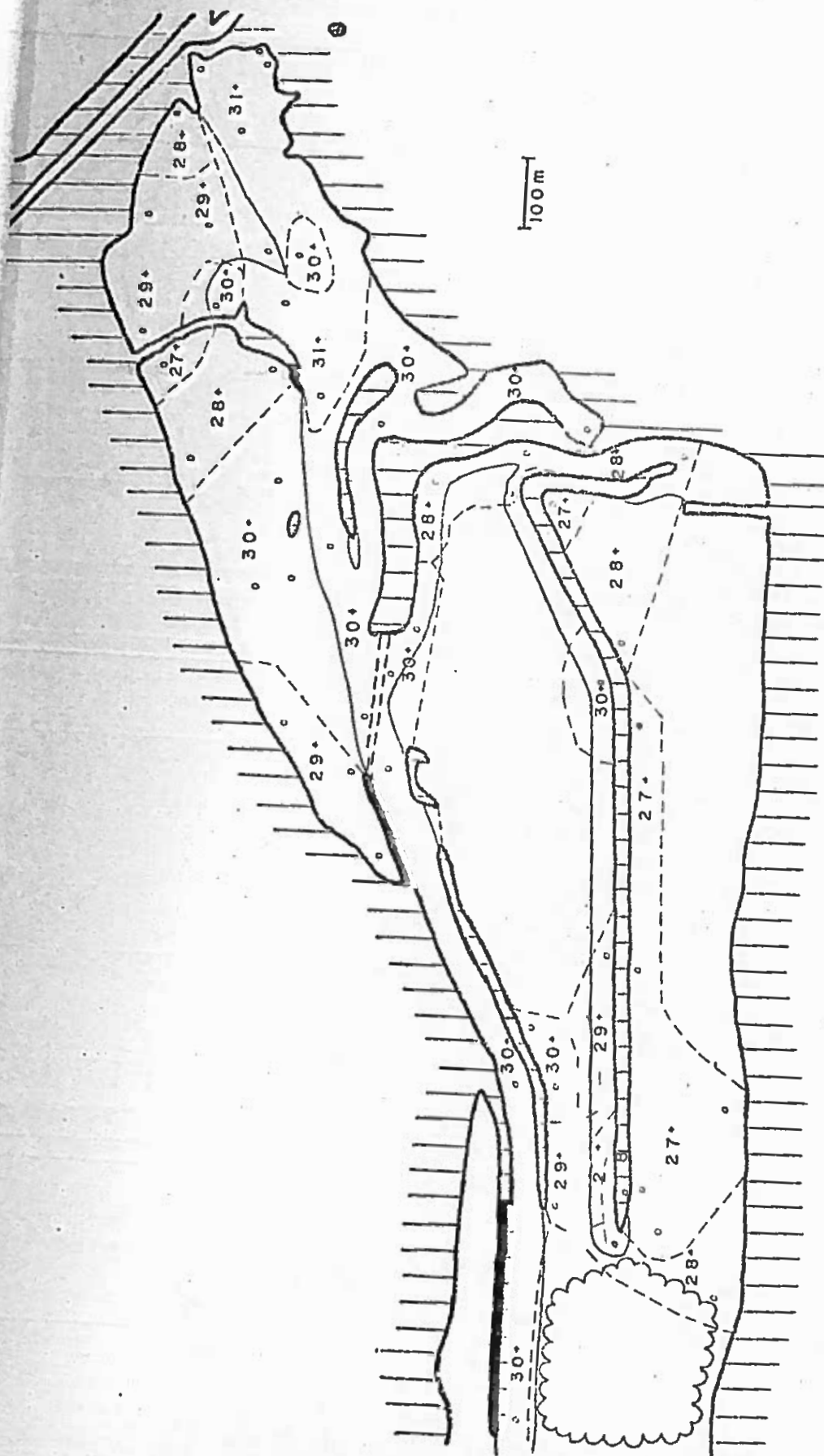
Figure 7. Isotherm plot for 11 August 1972, 1000-1200 hours. A high tide of 1.9 ft occurred at 0754 hours, and a low tide of -0.3 ft occurred at 1506 hours. The sky was mostly overcast.
