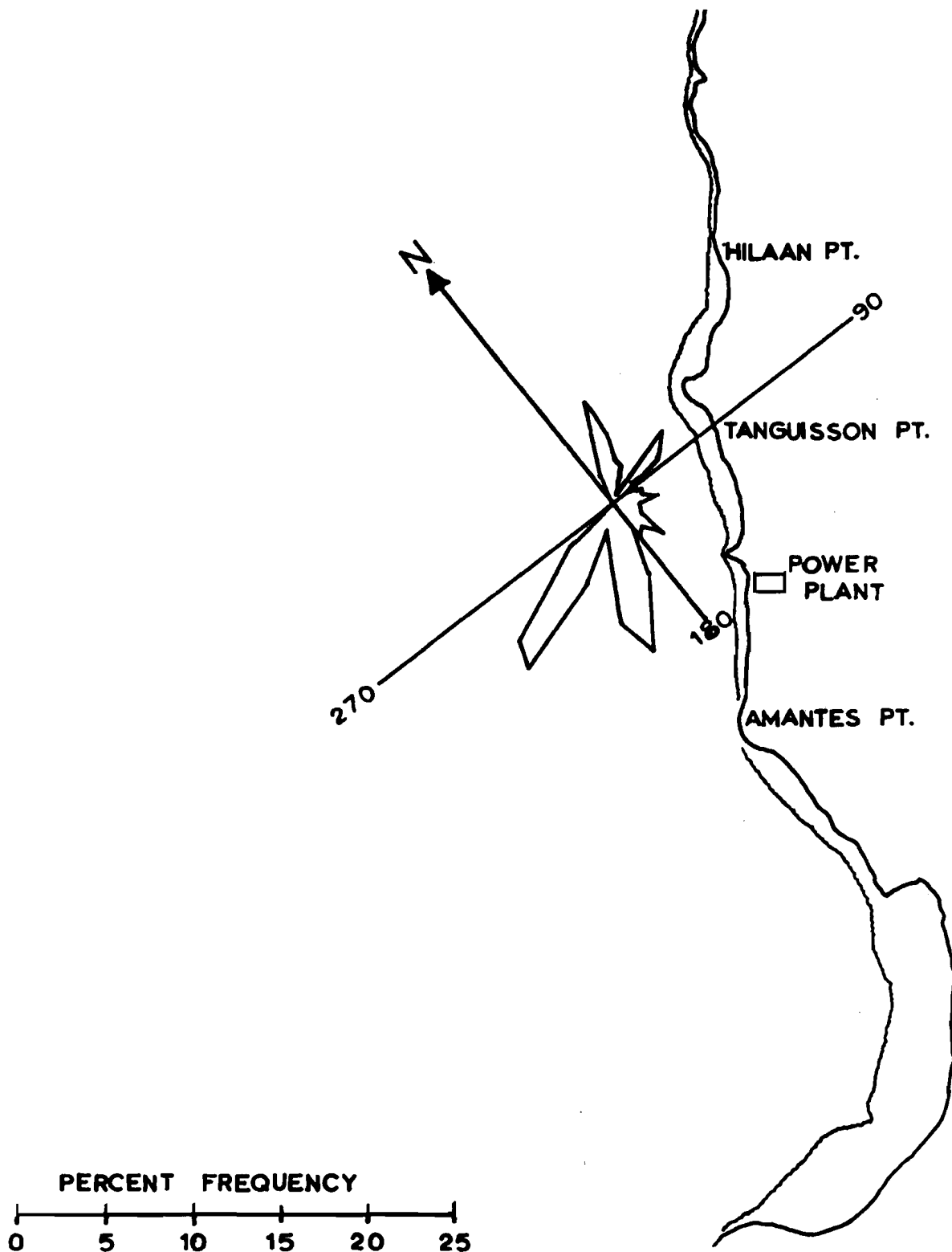
Figure 7 Mean frequency diagram for current direction at 5 m
