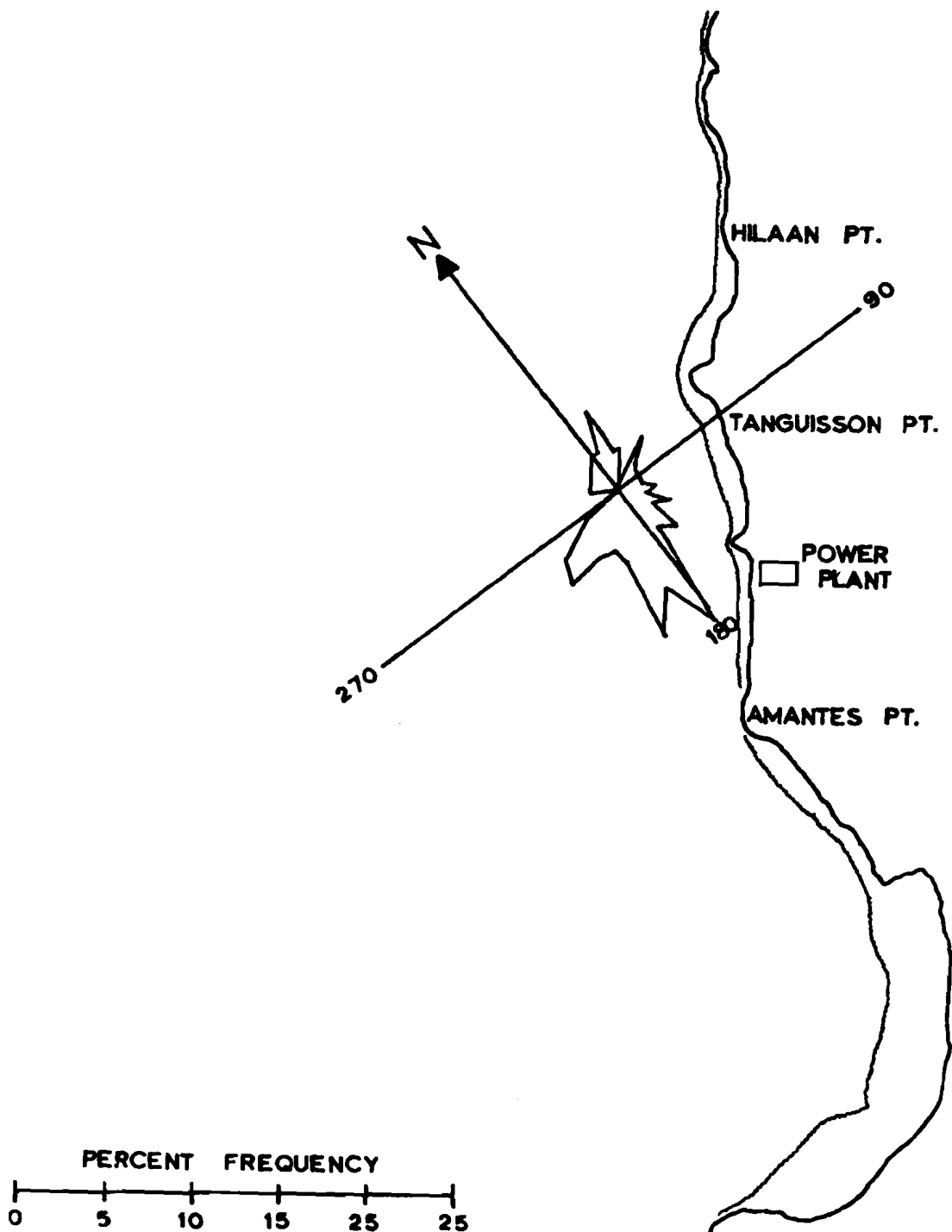
Figure 11 Mean frequency diagram for current direction, all stations combined
