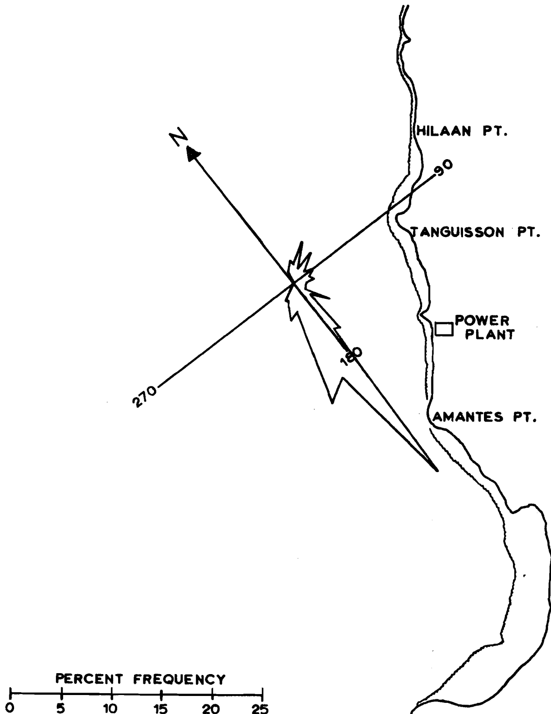
Figure 8 Mean frequency diagram for current direction at 10 to 14 m
