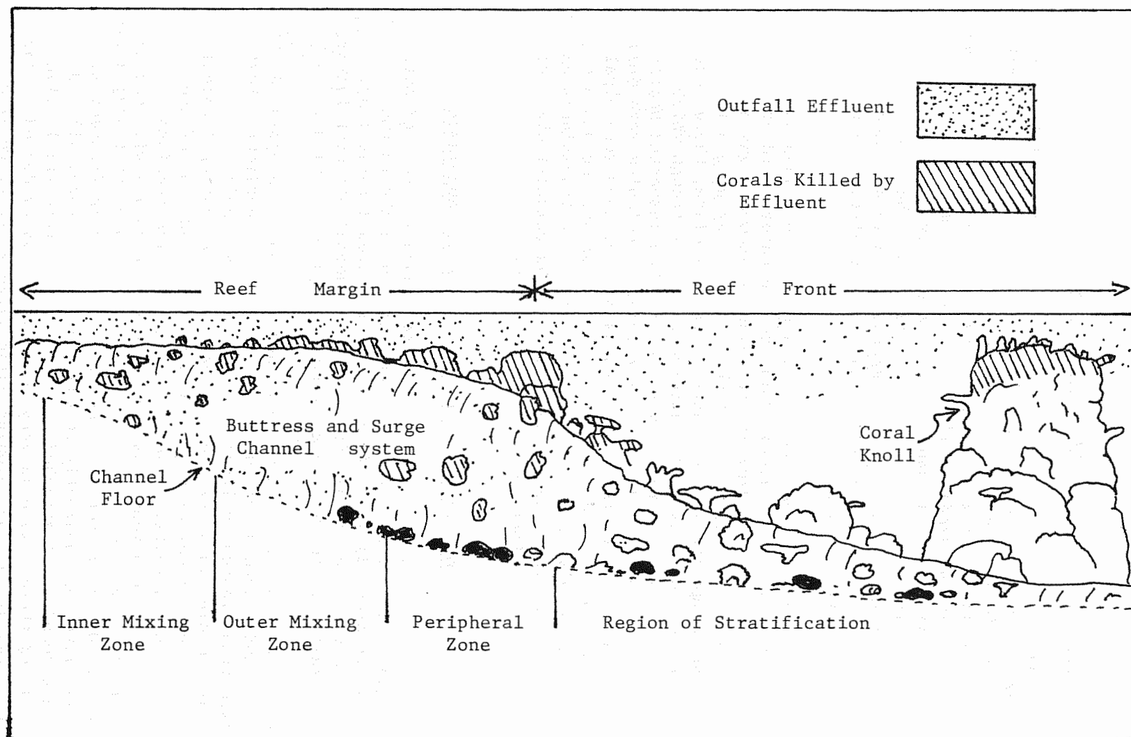
Fig. 4. Vertical profile through the reef margin and reef front zones.
