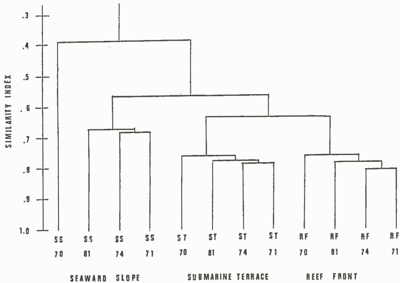
Figure 2. Dendrogram constructed from similarity indices (Table 1).
