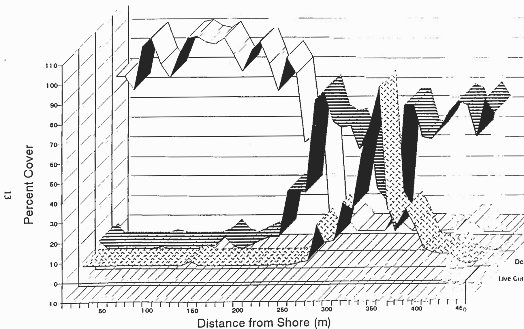
Figure II-2. Percent cover of sand (white ribbon), dead coral and reef pavement (hatched ribbon), and live coral (stitched ribbon) quantified within 10 meter intervals (0.25 meters wide) along Transect 2 in Tumon Bay during December 1991.
