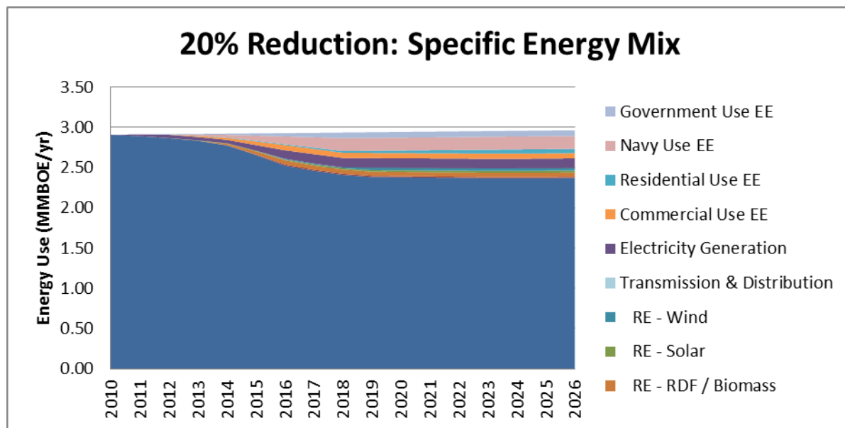
Figure 9. 20% reduction: specific energy mix
