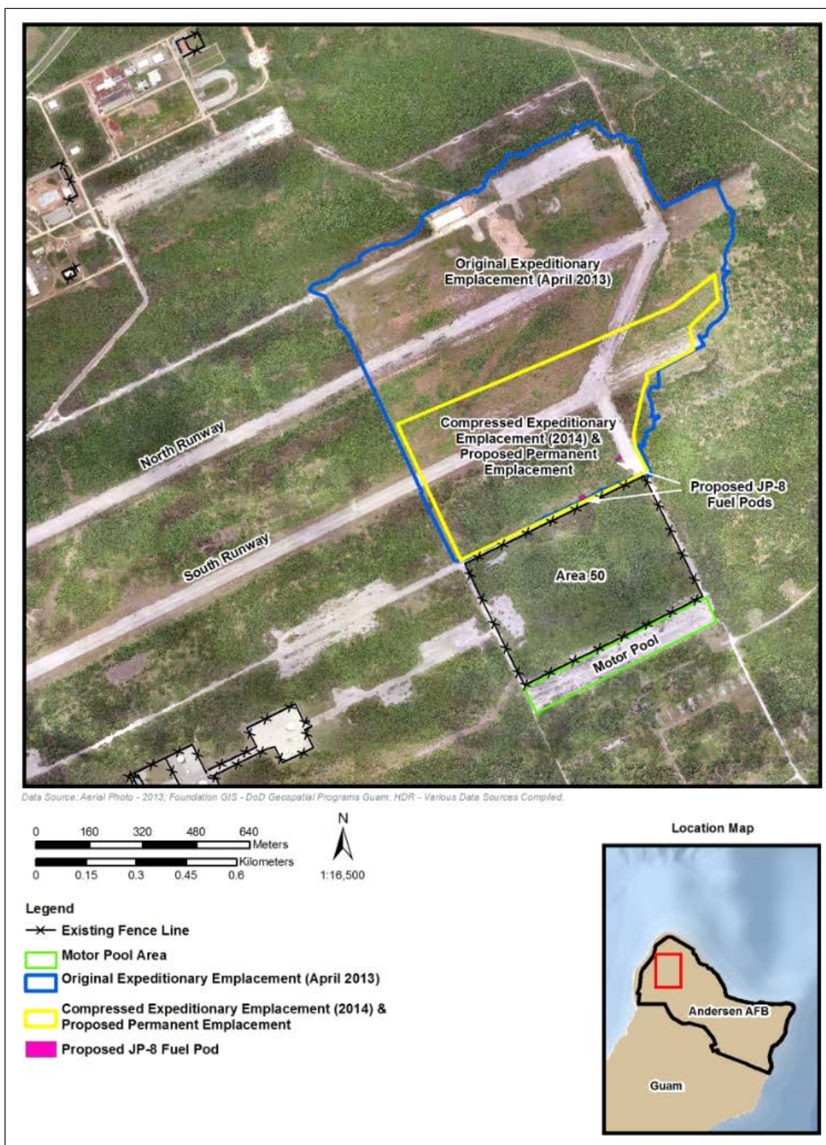
Figure 2-2. Original and Compressed Expeditionary Emplacement of the THAAD System
