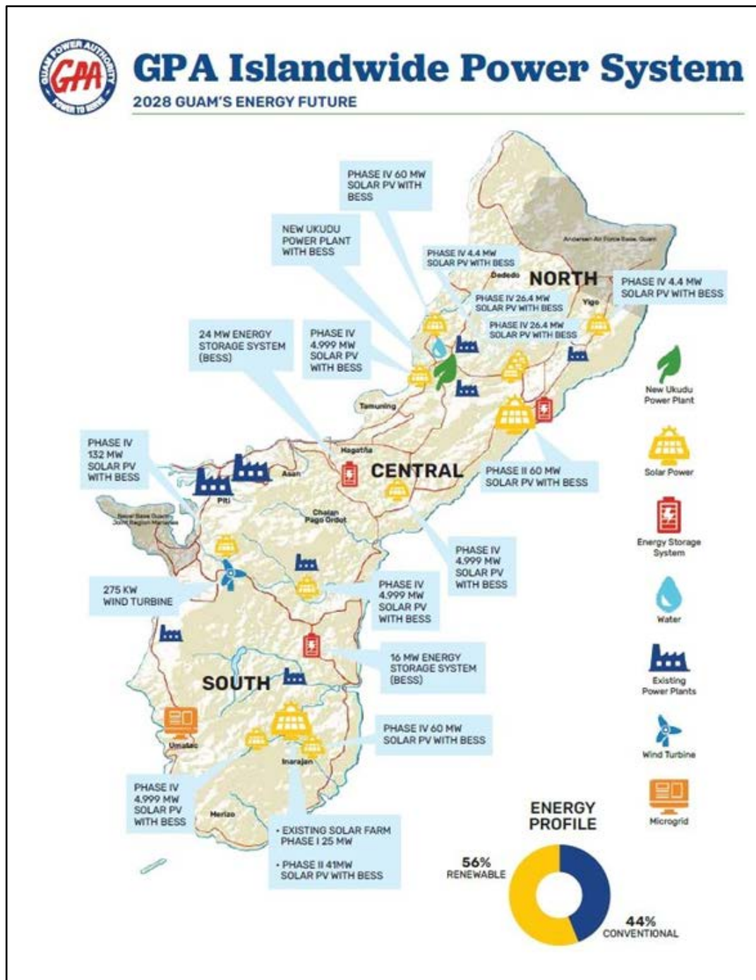
Figure 3-21. GPA Islandwide Power System: 2028 Guam's Energy Future.
