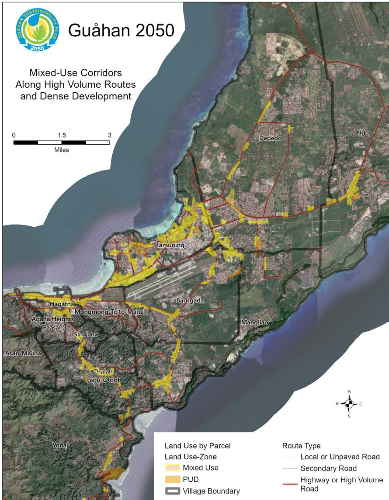
Figure 3-29. Mixed-use corridors (yellow) in North and Central Guam.
