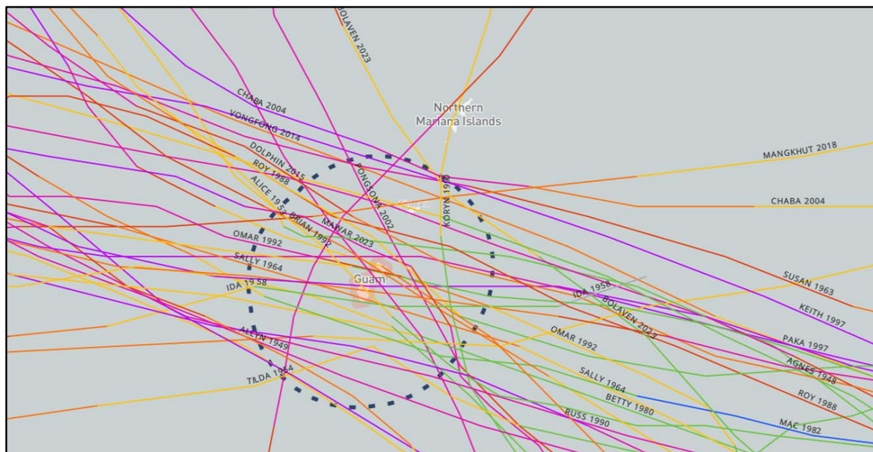
Figure 3-33. Typhoon tracks near Guam, 1948-present (NOAA, 2025).
