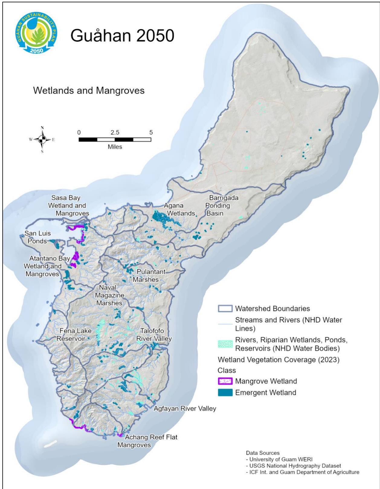
Figure 5-8. Map of Guam Wetlands by Type.
