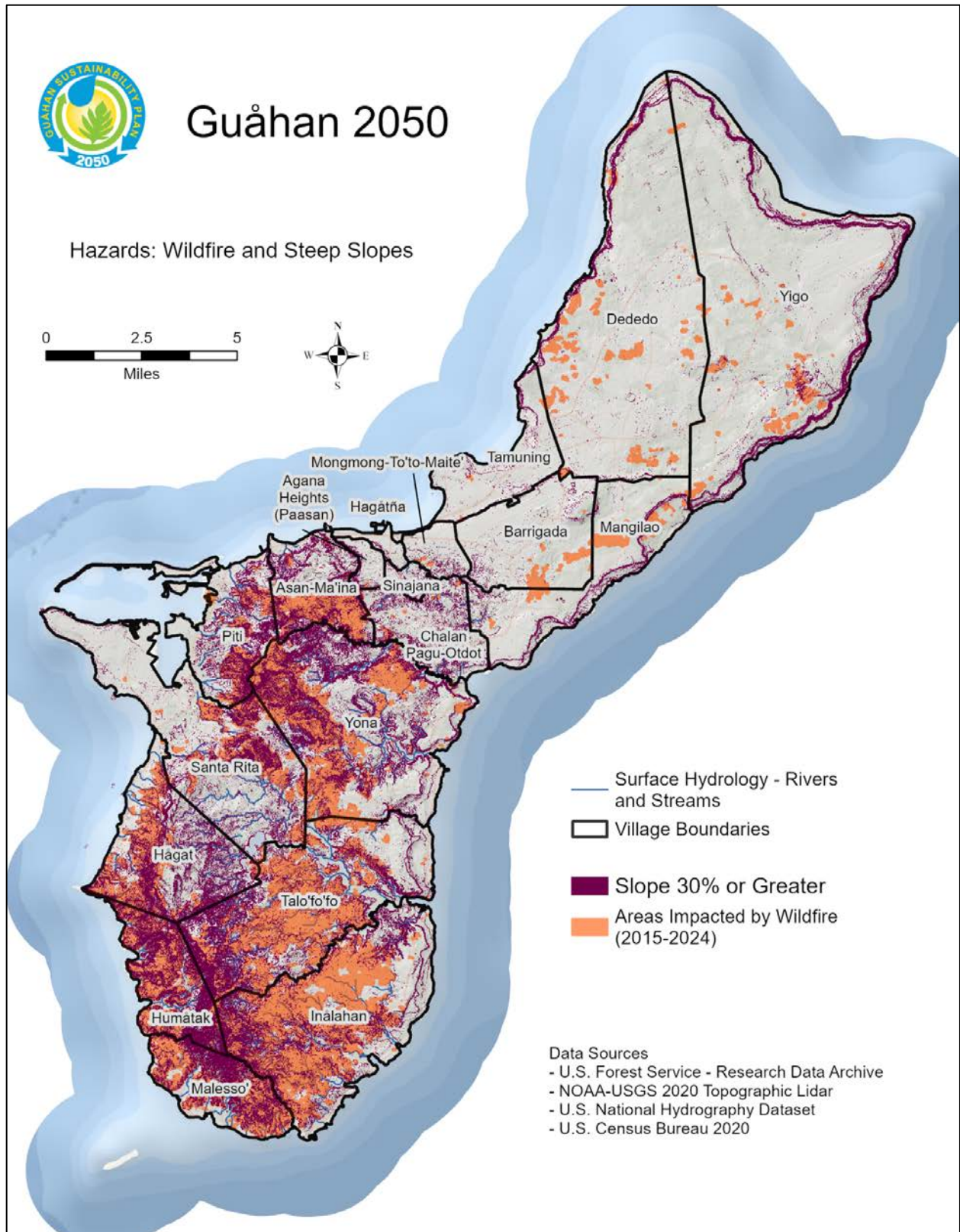
Figure 3-39. Guam Wildfire Hazards and Steep Terrain
