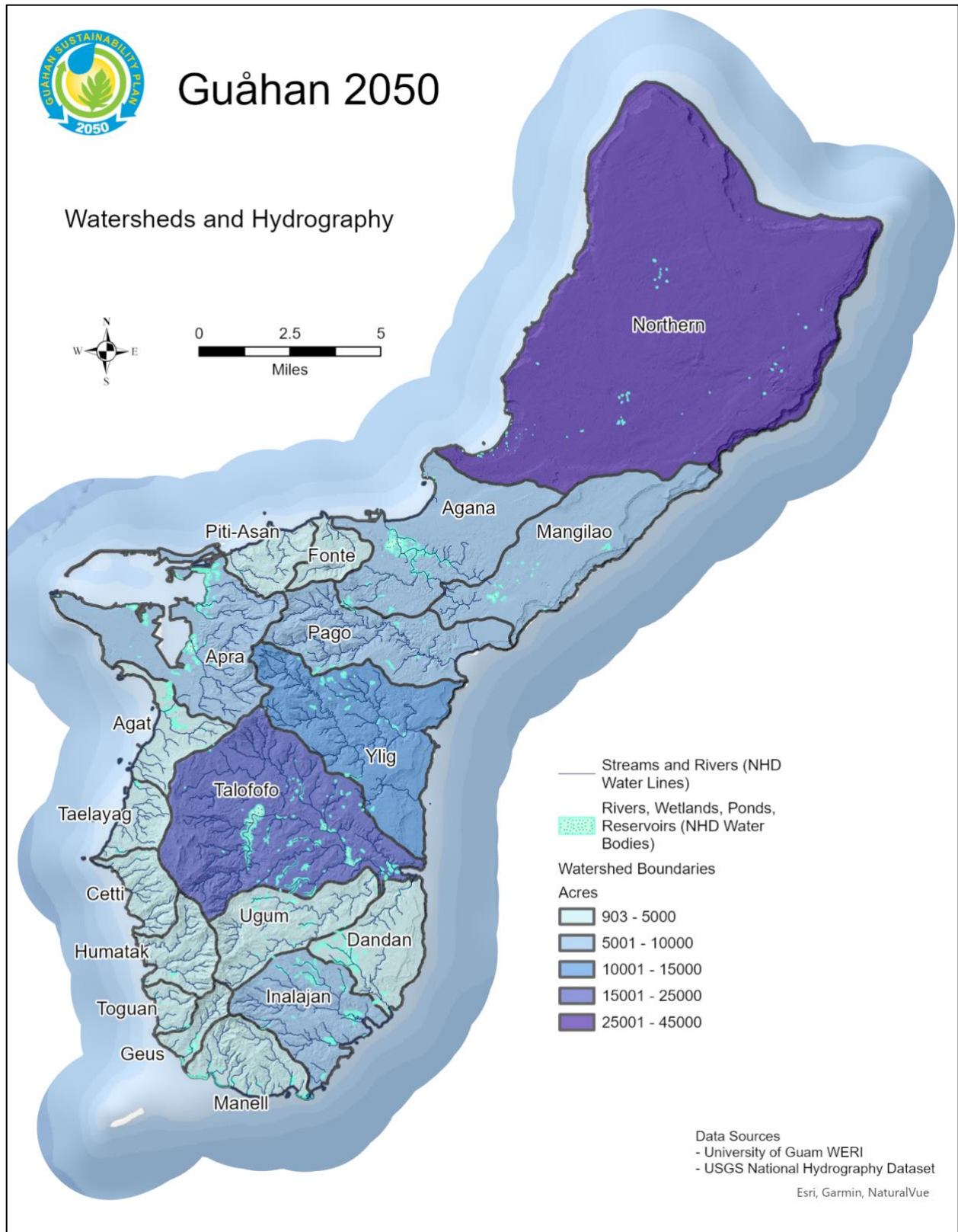
Figure 5-3. Guam Watersheds and Hydrography.
