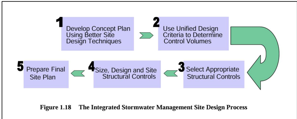
Figure 5-7. Stormwater Management for Proposed Development Sites (from CNMI and Guam Stormwater Management Manual).
