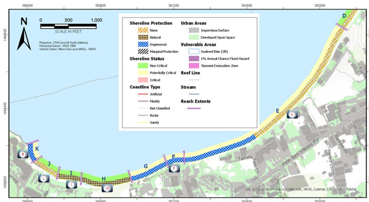
Figure 3-37. Guam Shoreline Atlas Shoreline Status, Tamuning.
