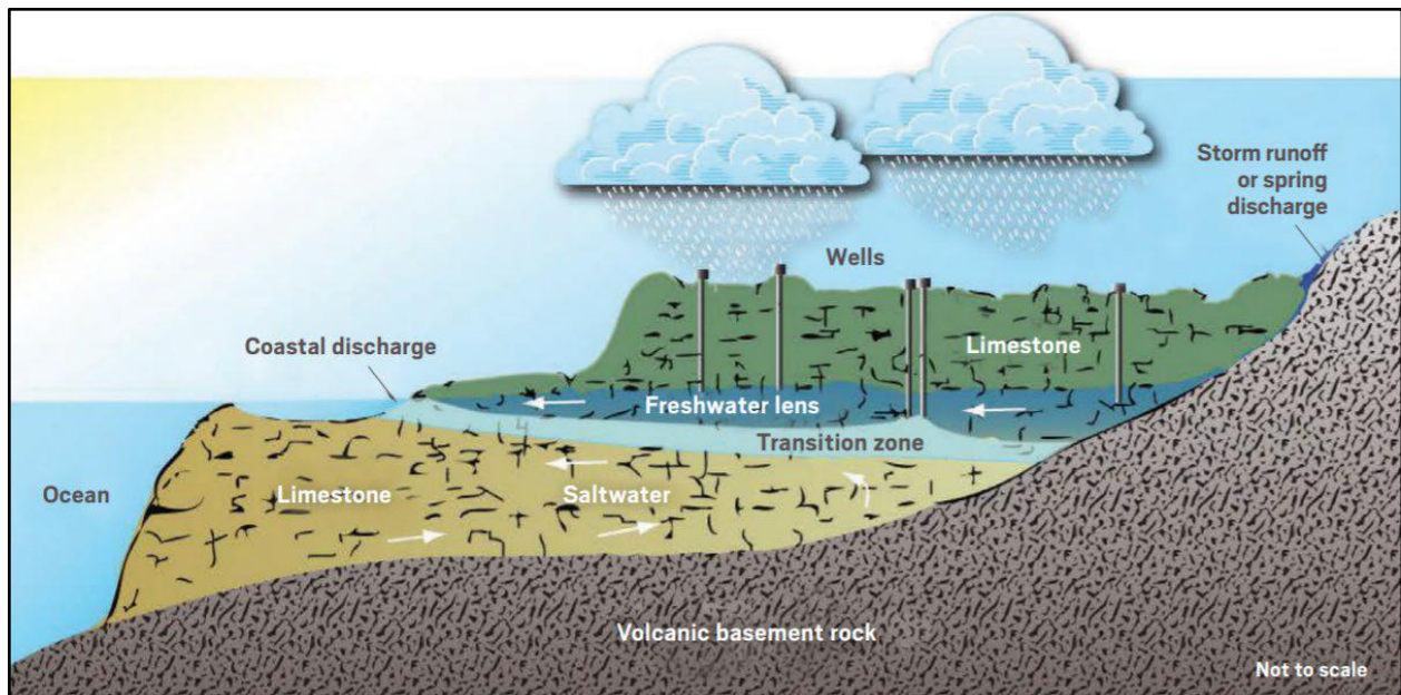
Figure 5-4. Northern Guam Lens Aquifer.
