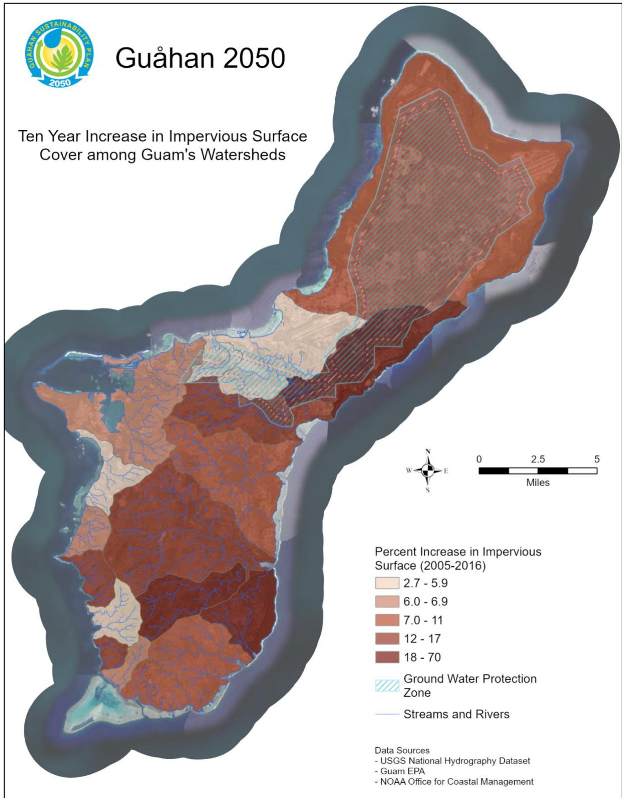
Figure 5-11. A Decade of Increases in Impervious Surface Cover in Guam's Watersheds from 2005-2016.
