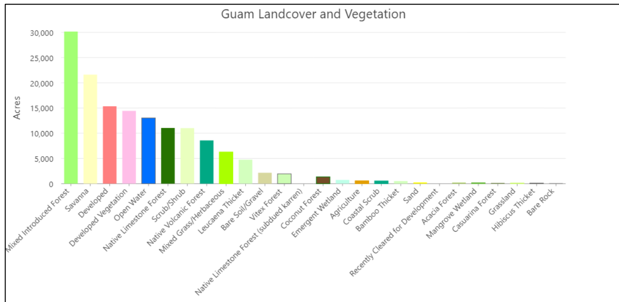
Figure 5-10. Guam Land Cover Composition by Acreage, as mapped by ICF International Inc. and Guam Department of Agriculture (2023).
