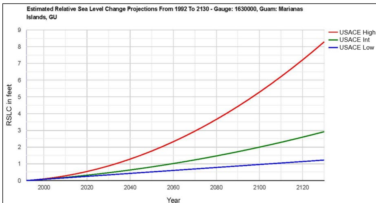
Figure 4-2. Projected RSLC for Guam
