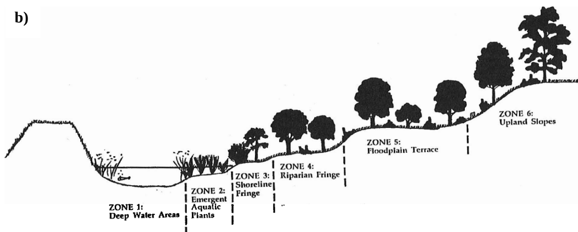
Figure 5.1 Planting Zones for Stormwater Ponds and Wetlands as they appear in a) plan view and b) cross-section (Schueler, 1992).
