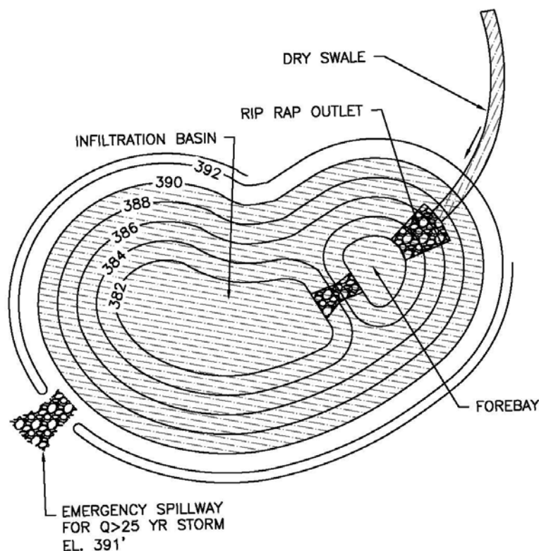
Figure 4.6 Plan View of Infiltration Basin
