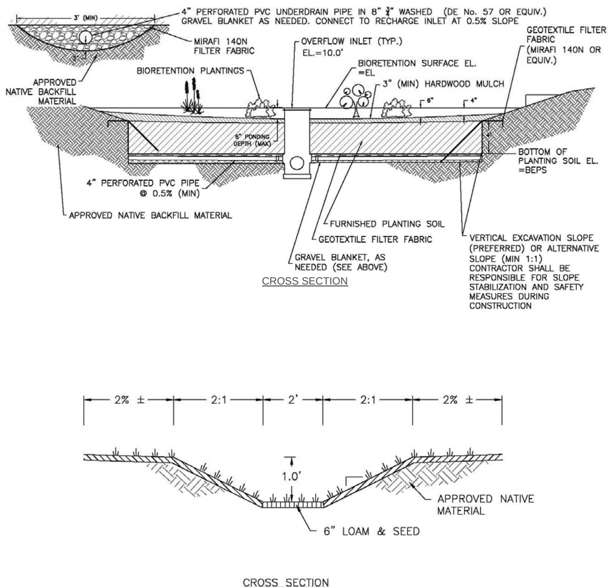
Figure 4.10 Typical Sections of a Bioretention Facility and a Grass Swale
